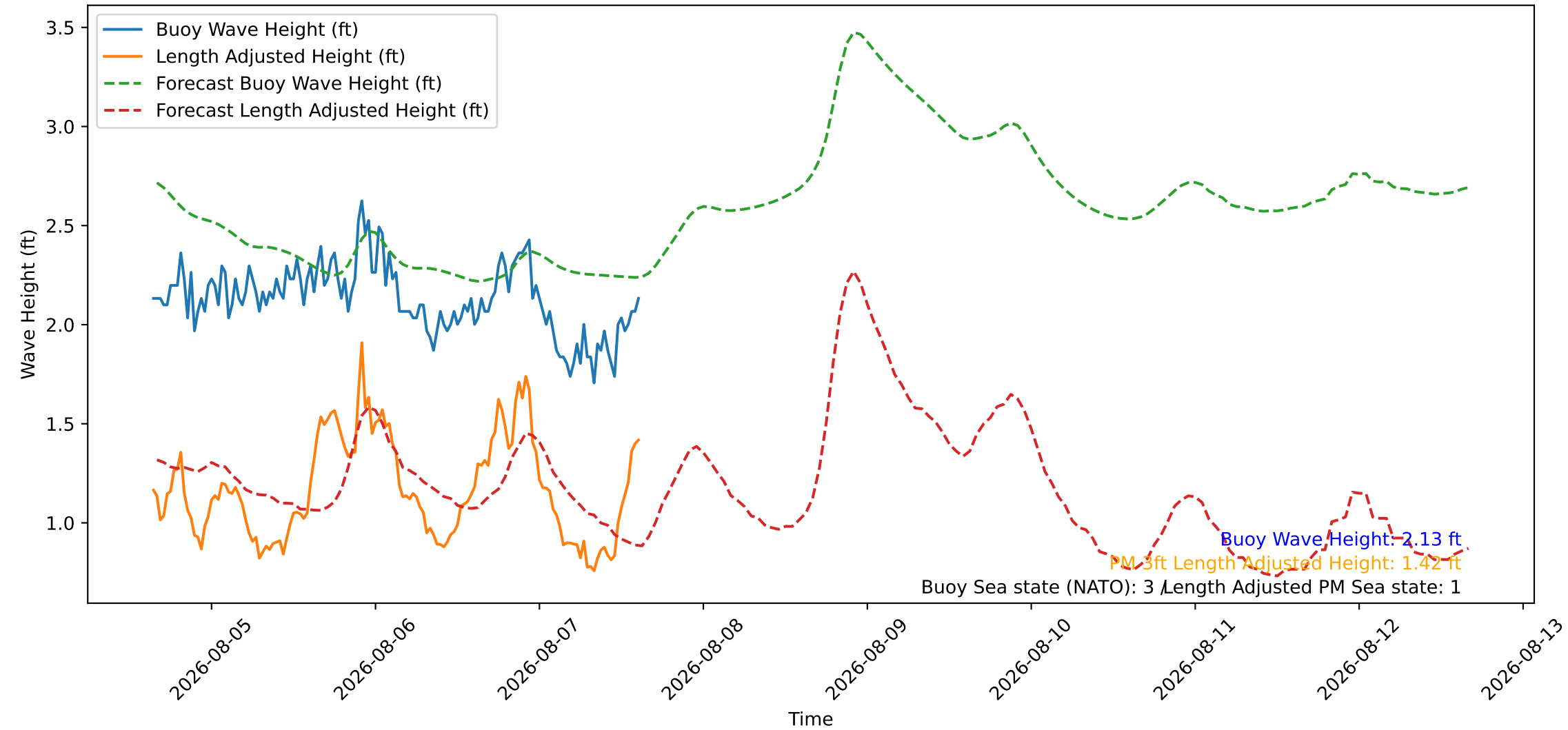
Wave Heights over Time for Green Beach at 2026-08-07 15:31:08
