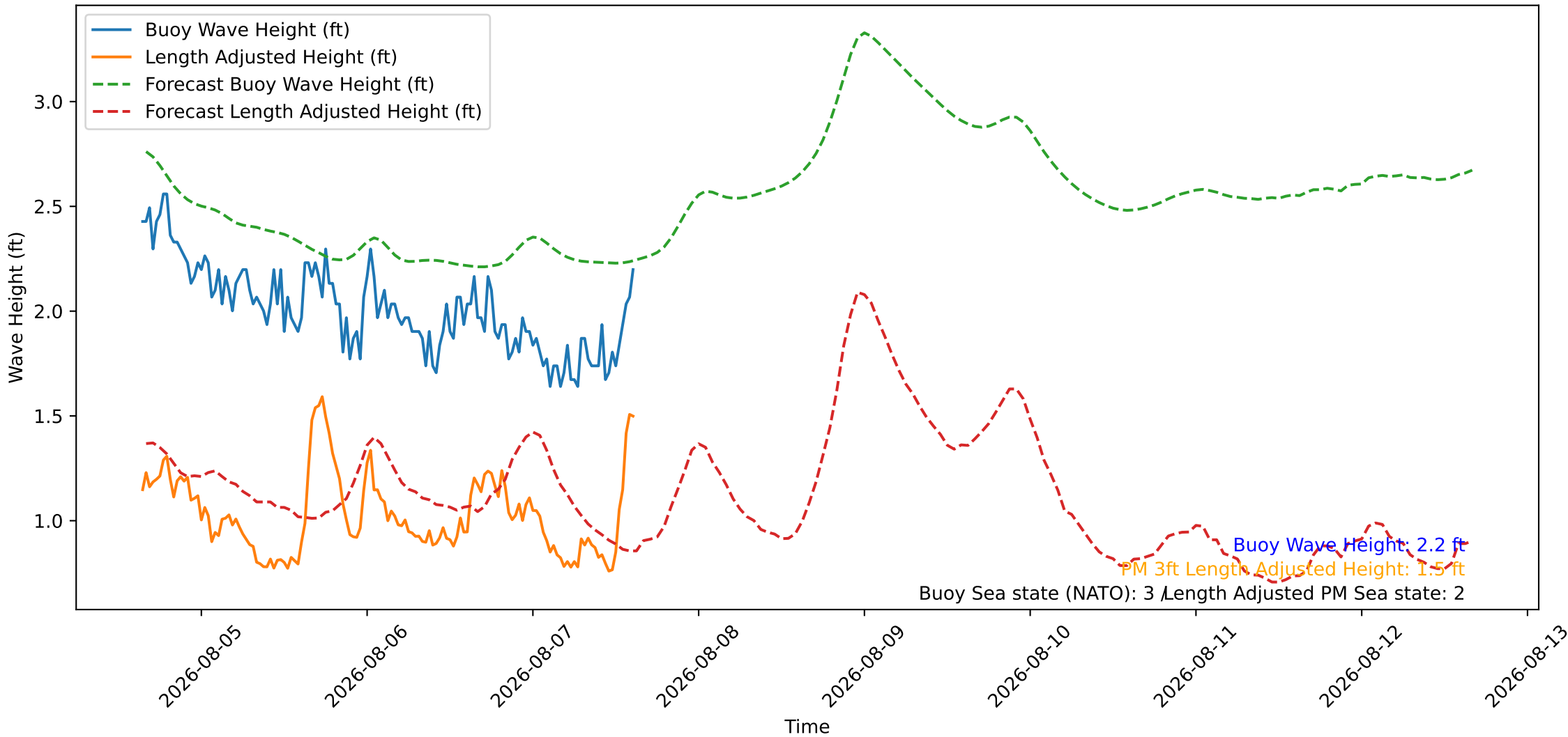
Wave Heights over Time for Oceanside Harbor at 2026-08-07 15:30:26
