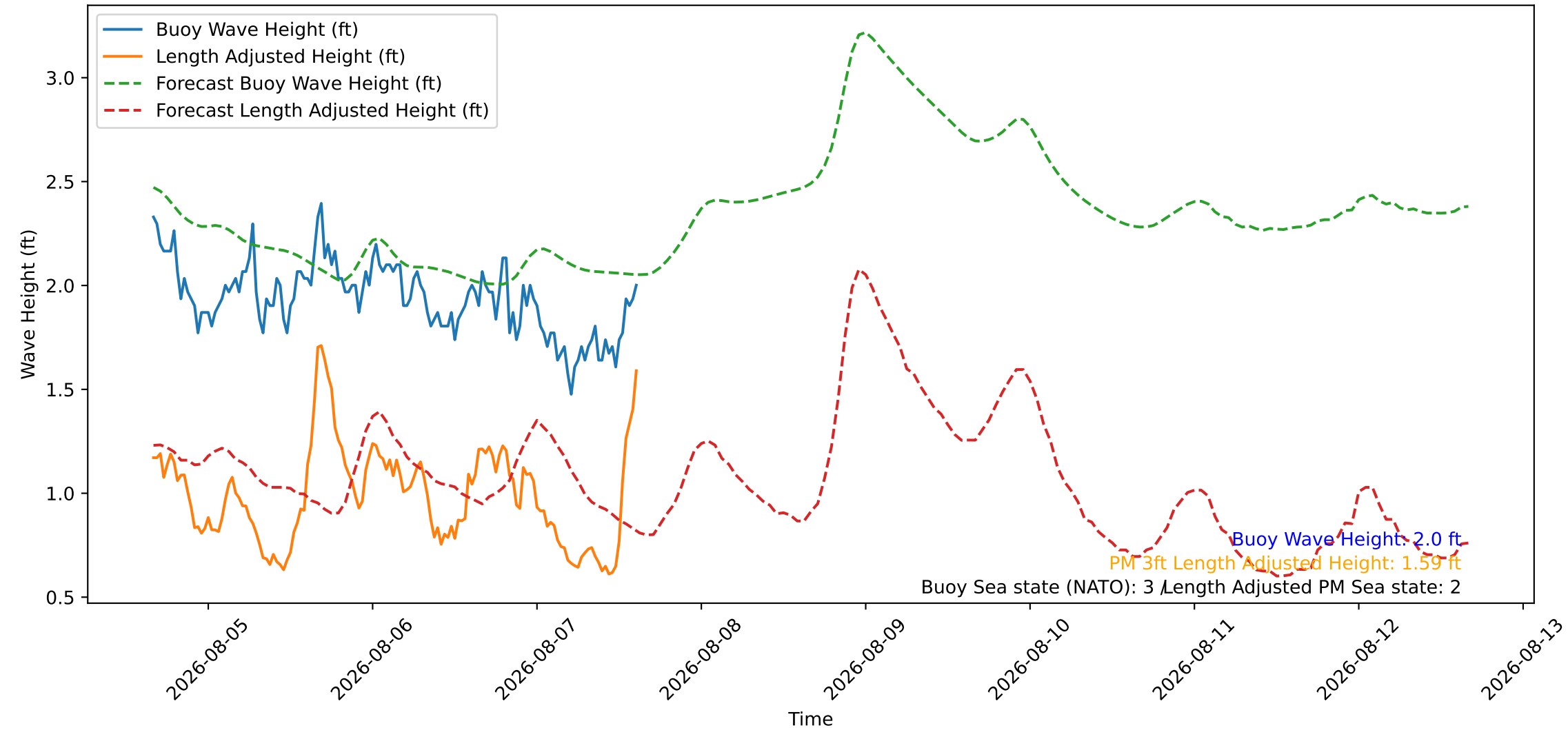
Wave Heights over Time for Red Beach at 2026-08-07 15:30:46
