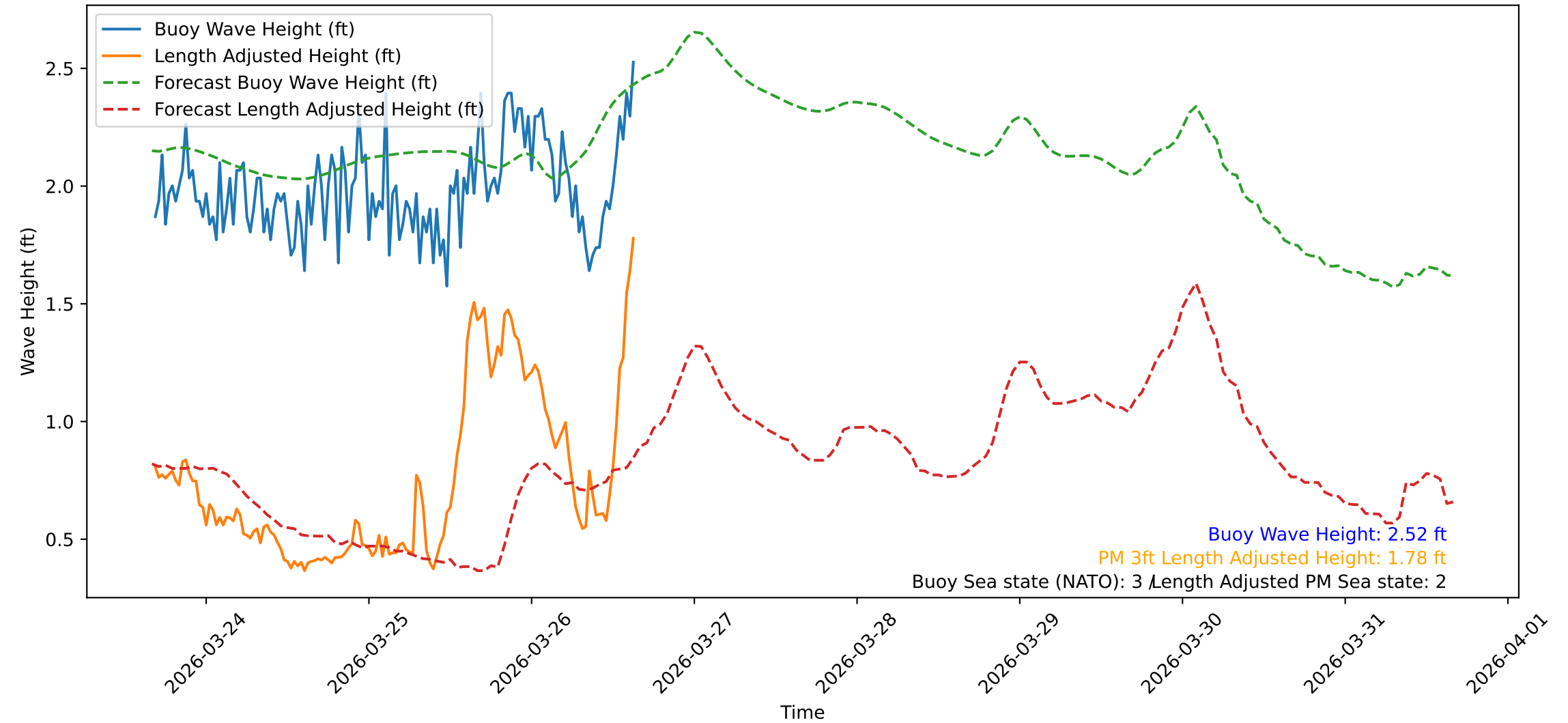
Wave Heights over Time for Red Beach at 2026-03-26 16:00:48
