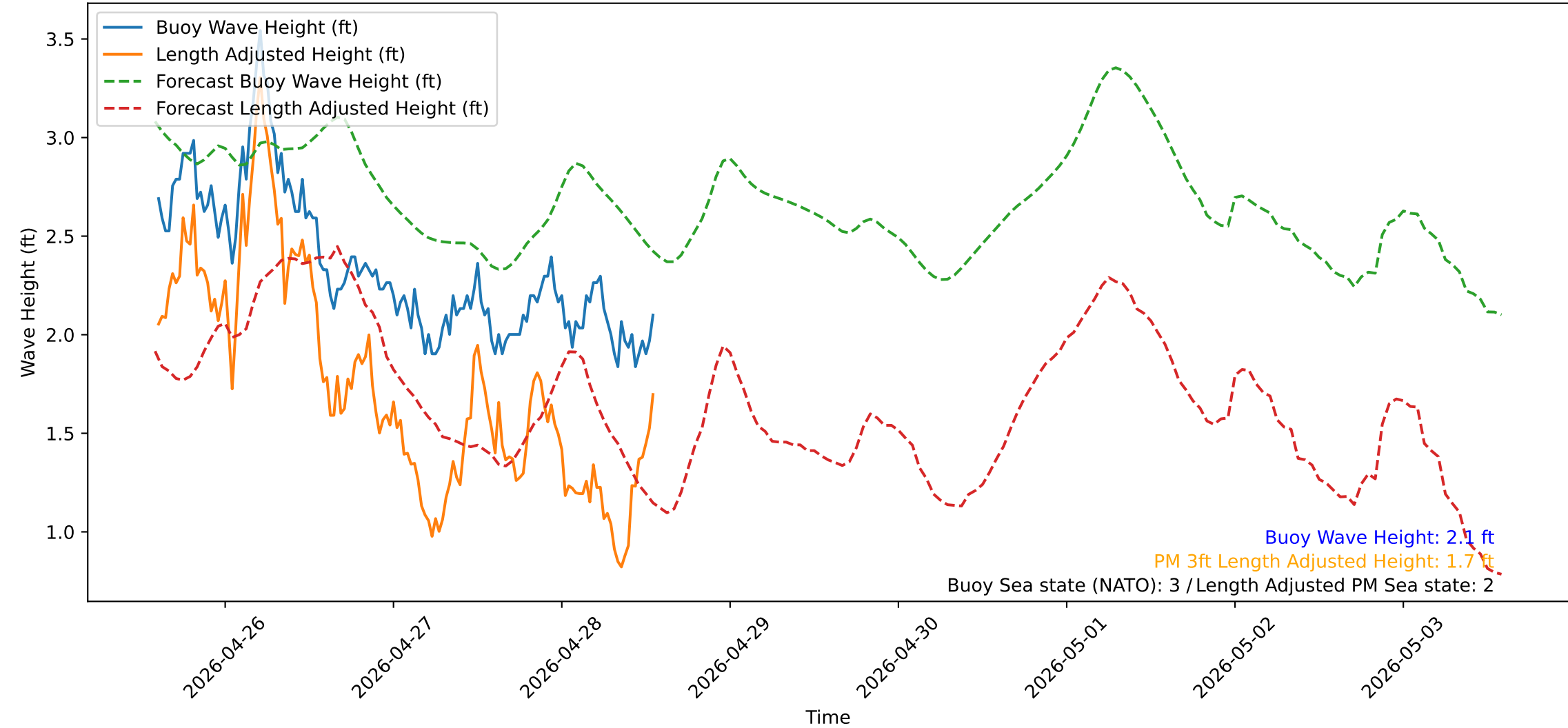
Wave Heights over Time for Red Beach at 2026-04-28 14:00:52
