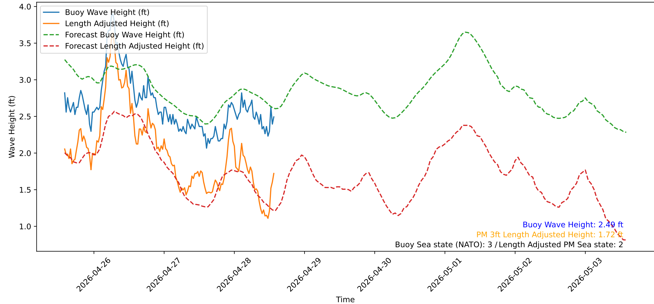
Wave Heights over Time for Oceanside Harbor at 2026-04-28 14:00:32
