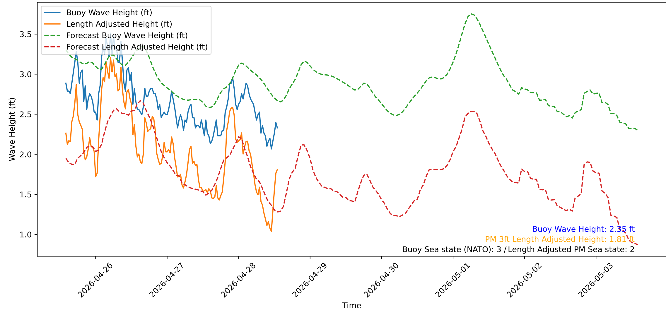
Wave Heights over Time for Green Beach at 2026-04-28 14:01:14
