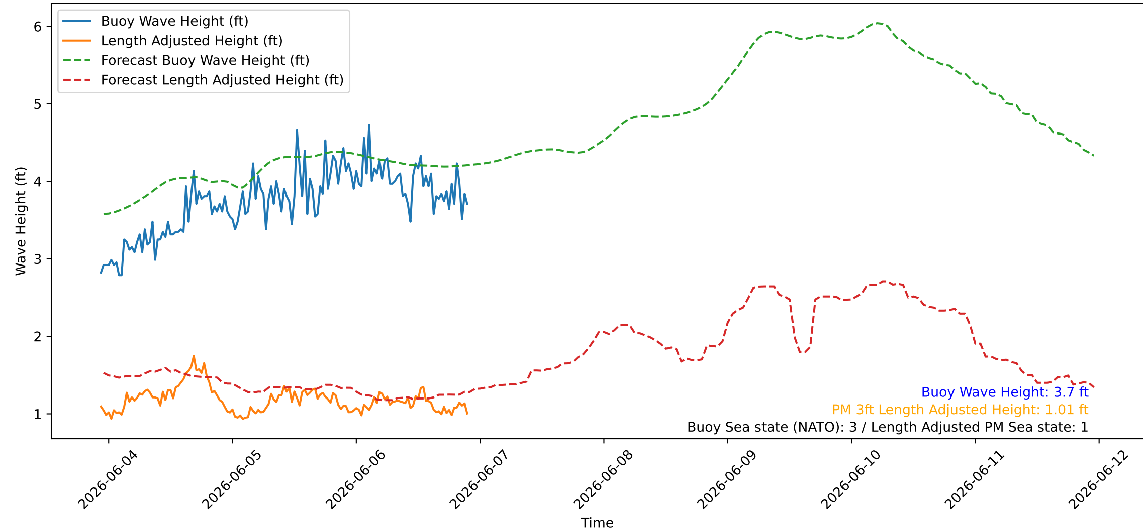
Wave Heights over Time for Green Beach at 2026-06-06 22:31:08
