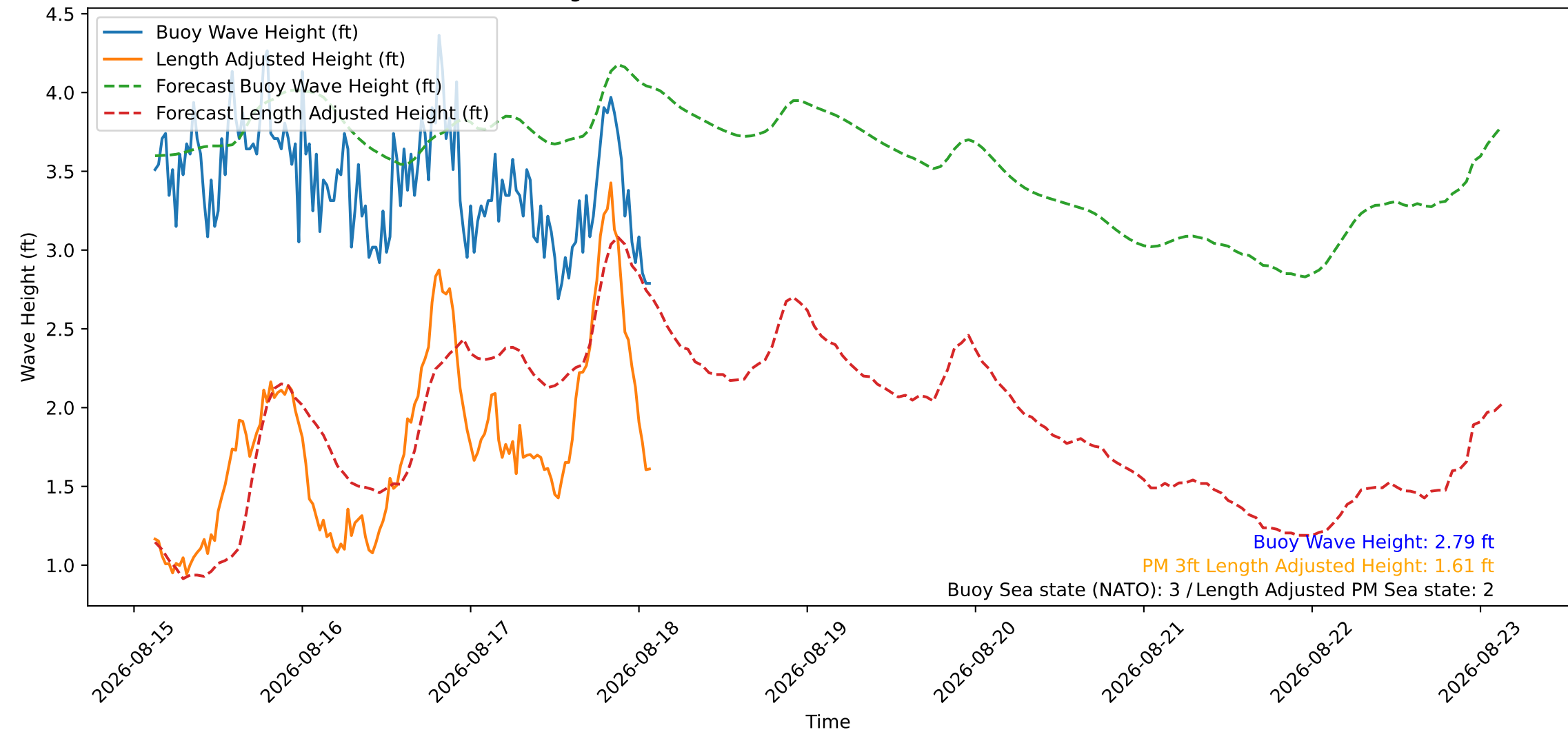
Wave Heights over Time for Green Beach at 2026-08-18 02:31:08
