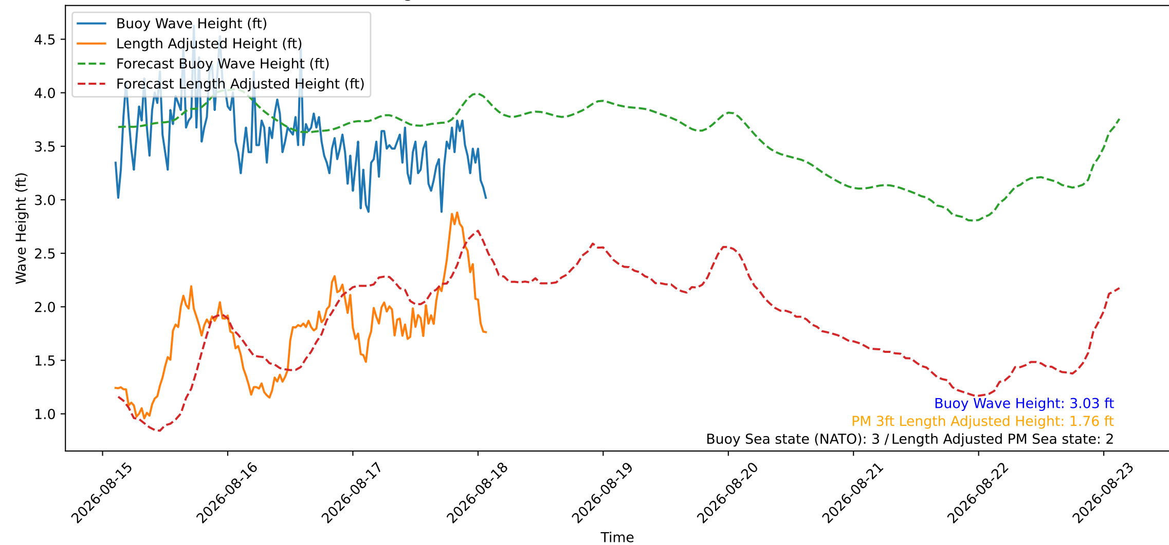
Wave Heights over Time for Oceanside Harbor at 2026-08-18 02:30:26
