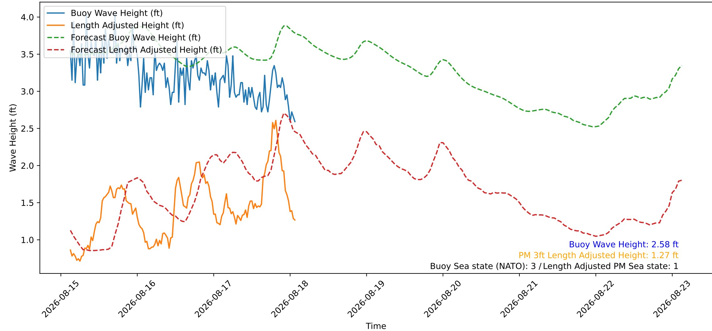
Wave Heights over Time for Red Beach at 2026-08-18 02:30:46
