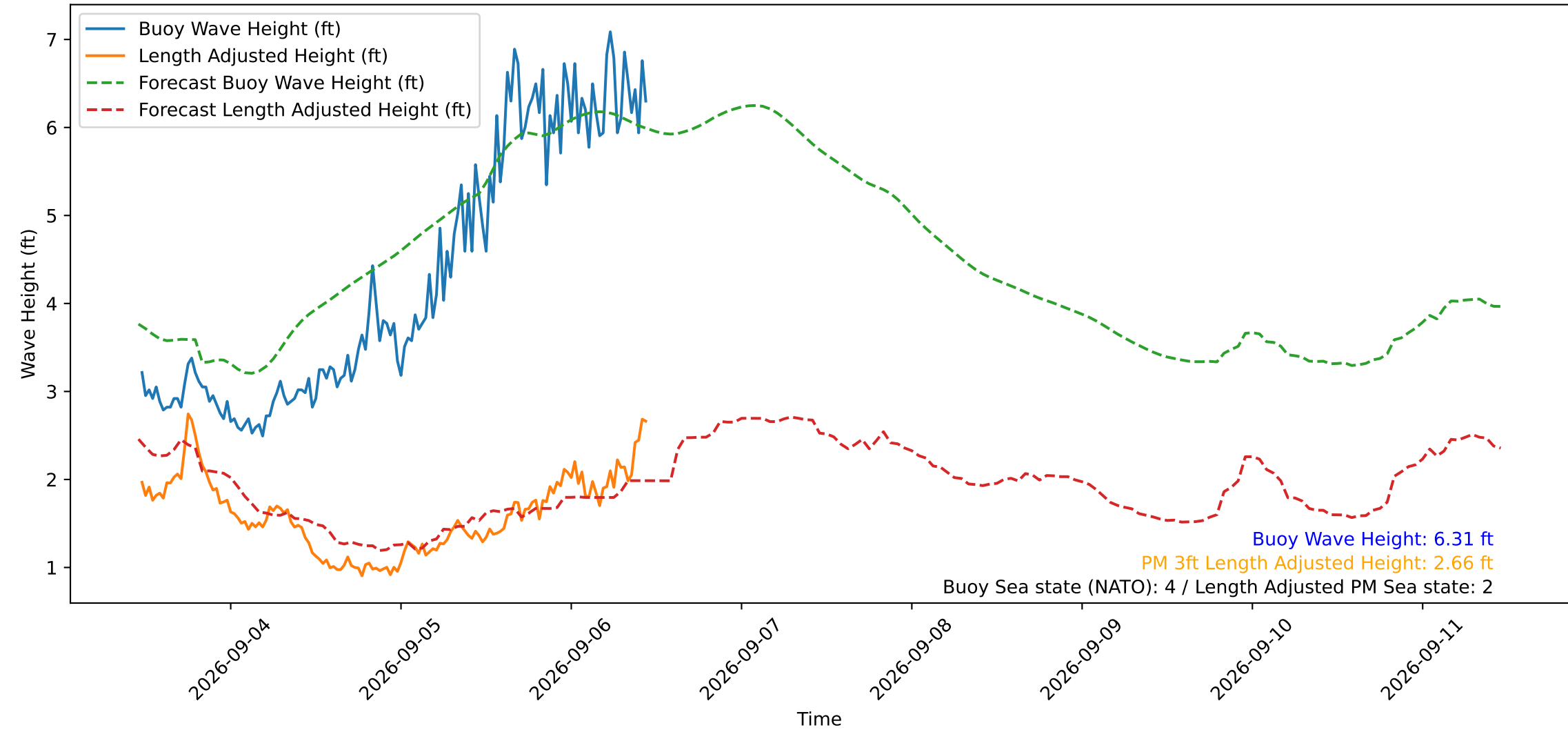
Wave Heights over Time for Green Beach at 2026-09-06 11:11:13
