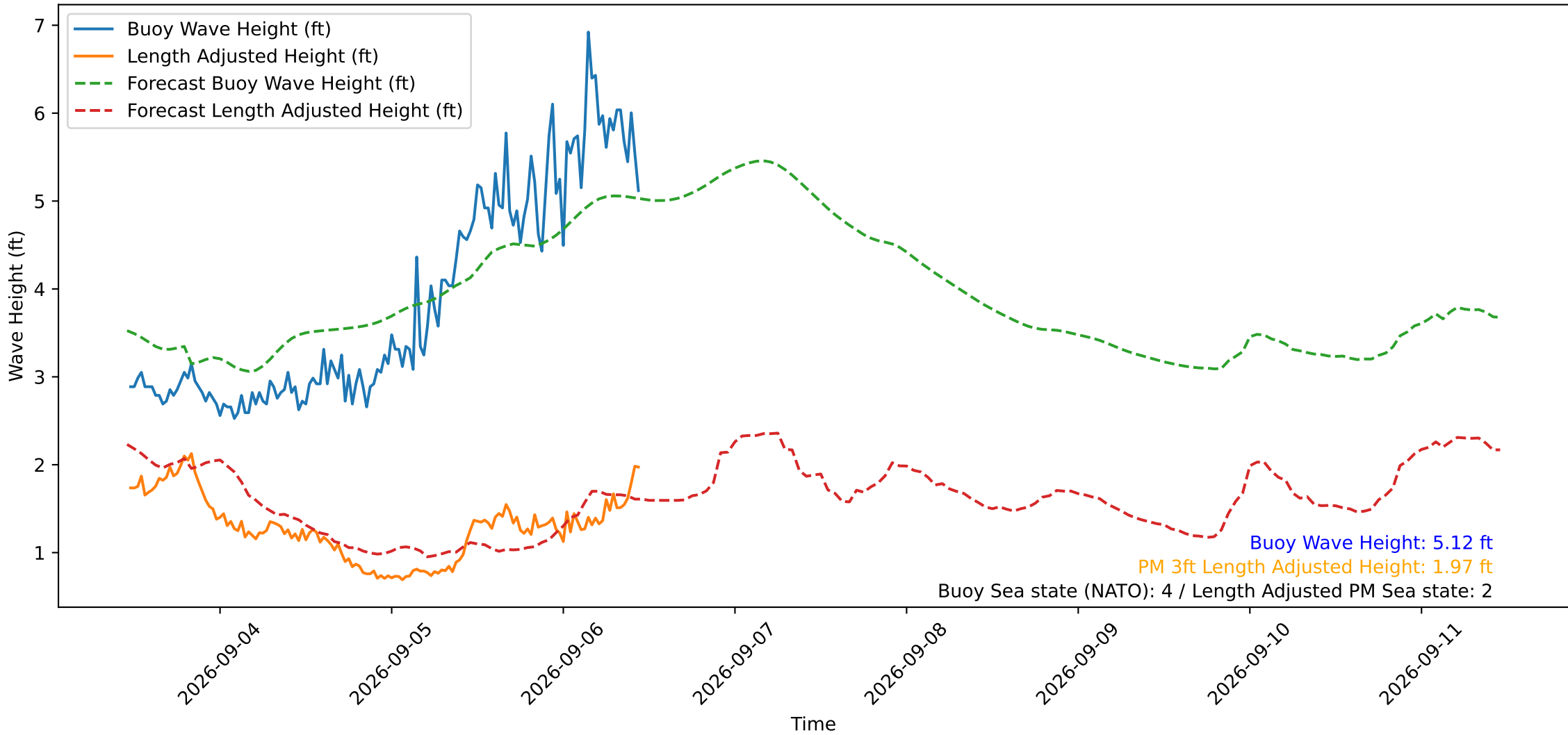
Wave Heights over Time for Red Beach at 2026-09-06 11:10:50
