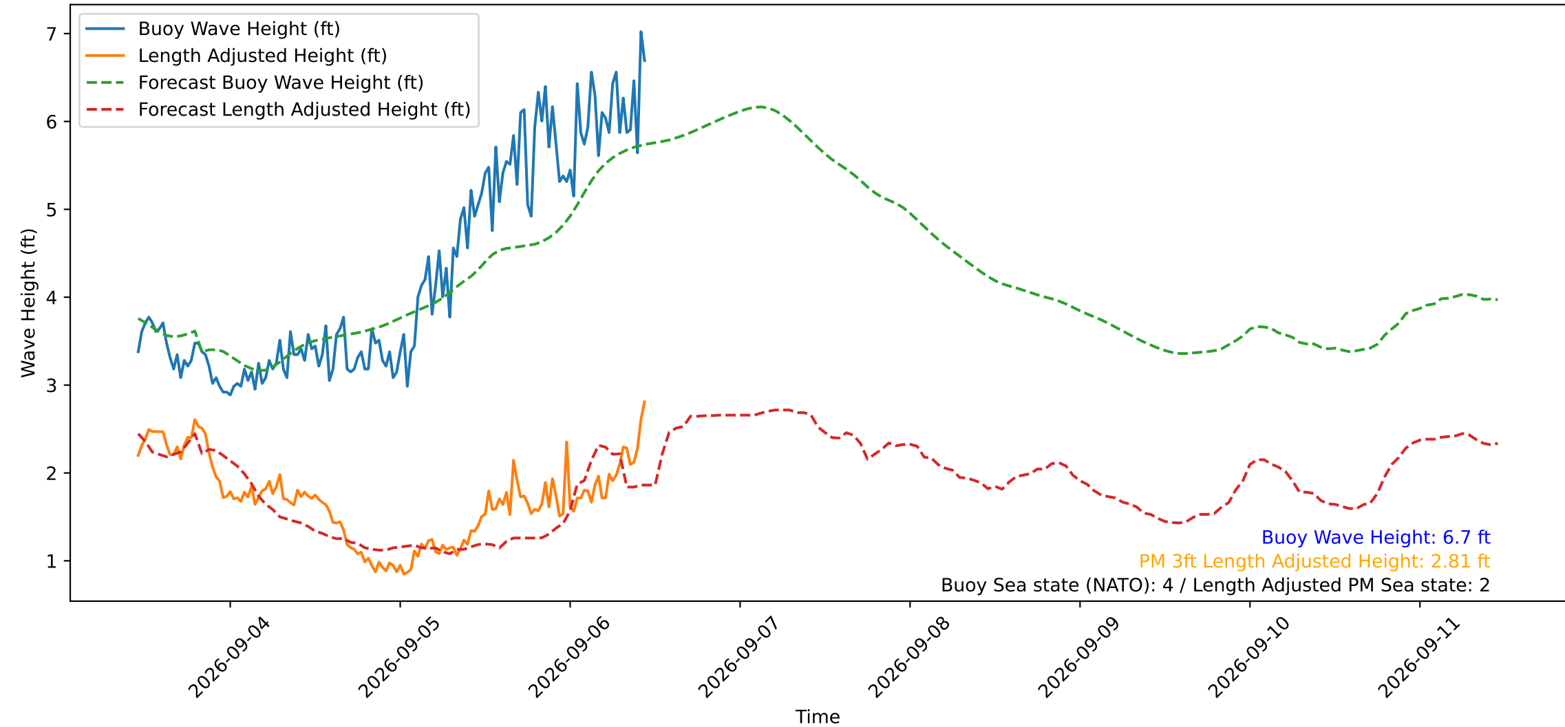
Wave Heights over Time for Oceanside Harbor at 2026-09-06 11:10:30
