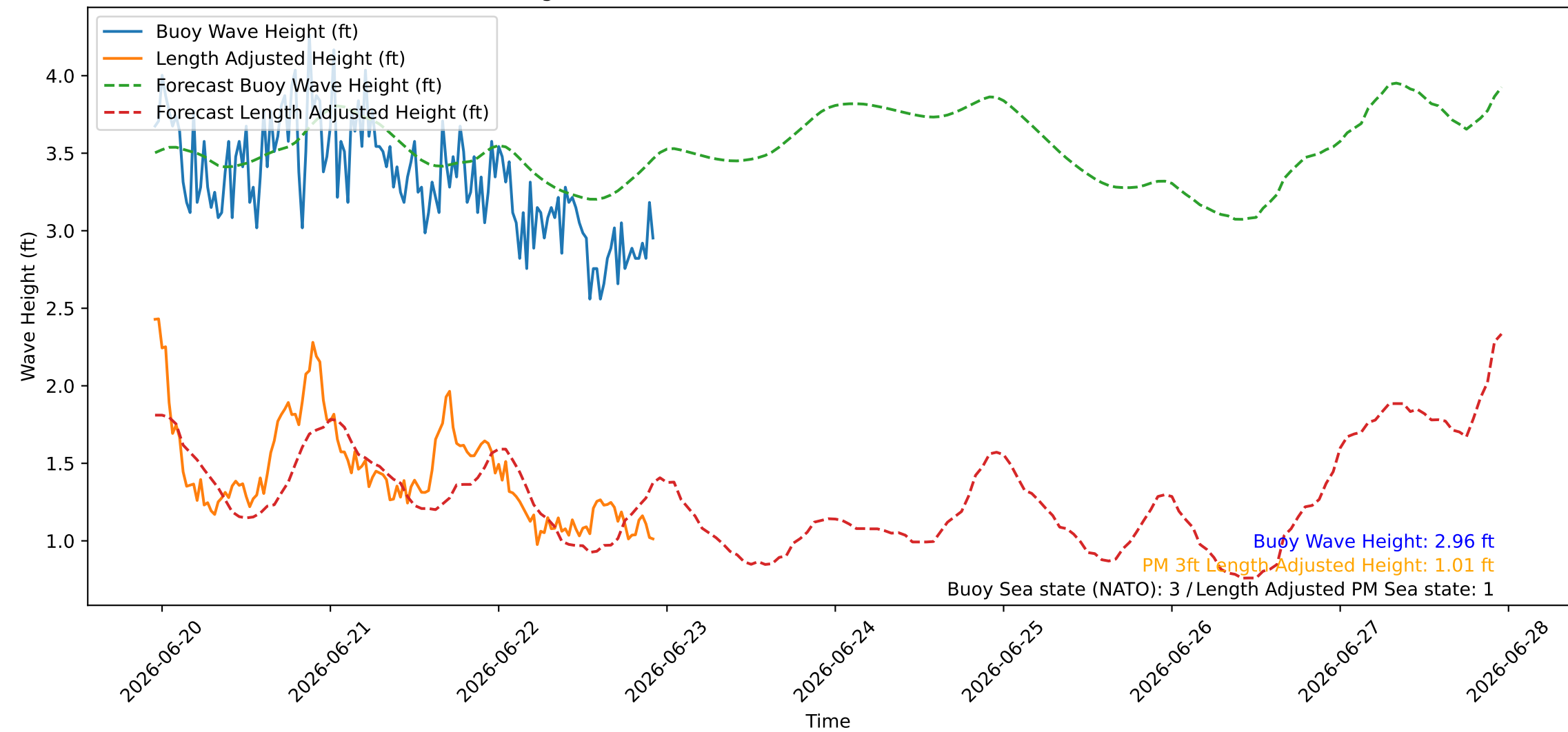
Wave Heights over Time for Oceanside Harbor at 2026-06-22 22:50:26
