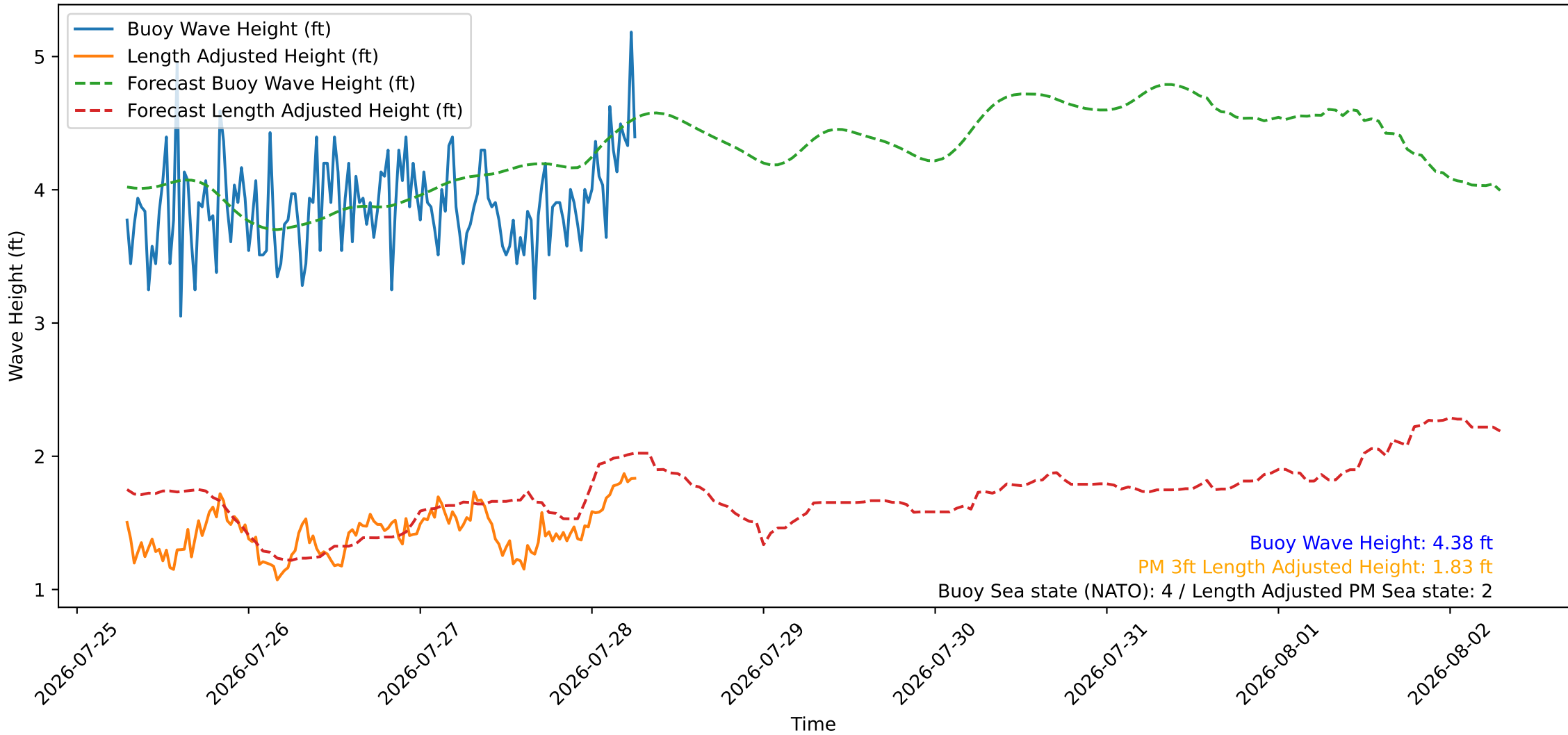
Wave Heights over Time for Oceanside Harbor at 2026-07-28 07:00:26
