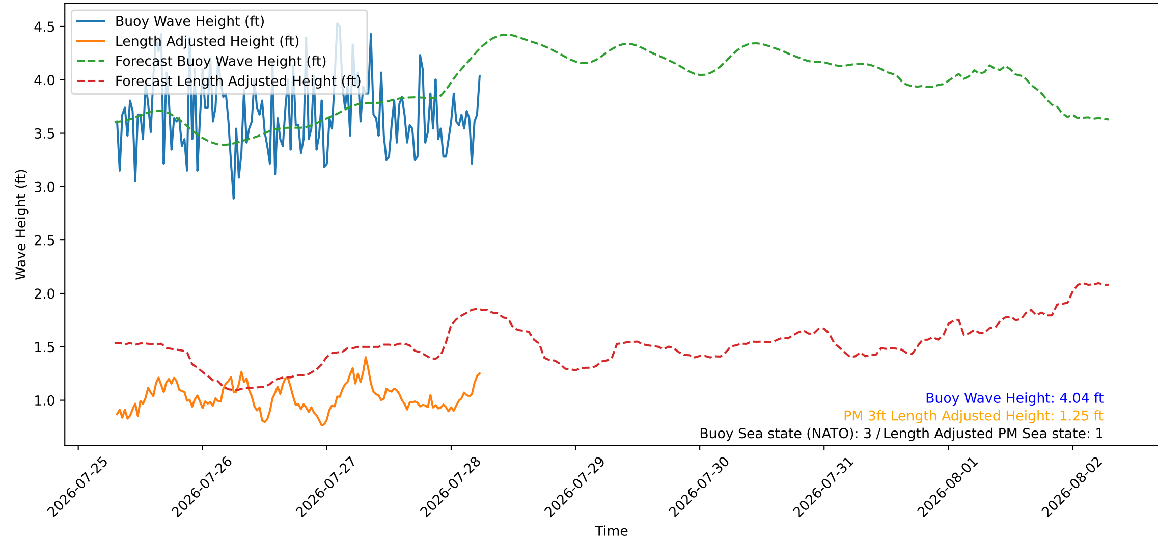
Wave Heights over Time for Red Beach at 2026-07-28 07:00:45
