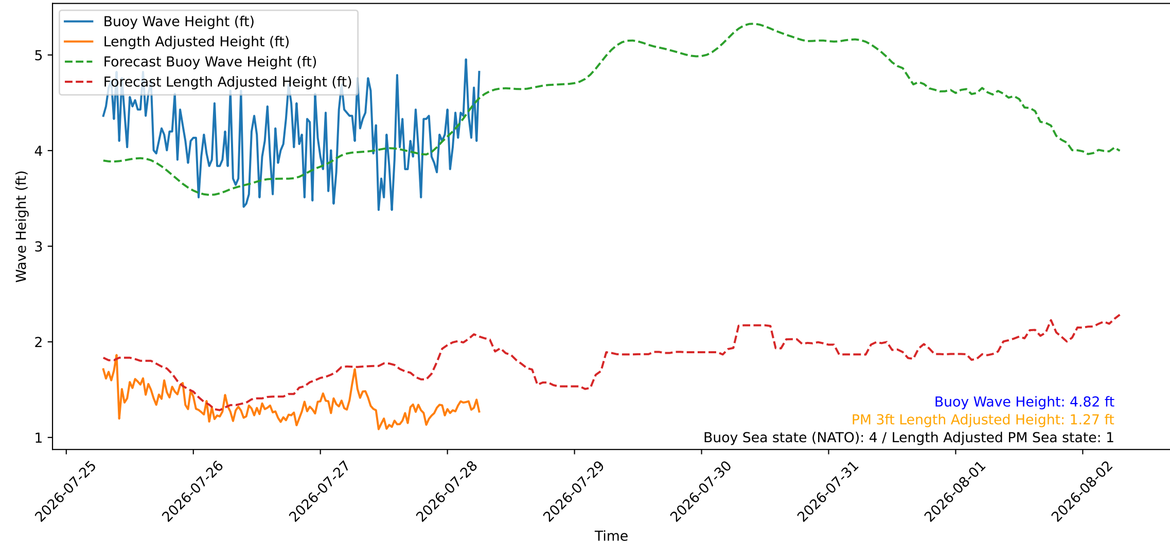
Wave Heights over Time for Green Beach at 2026-07-28 07:01:08
