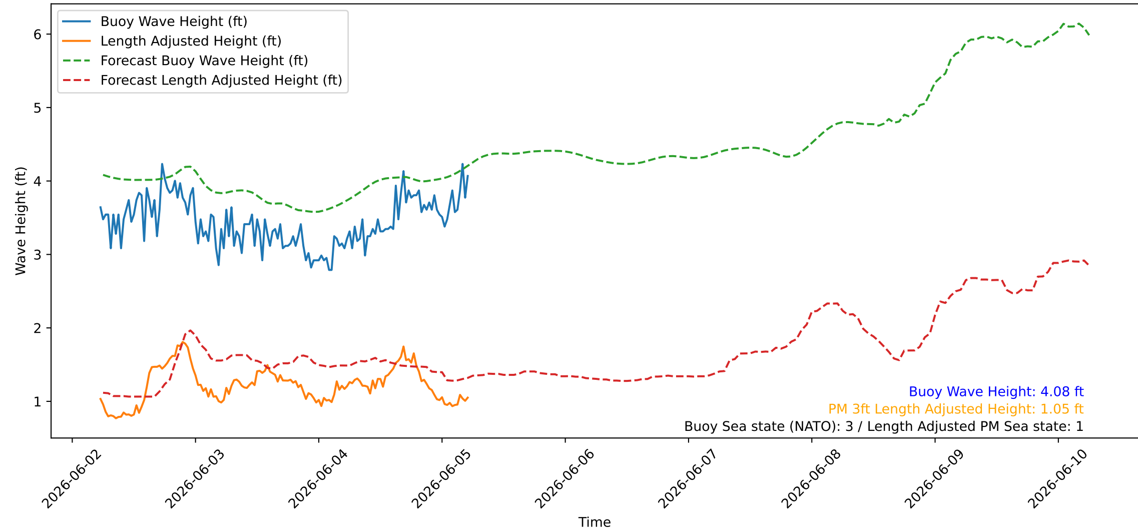
Wave Heights over Time for Green Beach at 2026-06-05 05:41:08
