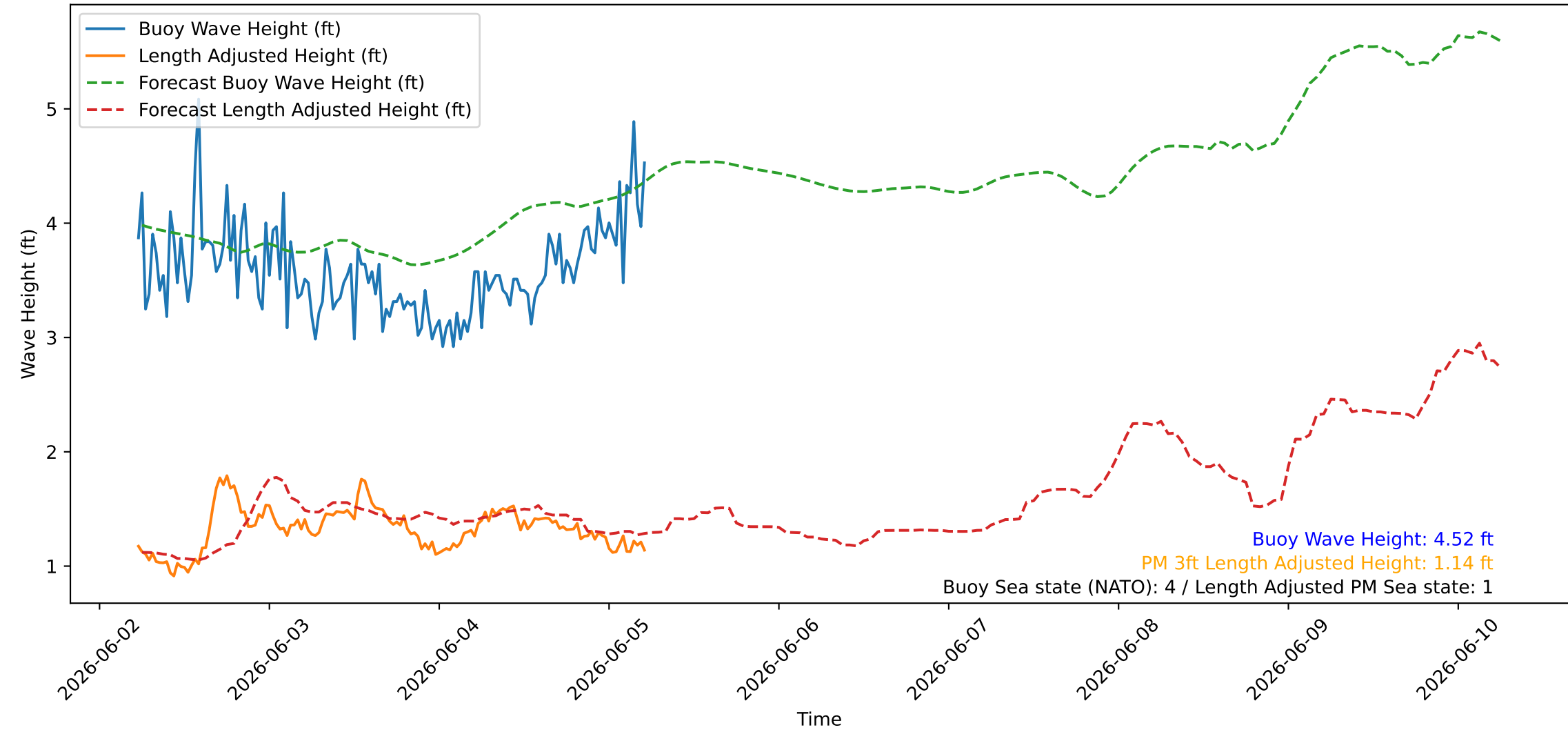
Wave Heights over Time for Oceanside Harbor at 2026-06-05 05:40:26
