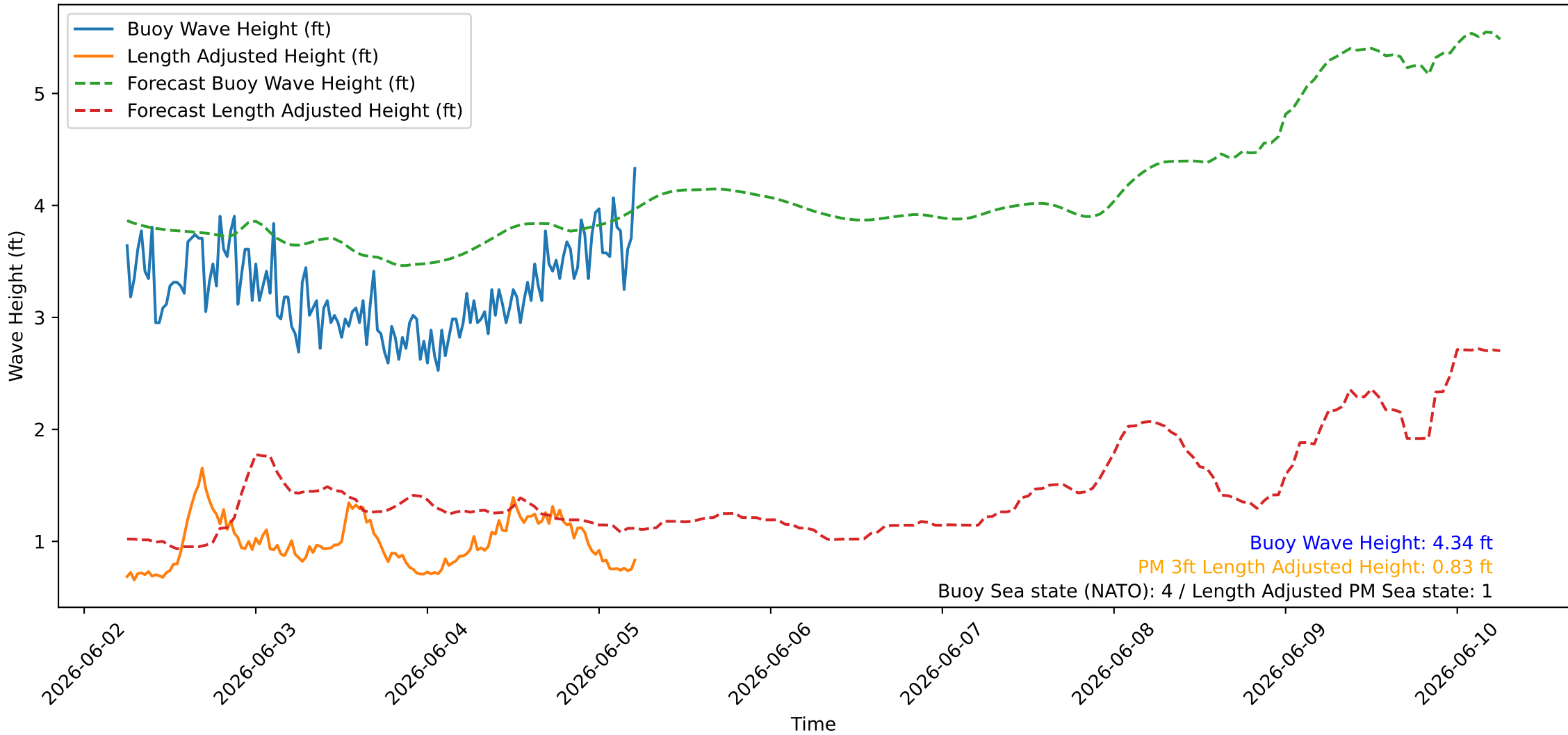
Wave Heights over Time for Red Beach at 2026-06-05 05:40:45
