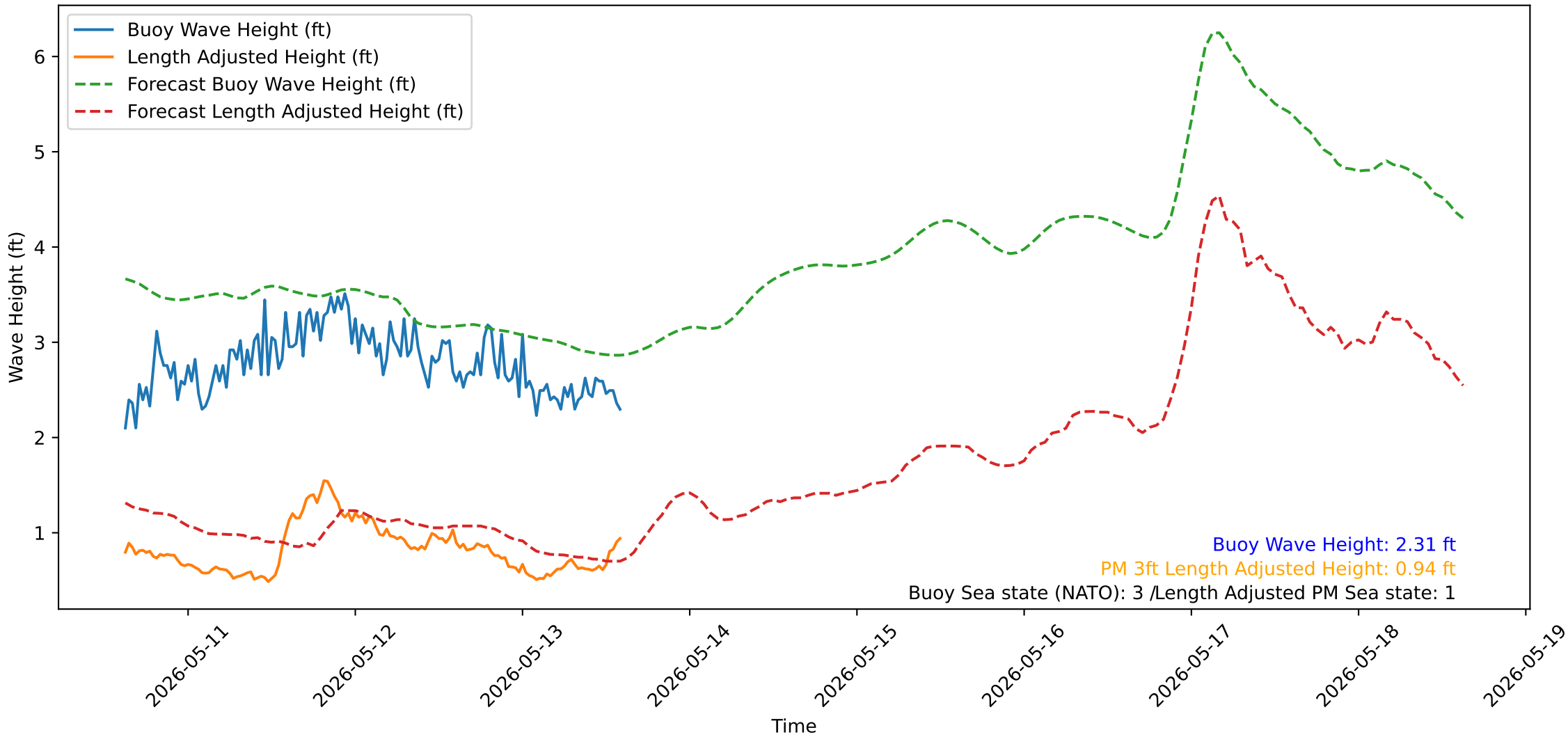
Wave Heights over Time for Green Beach at 2026-05-13 14:51:14
