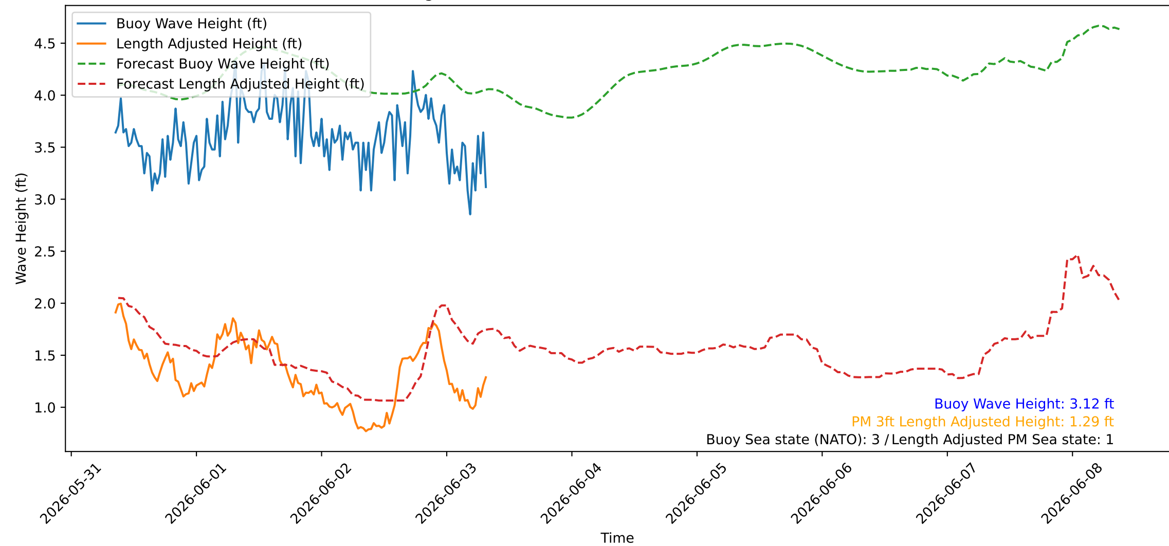
Wave Heights over Time for Green Beach at 2026-06-03 08:31:08
