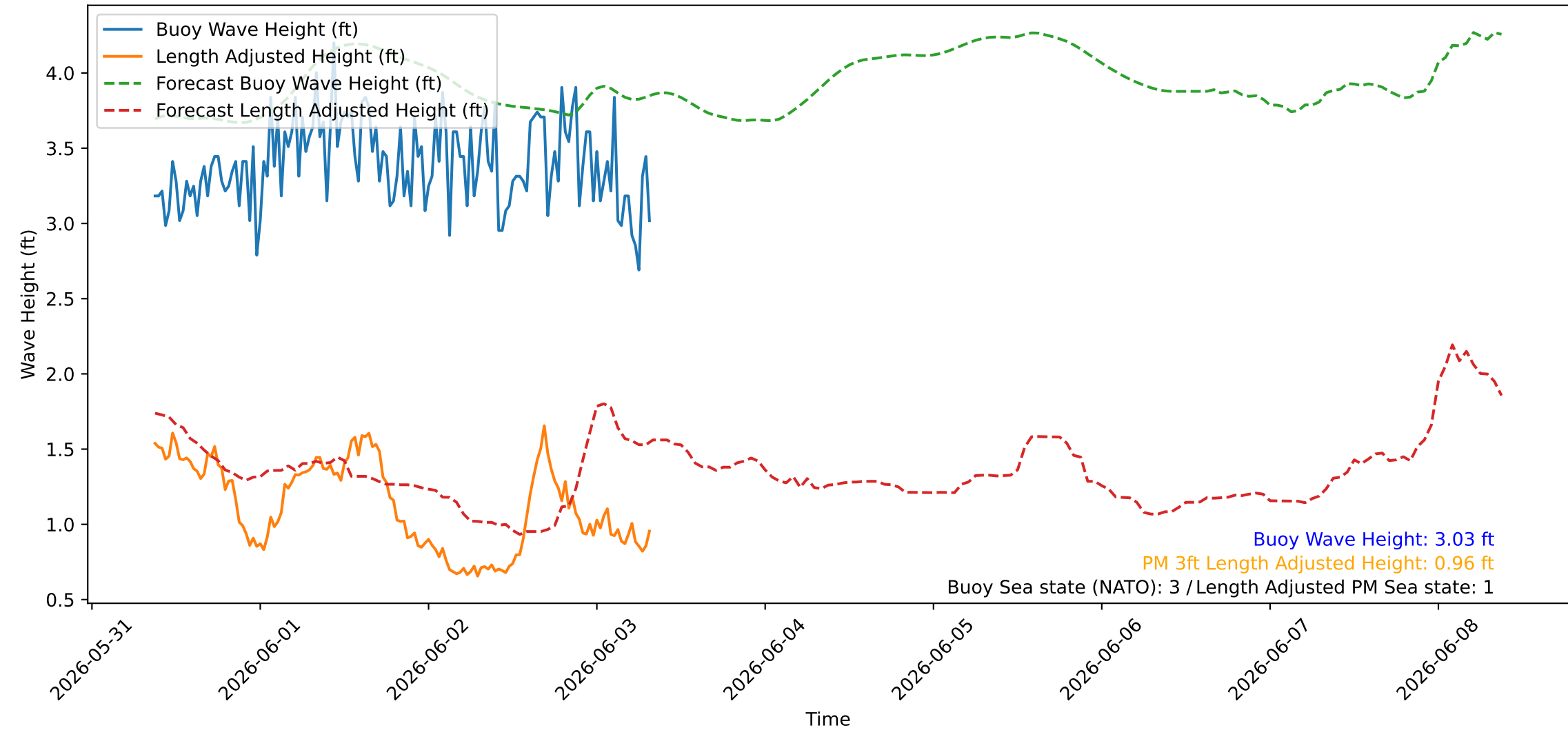
Wave Heights over Time for Red Beach at 2026-06-03 08:30:45
