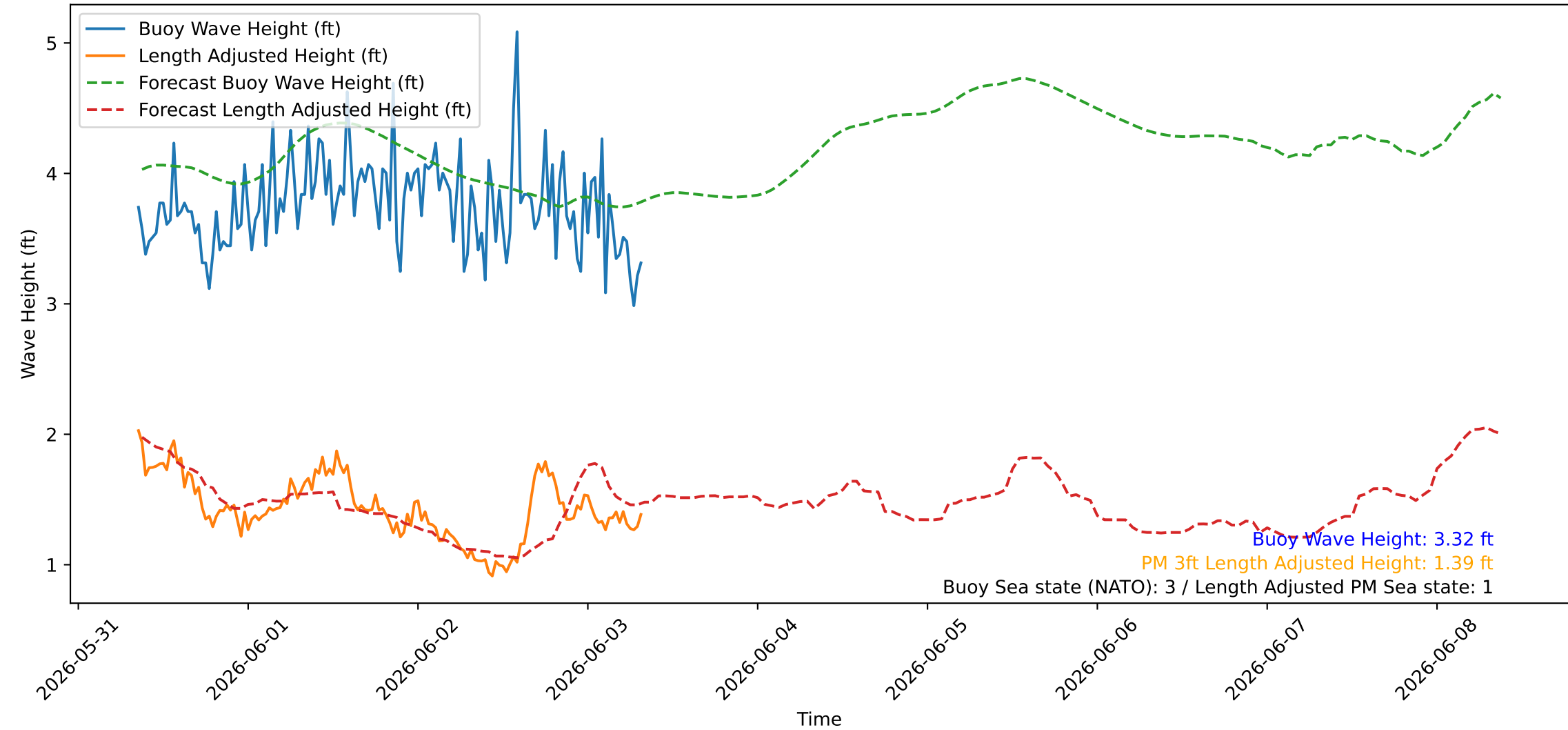
Wave Heights over Time for Oceanside Harbor at 2026-06-03 08:30:26
