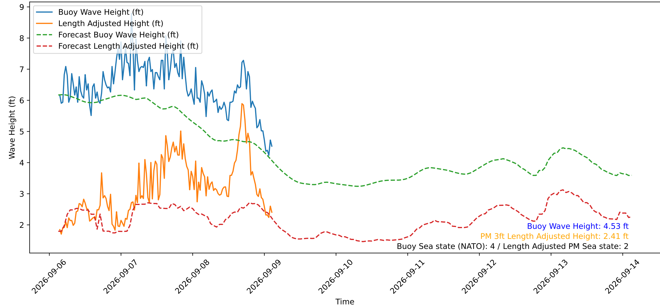
Wave Heights over Time for Green Beach at 2026-09-09 03:11:11
