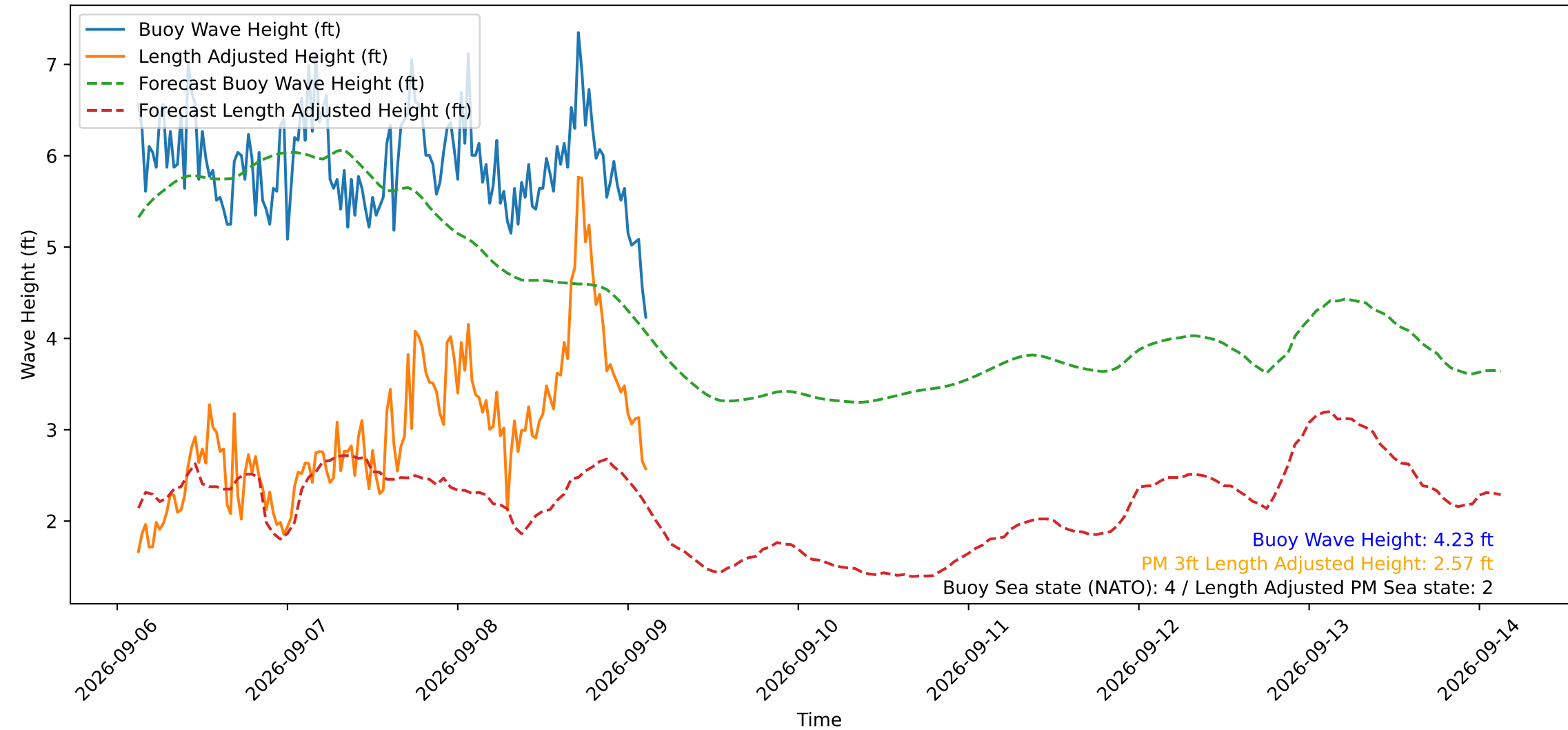
Wave Heights over Time for Oceanside Harbor at 2026-09-09 03:10:30
