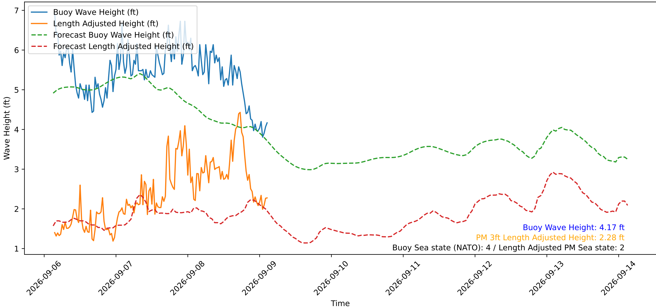
Wave Heights over Time for Red Beach at 2026-09-09 03:10:49
