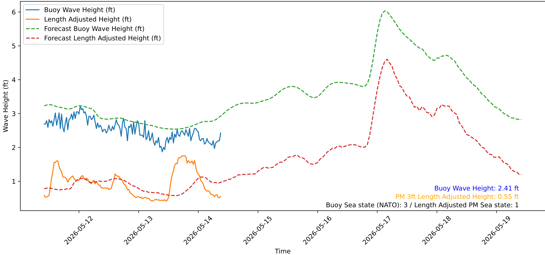
Wave Heights over Time for Red Beach at 2026-05-14 09:40:51
