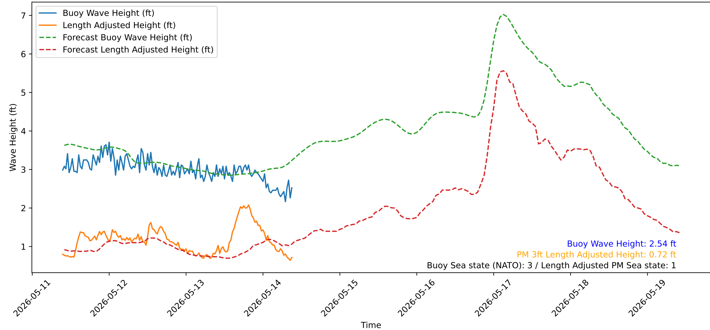
Wave Heights over Time for Oceanside Harbor at 2026-05-14 09:40:31
