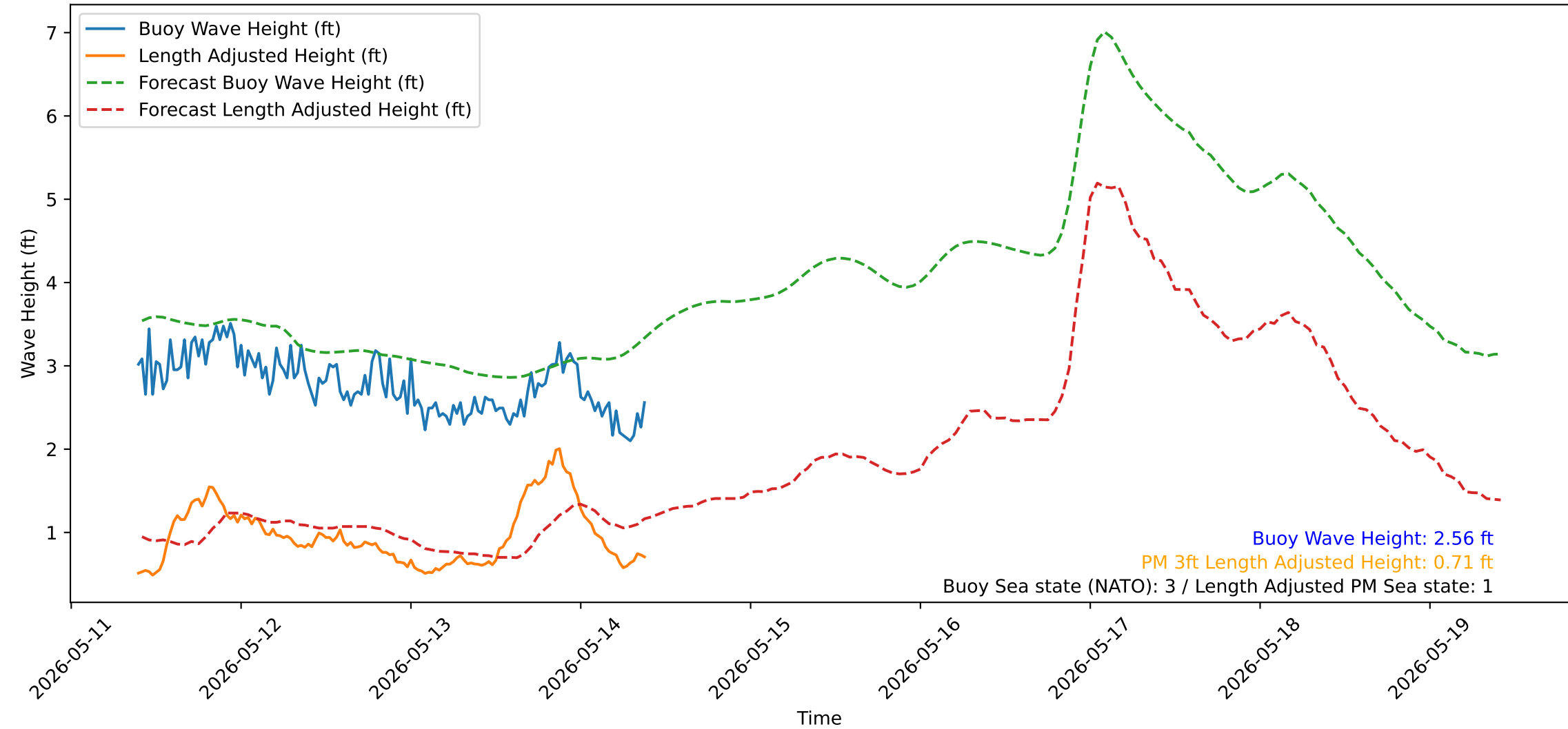
Wave Heights over Time for Green Beach at 2026-05-14 09:41:13
