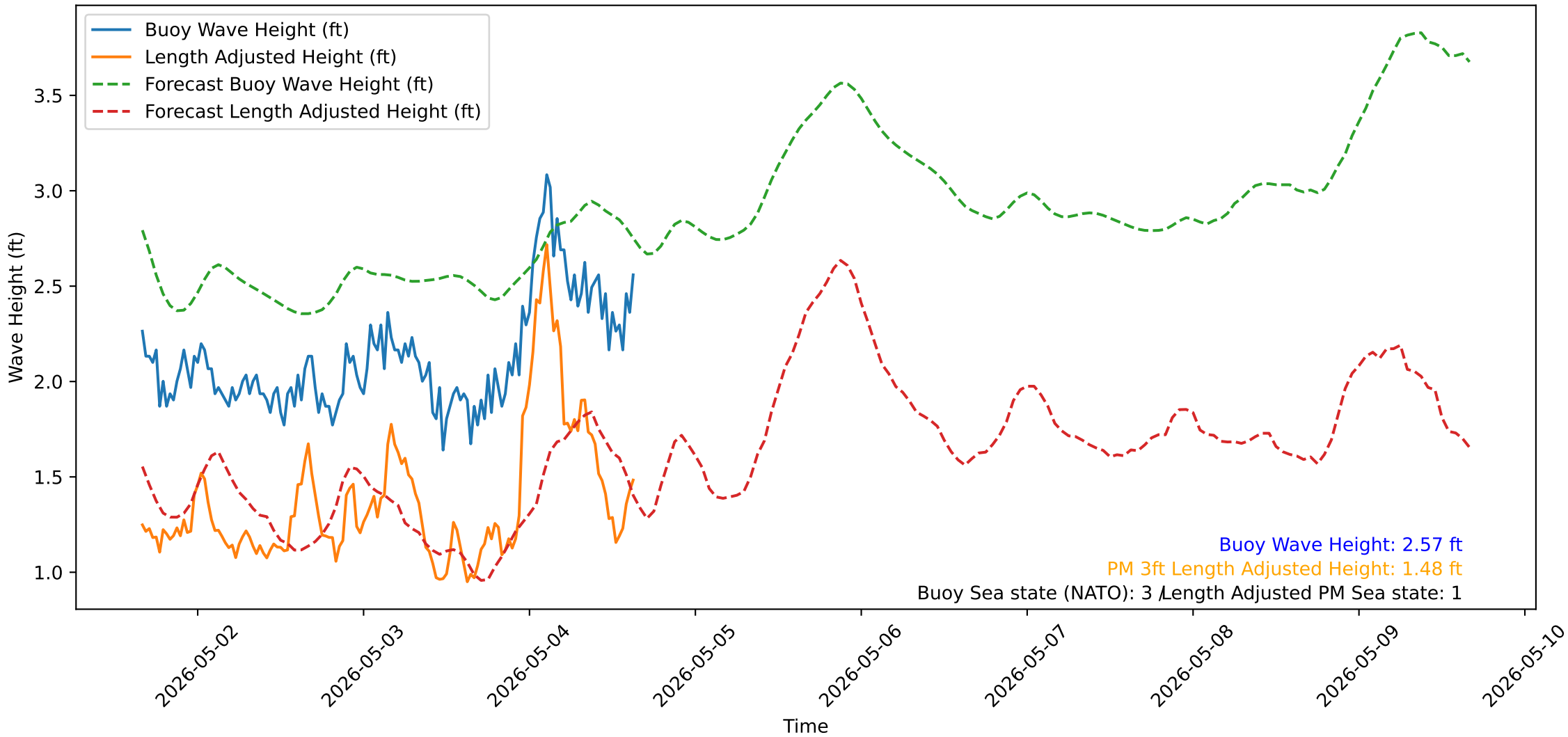
Wave Heights over Time for Oceanside Harbor at 2026-05-04 16:00:31
