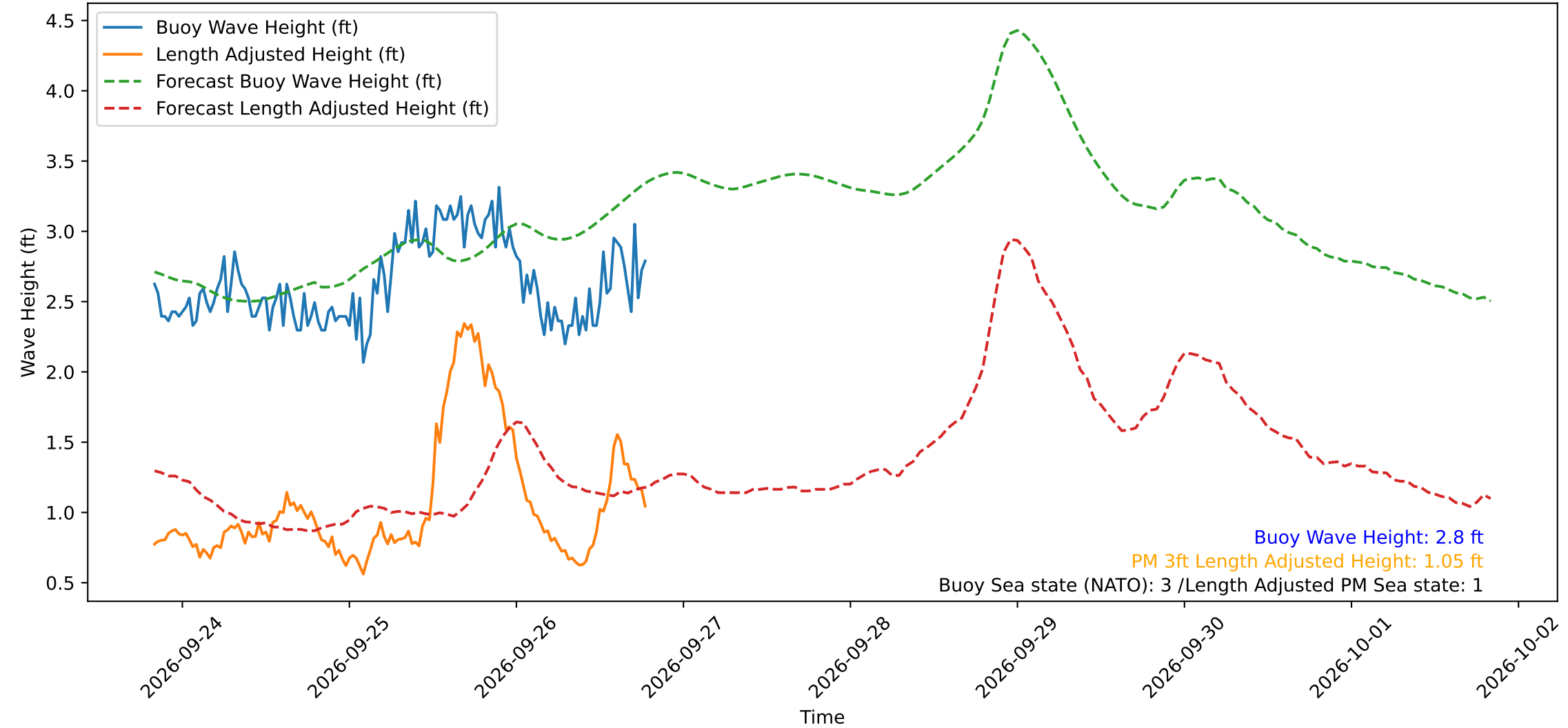
Wave Heights over Time for Red Beach at 2026-09-26 19:30:50
