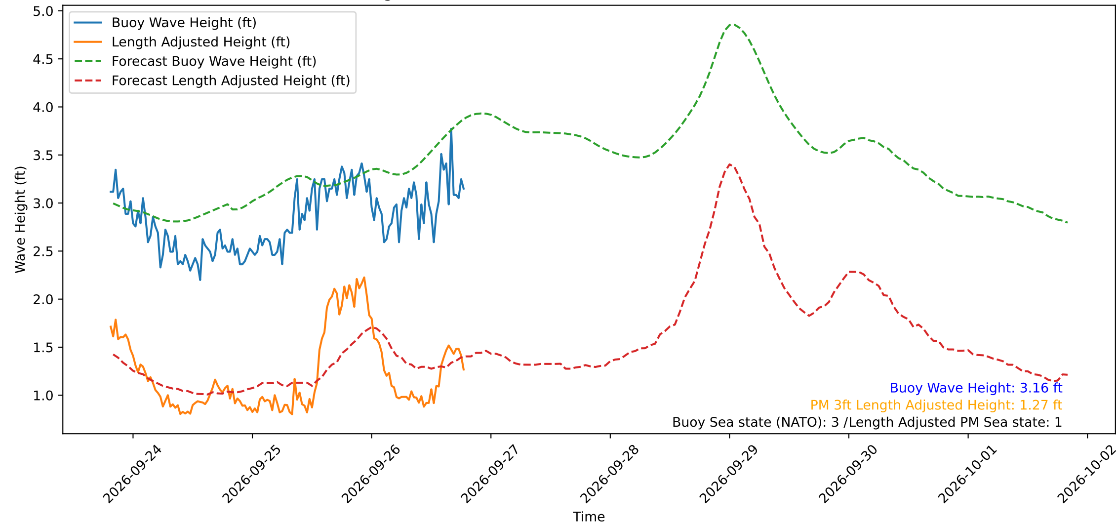
Wave Heights over Time for Oceanside Harbor at 2026-09-26 19:30:30
