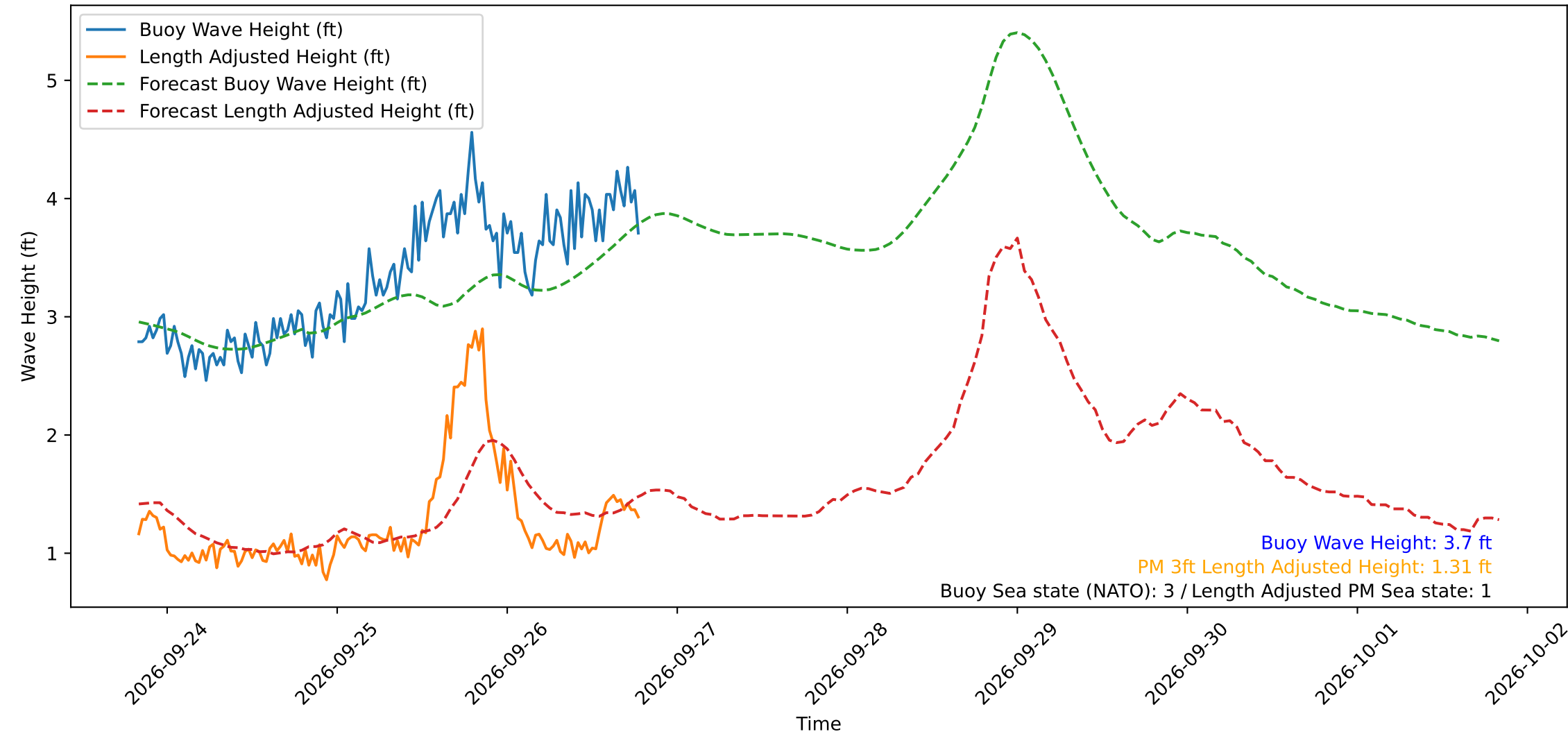
Wave Heights over Time for Green Beach at 2026-09-26 19:31:13
