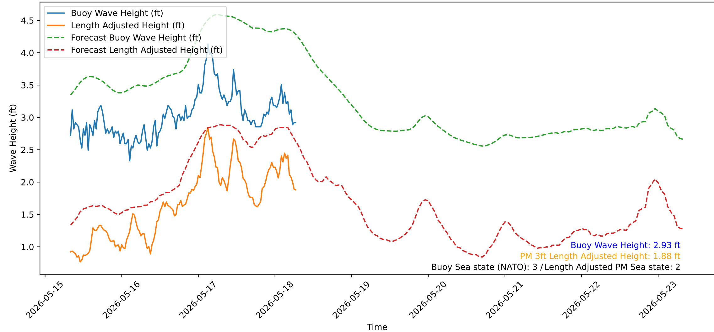
Wave Heights over Time for Red Beach at 2026-05-18 07:30:51
