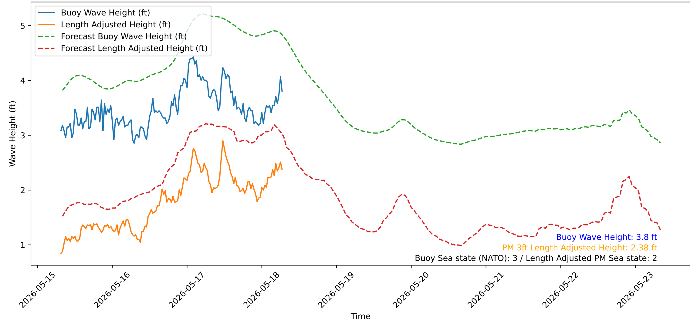
Wave Heights over Time for Green Beach at 2026-05-18 07:31:14
