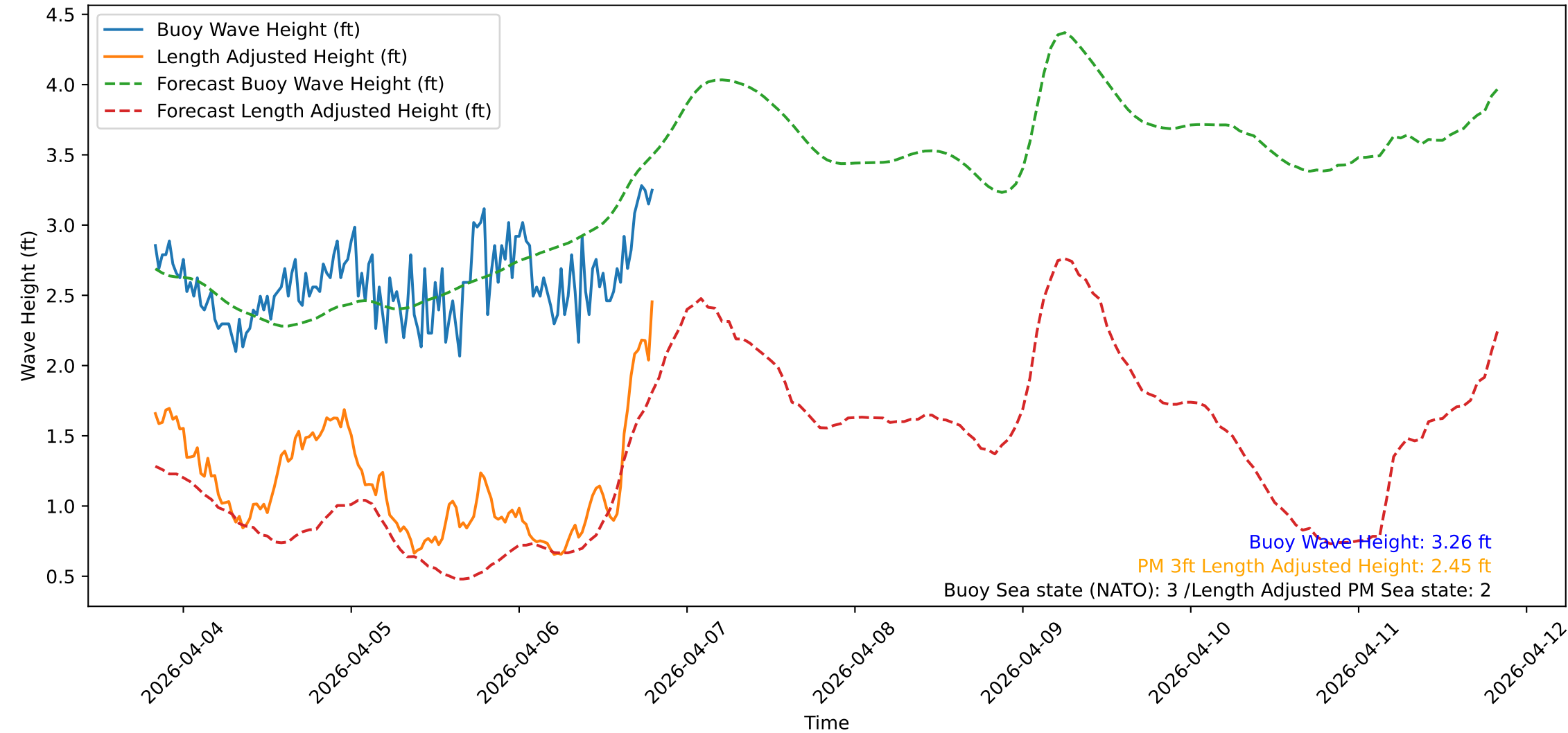
Wave Heights over Time for Oceanside Harbor at 2026-04-06 19:50:31
