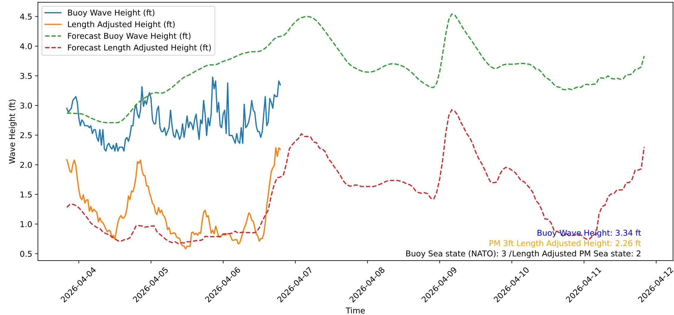
Wave Heights over Time for Green Beach at 2026-04-06 19:51:10
