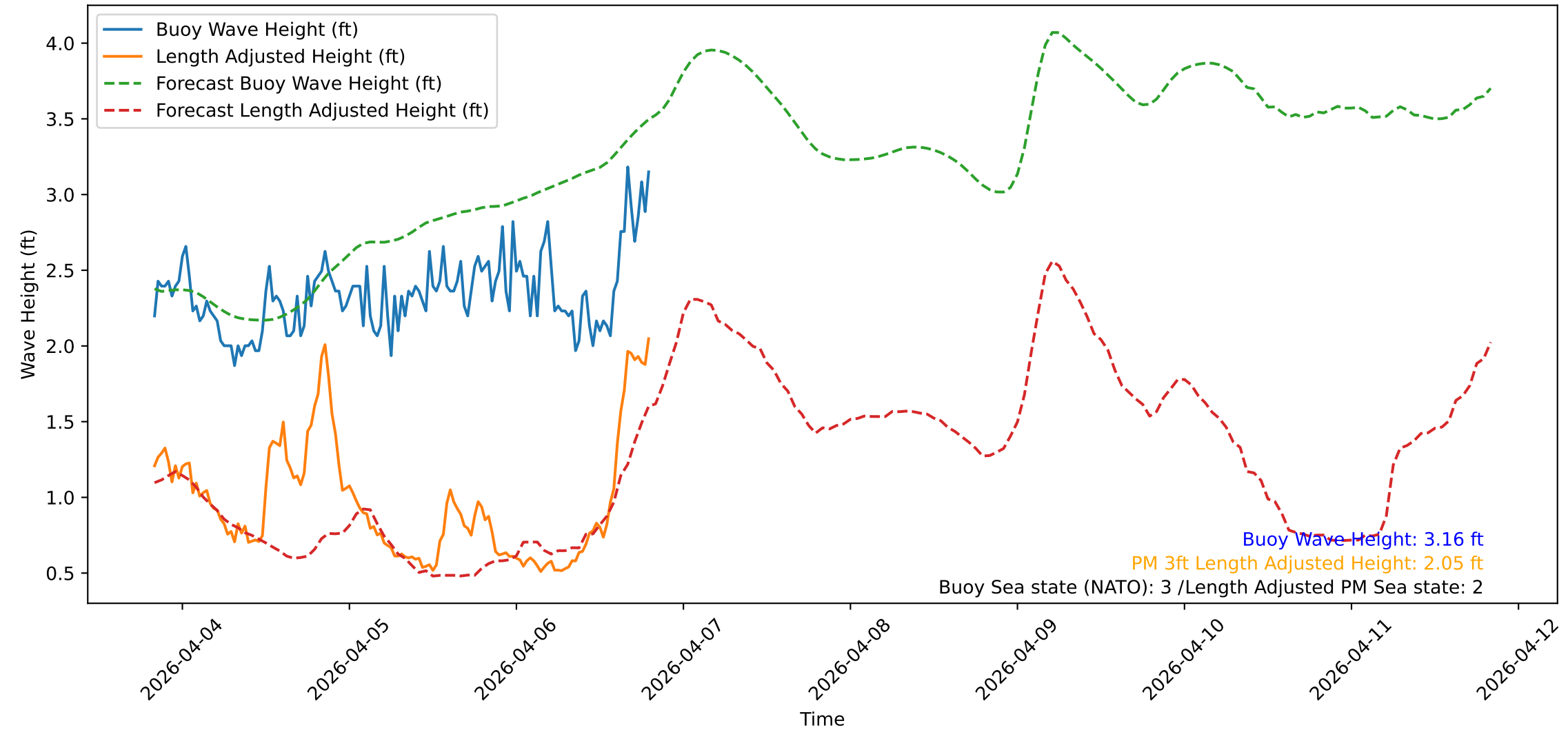
Wave Heights over Time for Red Beach at 2026-04-06 19:50:47
