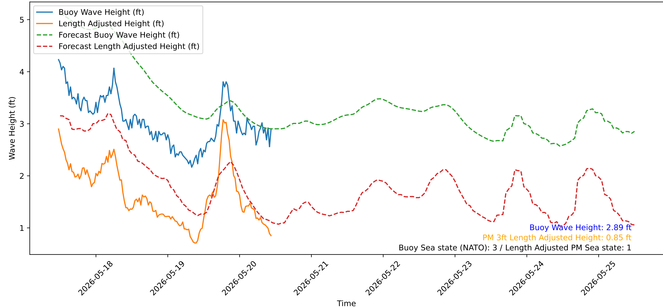
Wave Heights over Time for Green Beach at 2026-05-20 11:31:14
