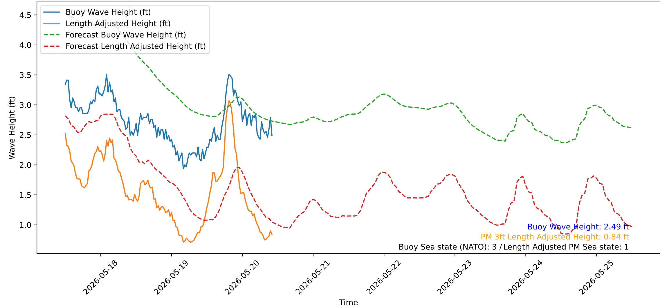
Wave Heights over Time for Red Beach at 2026-05-20 11:30:51
