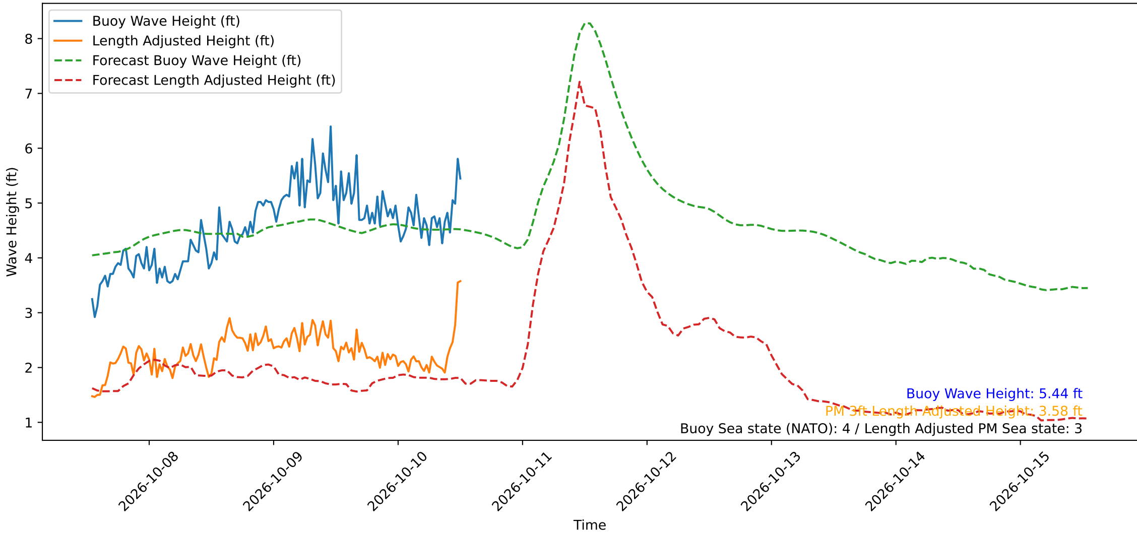
Wave Heights over Time for Oceanside Harbor at 2026-10-10 13:10:29
