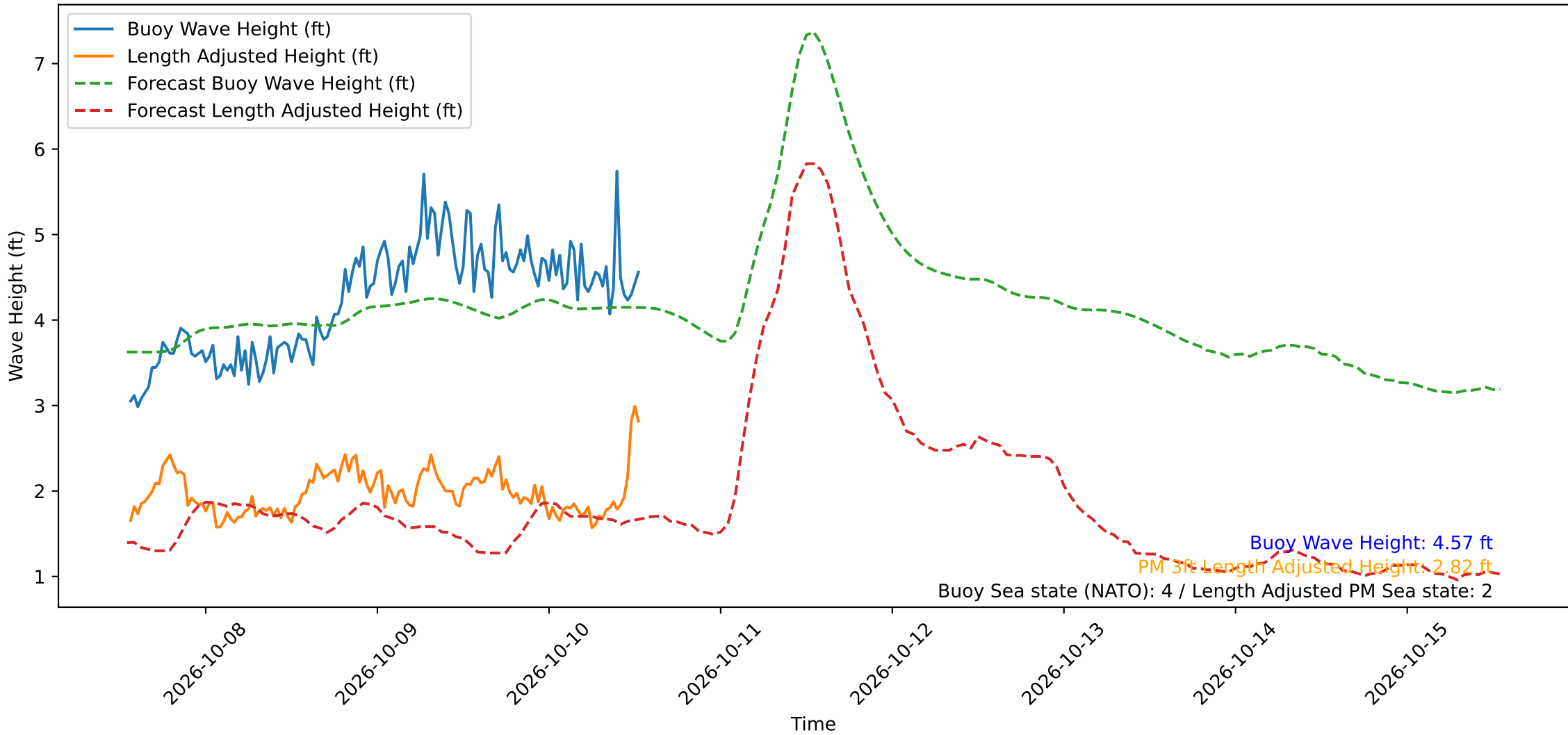
Wave Heights over Time for Red Beach at 2026-10-10 13:10:49
