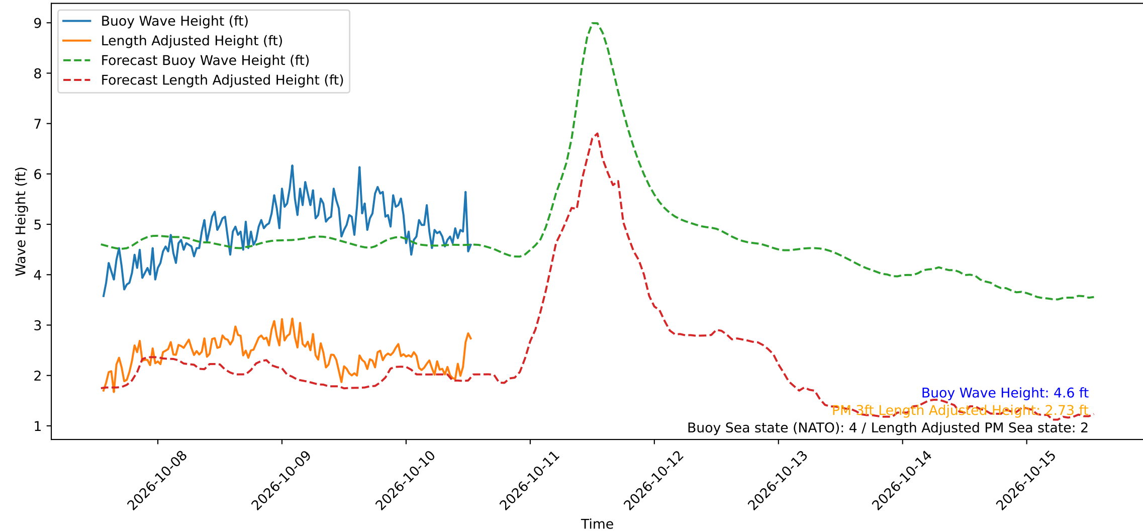
Wave Heights over Time for Green Beach at 2026-10-10 13:11:11
