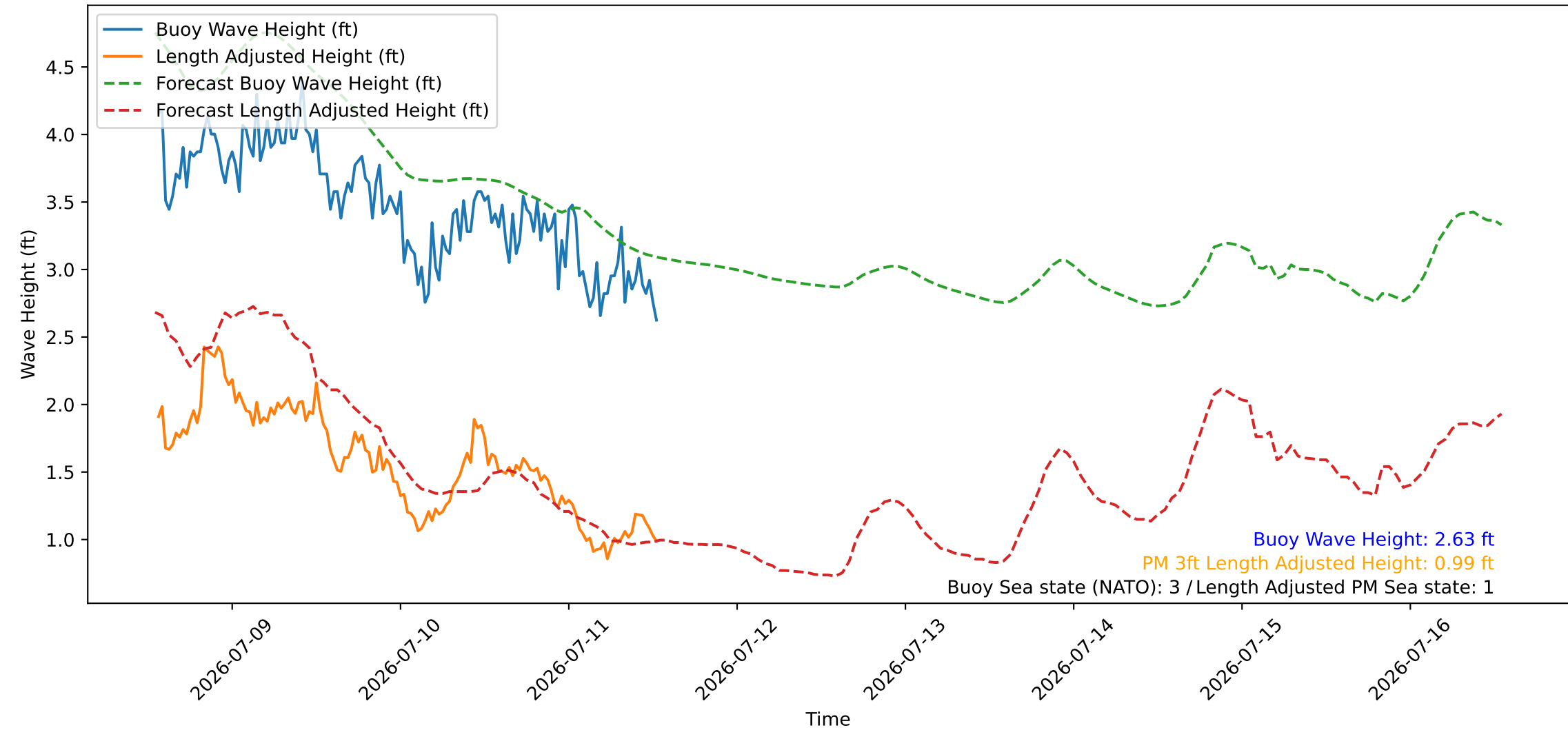
Wave Heights over Time for Green Beach at 2026-07-11 13:21:09
