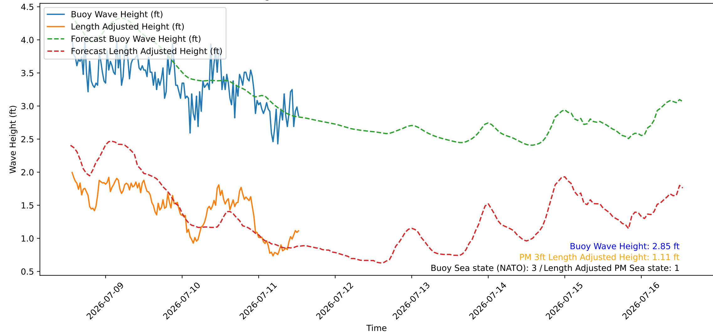
Wave Heights over Time for Red Beach at 2026-07-11 13:20:46
