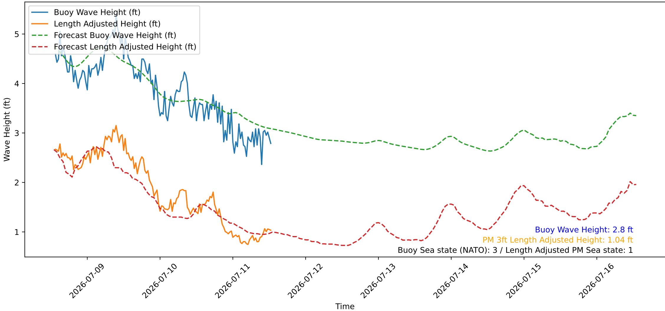
Wave Heights over Time for Oceanside Harbor at 2026-07-11 13:20:25
