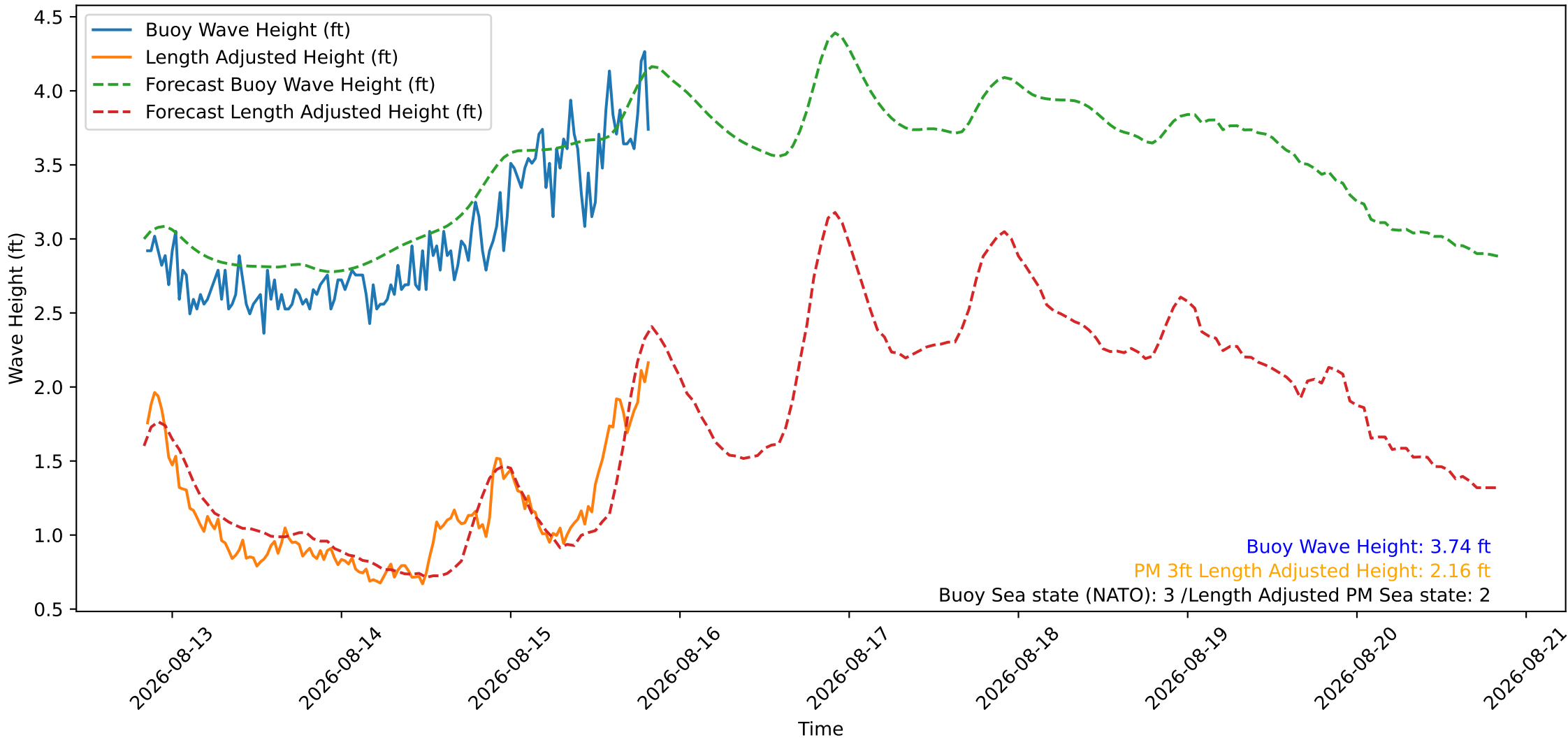
Wave Heights over Time for Green Beach at 2026-08-15 20:21:12
