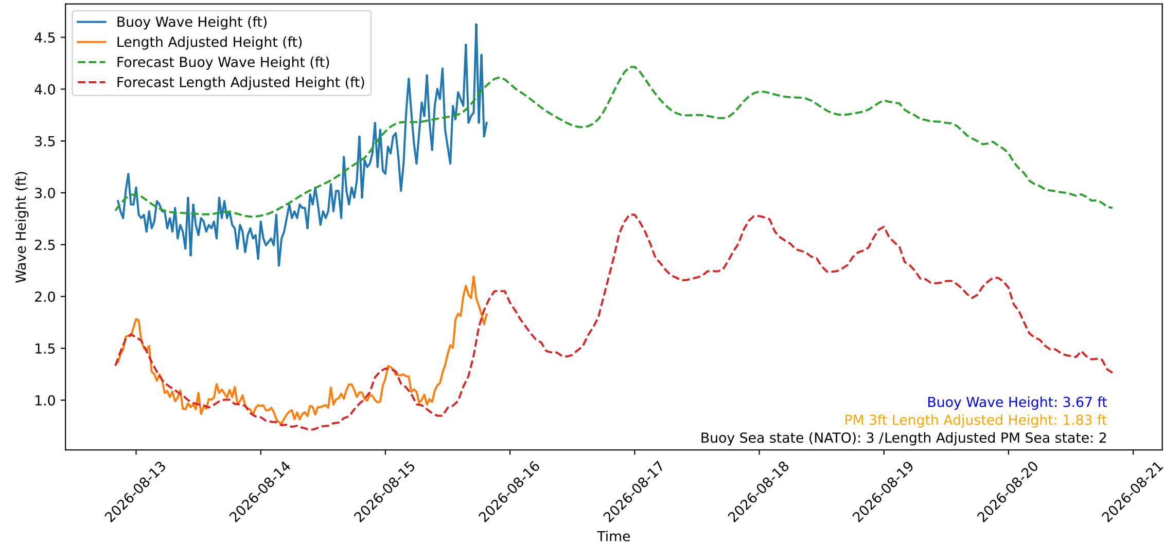
Wave Heights over Time for Oceanside Harbor at 2026-08-15 20:20:26
