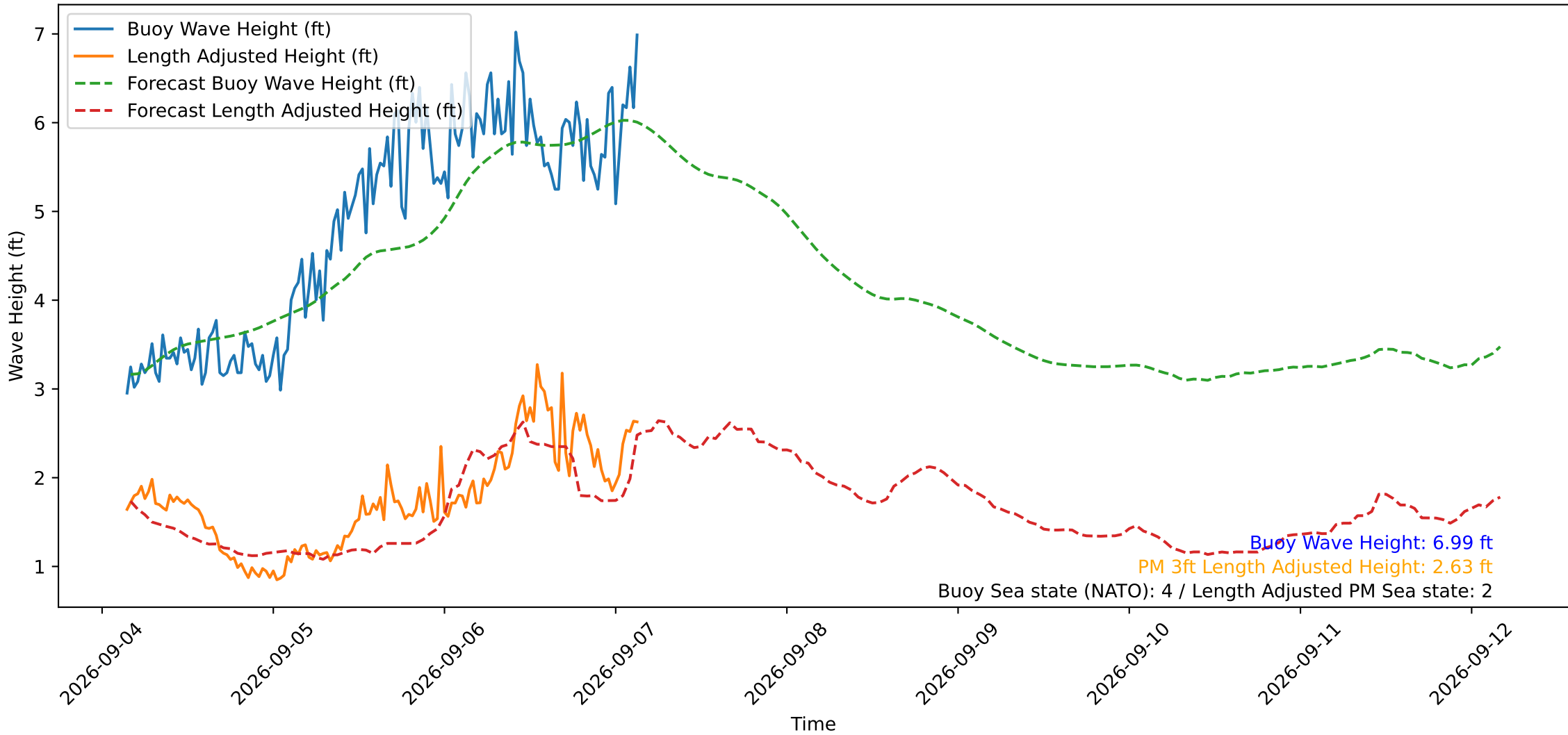
Wave Heights over Time for Oceanside Harbor at 2026-09-07 03:40:30
