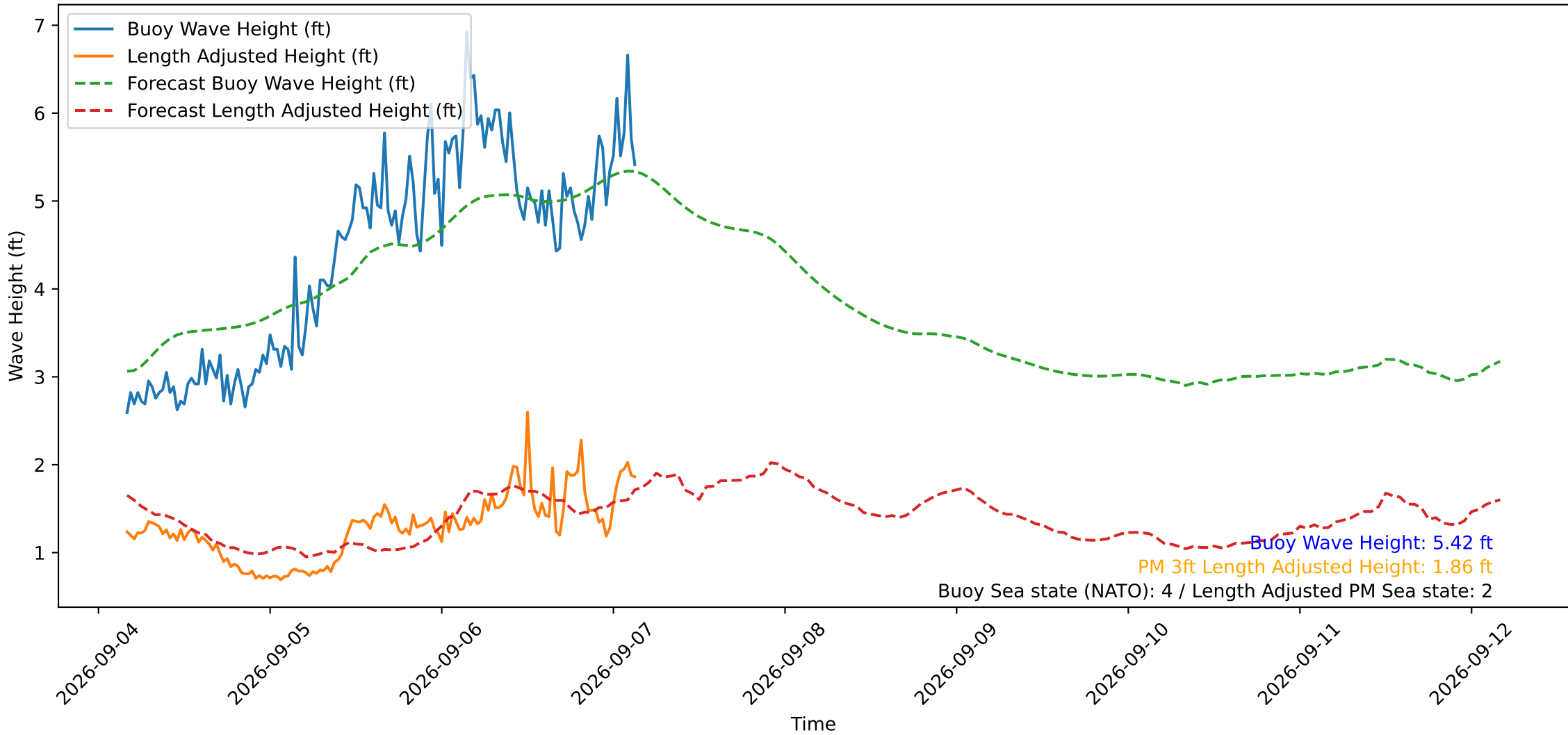
Wave Heights over Time for Red Beach at 2026-09-07 03:40:50
