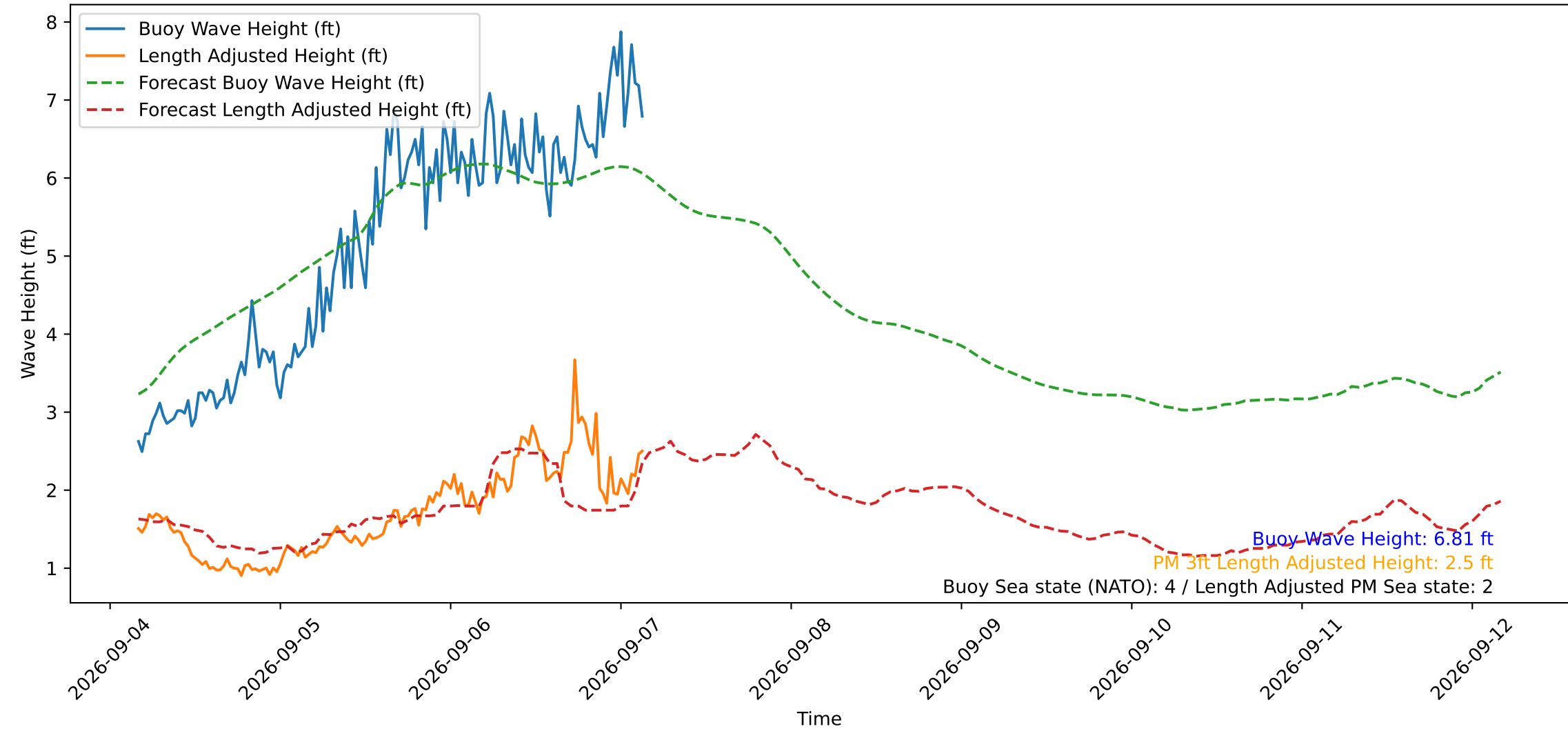
Wave Heights over Time for Green Beach at 2026-09-07 03:41:13
