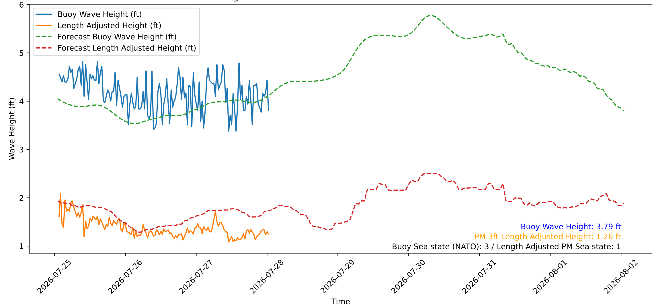
Wave Heights over Time for Green Beach at 2026-07-28 01:21:10
