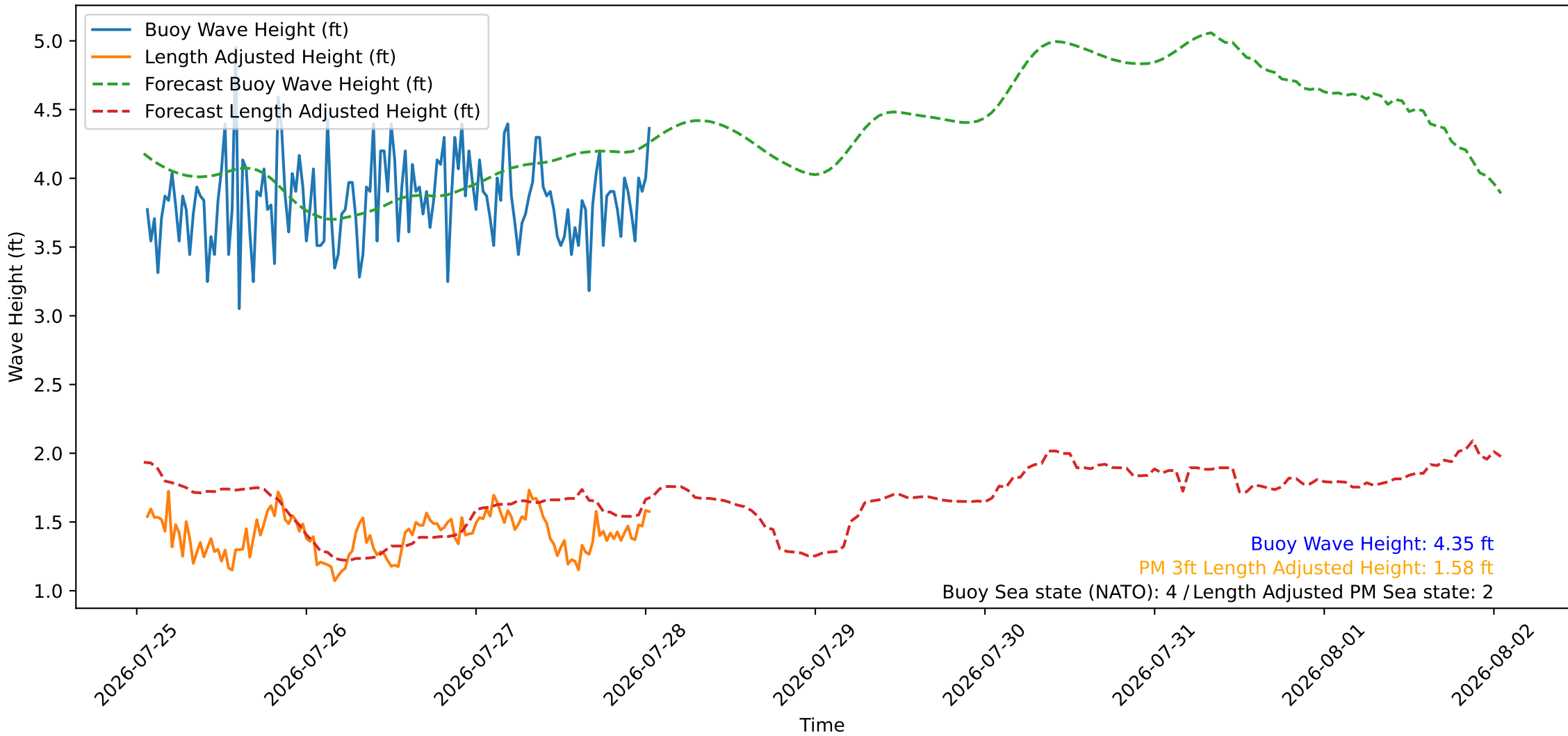
Wave Heights over Time for Oceanside Harbor at 2026-07-28 01:20:26
