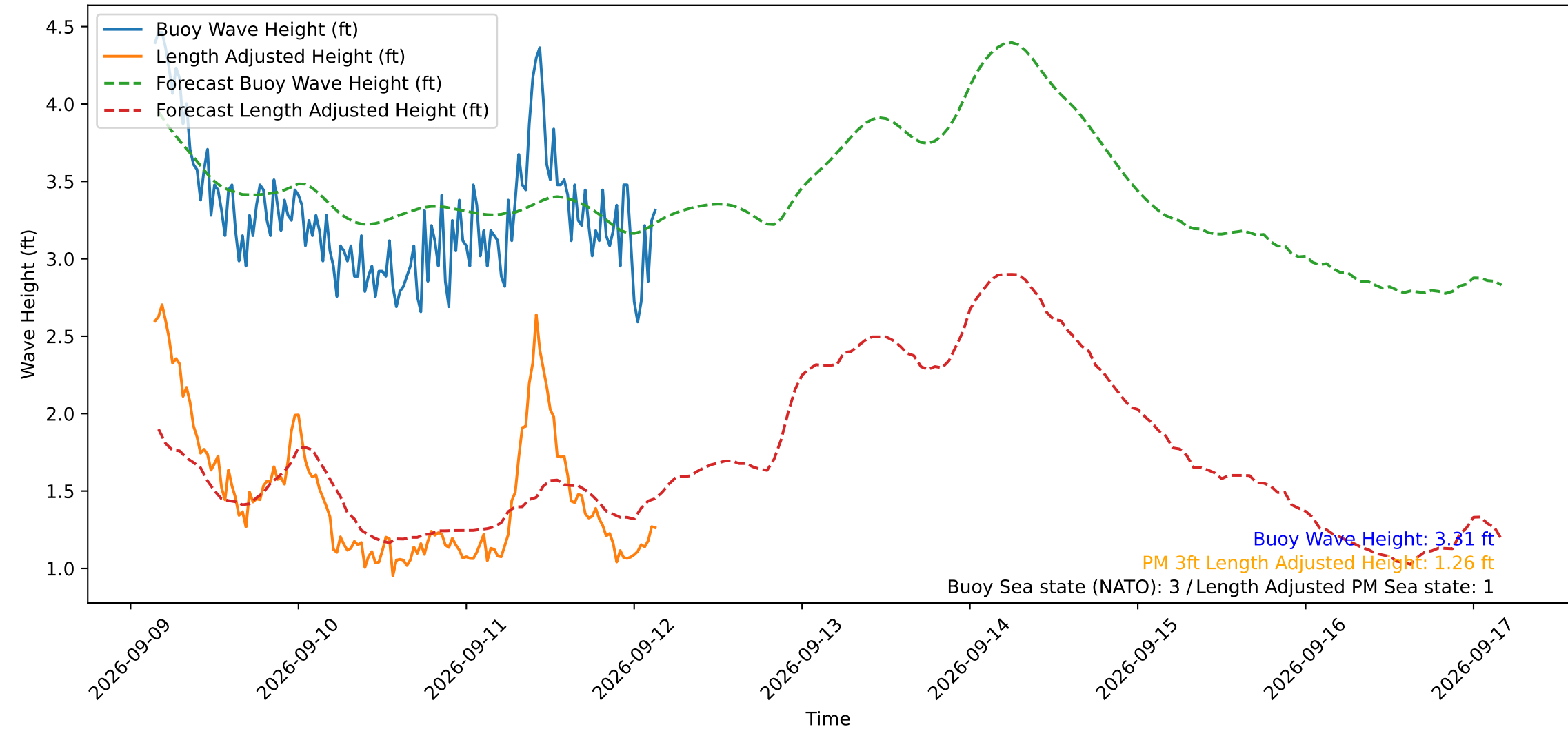
Wave Heights over Time for Oceanside Harbor at 2026-09-12 03:30:30
