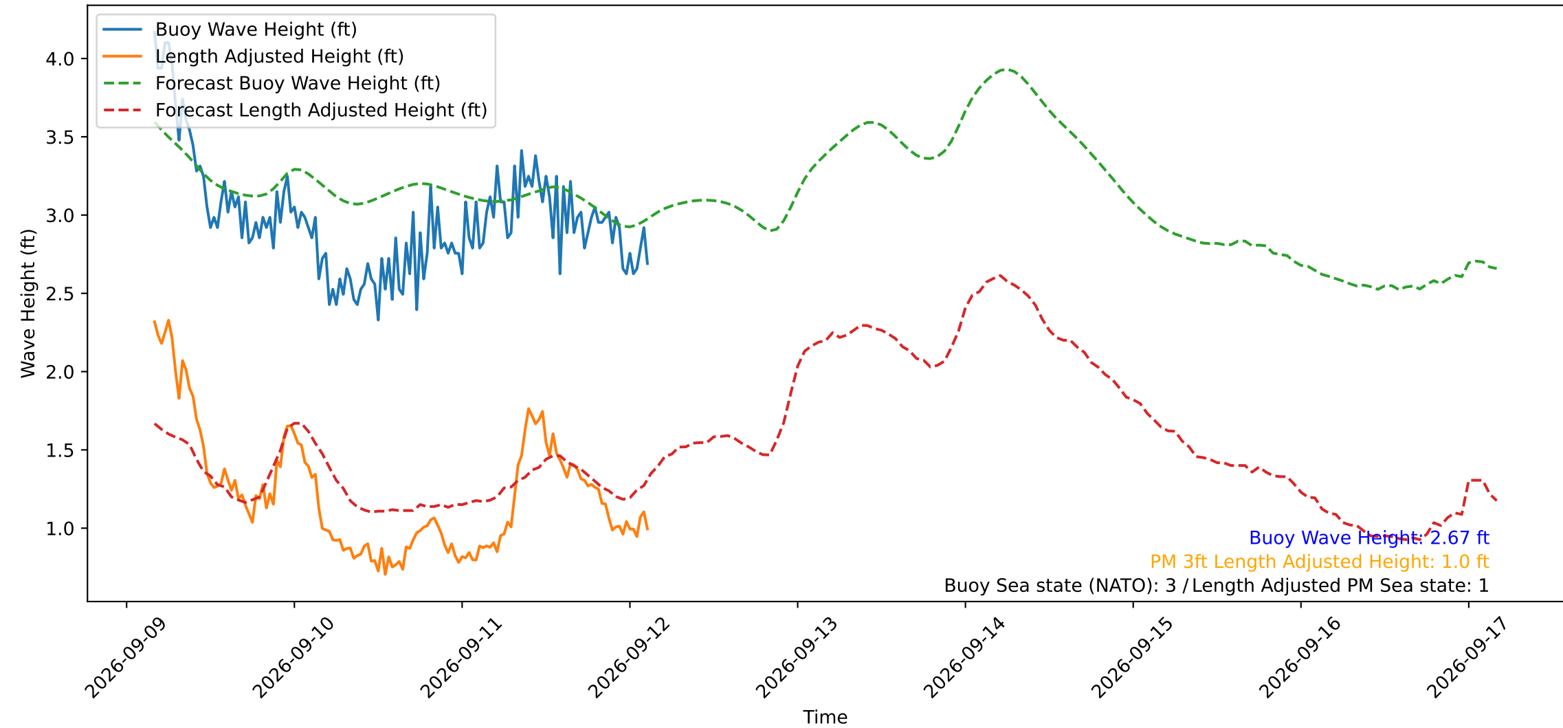
Wave Heights over Time for Red Beach at 2026-09-12 03:30:50
