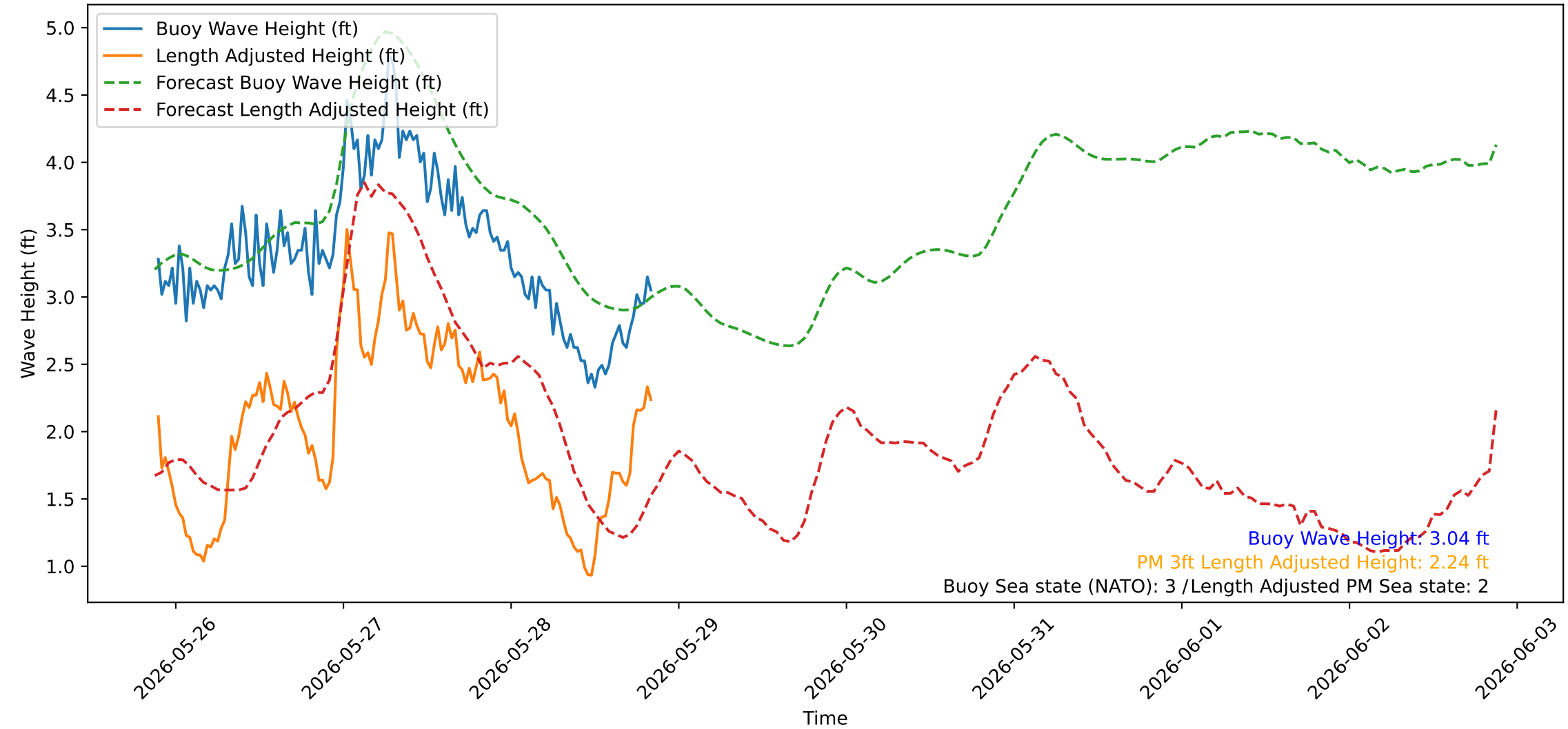
Wave Heights over Time for Red Beach at 2026-05-28 21:00:39
