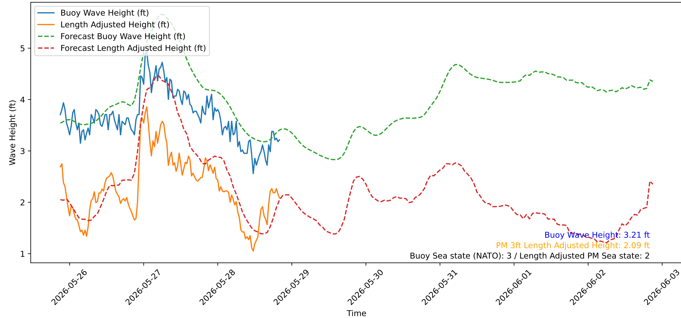
Wave Heights over Time for Green Beach at 2026-05-28 21:01:01
