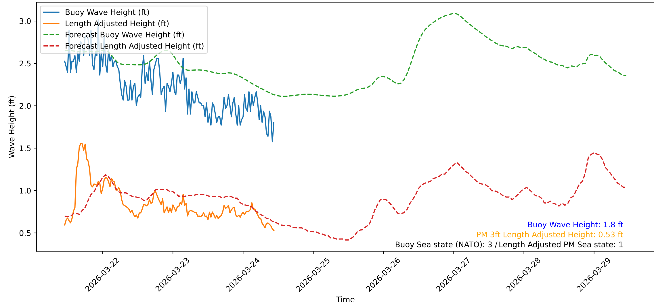
Wave Heights over Time for Oceanside Harbor at 2026-03-24 11:00:31
