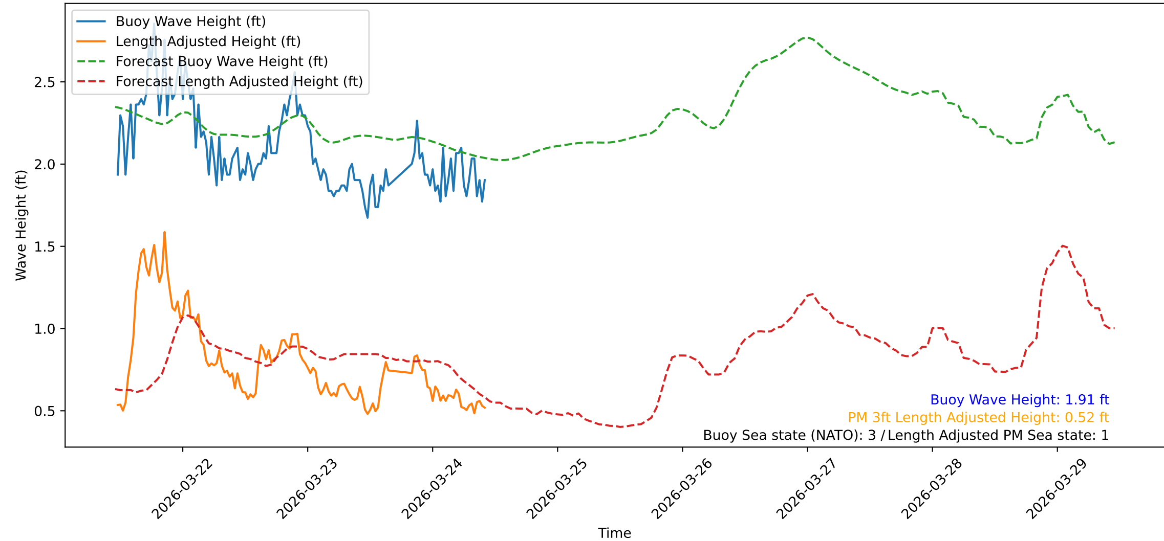
Wave Heights over Time for Red Beach at 2026-03-24 11:00:47
