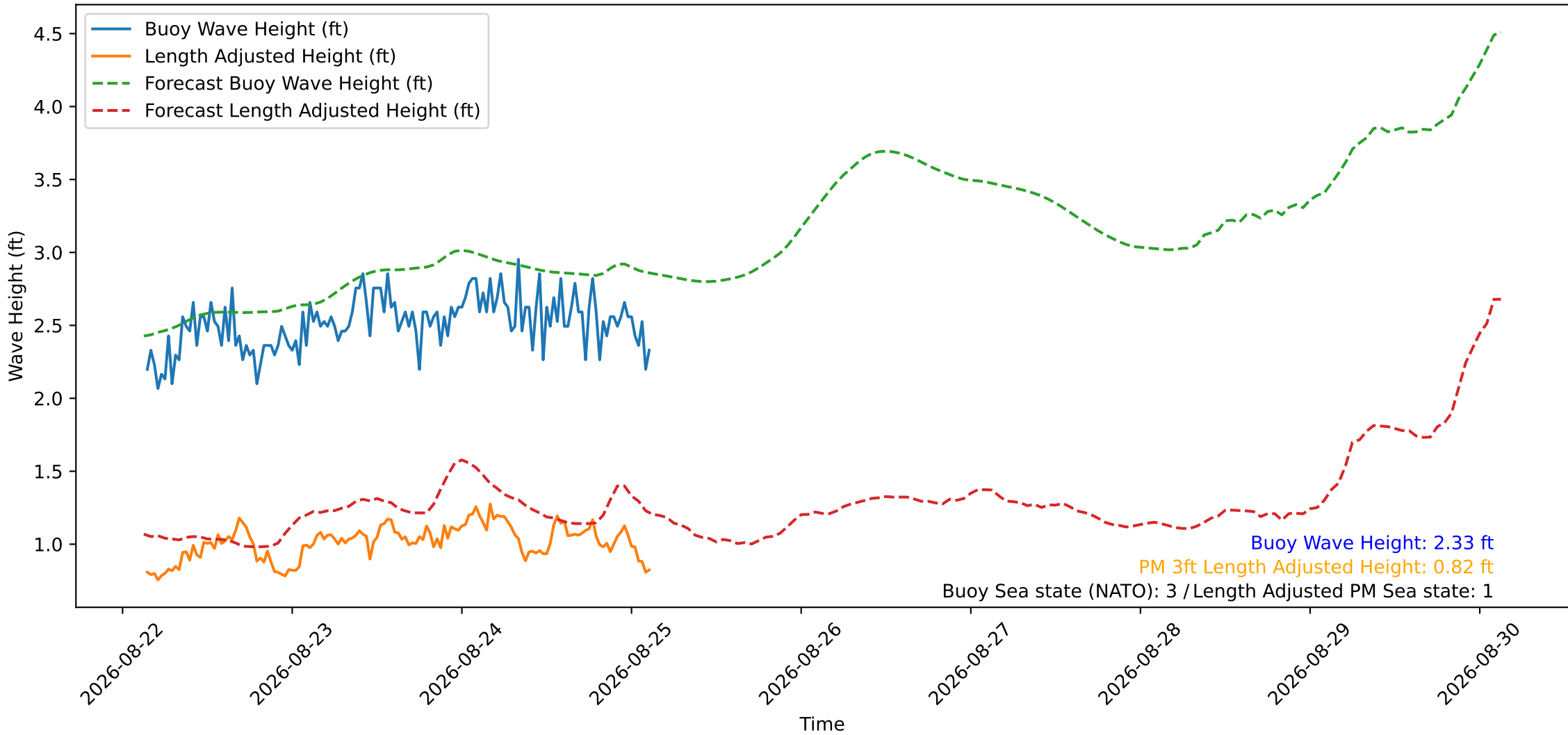
Wave Heights over Time for Red Beach at 2026-08-25 03:10:49
