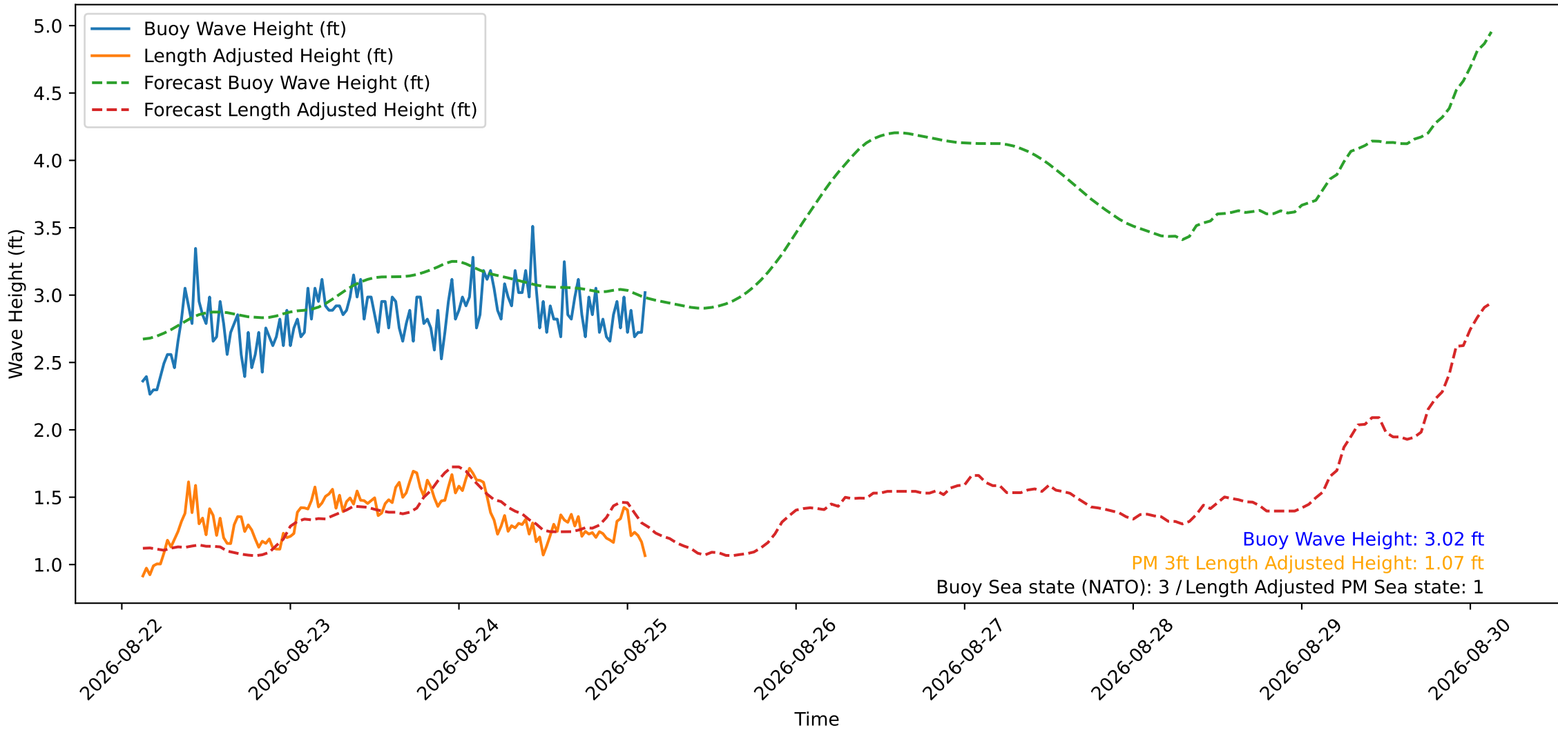
Wave Heights over Time for Oceanside Harbor at 2026-08-25 03:10:29
