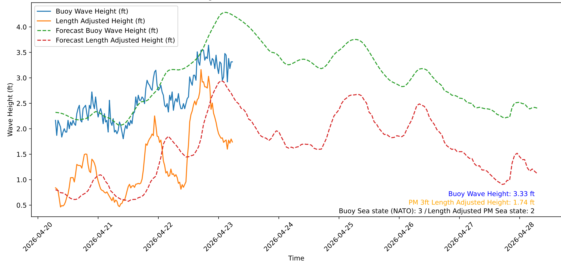
Wave Heights over Time for Red Beach at 2026-04-23 06:40:50
