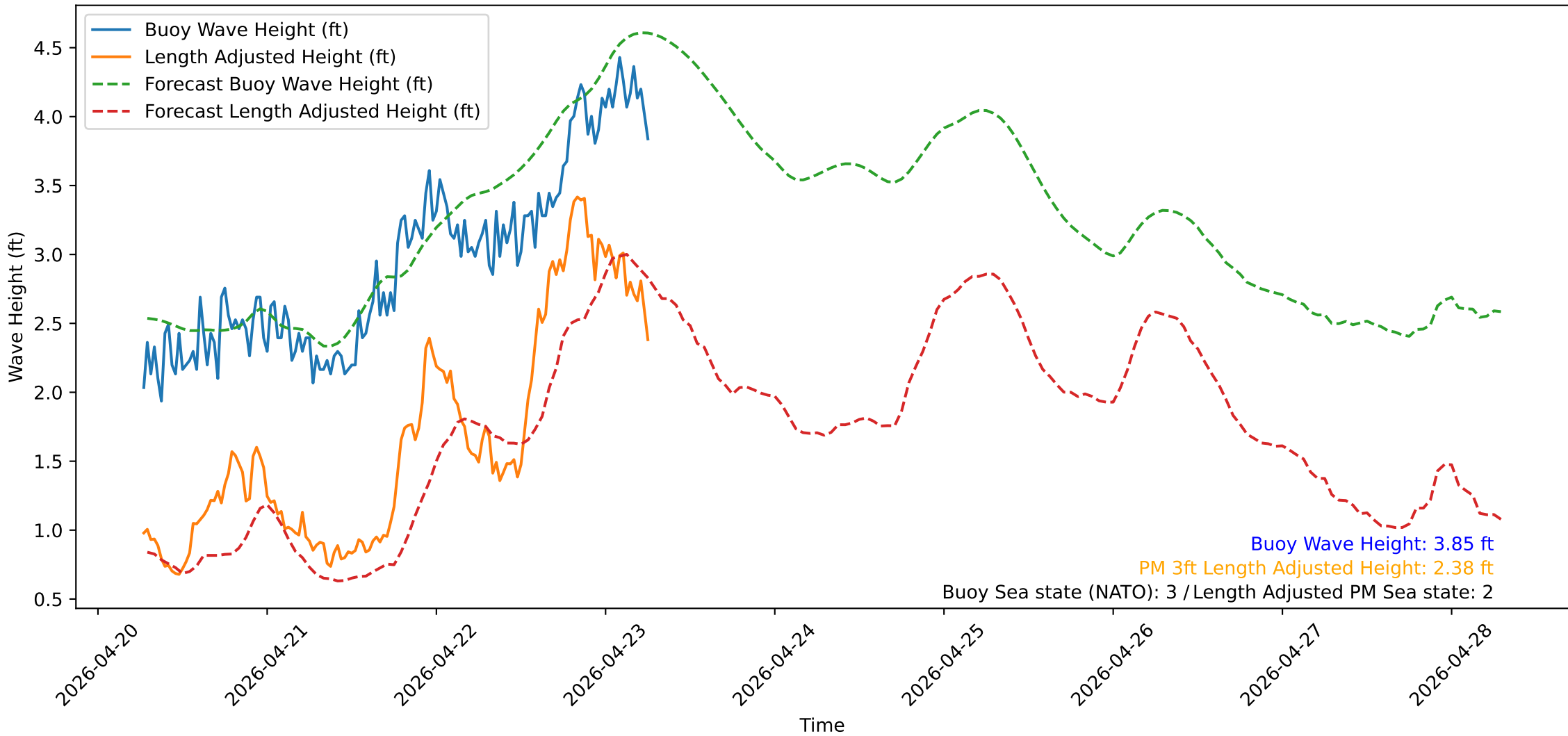
Wave Heights over Time for Oceanside Harbor at 2026-04-23 06:40:31
