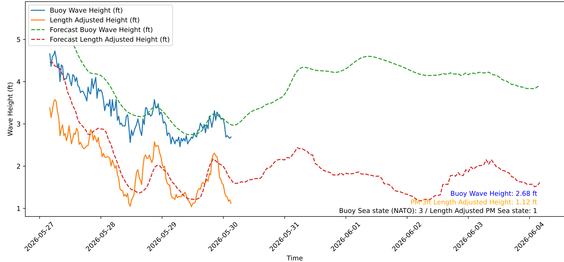
Wave Heights over Time for Green Beach at 2026-05-30 04:01:03
