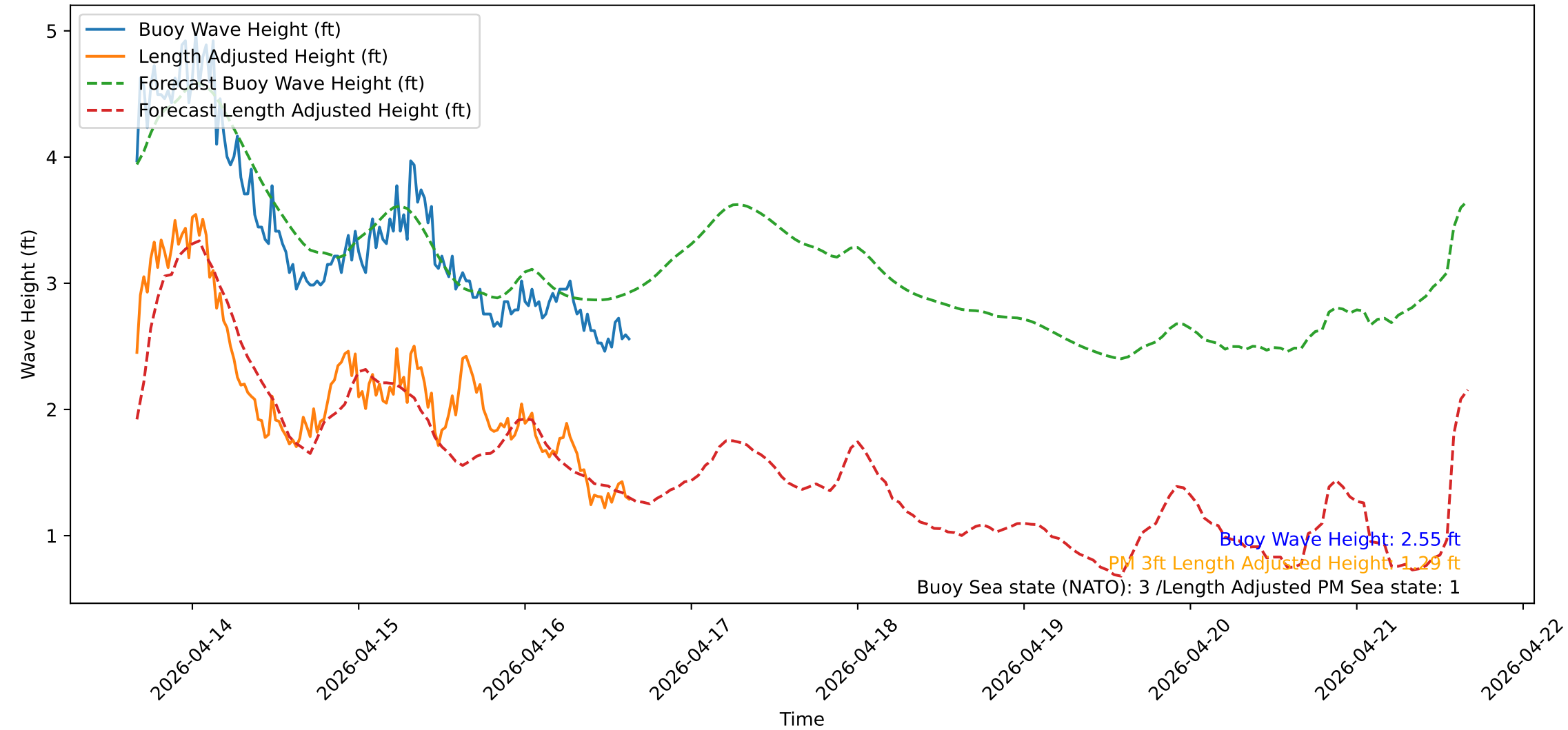
Wave Heights over Time for Green Beach at 2026-04-16 15:51:13
