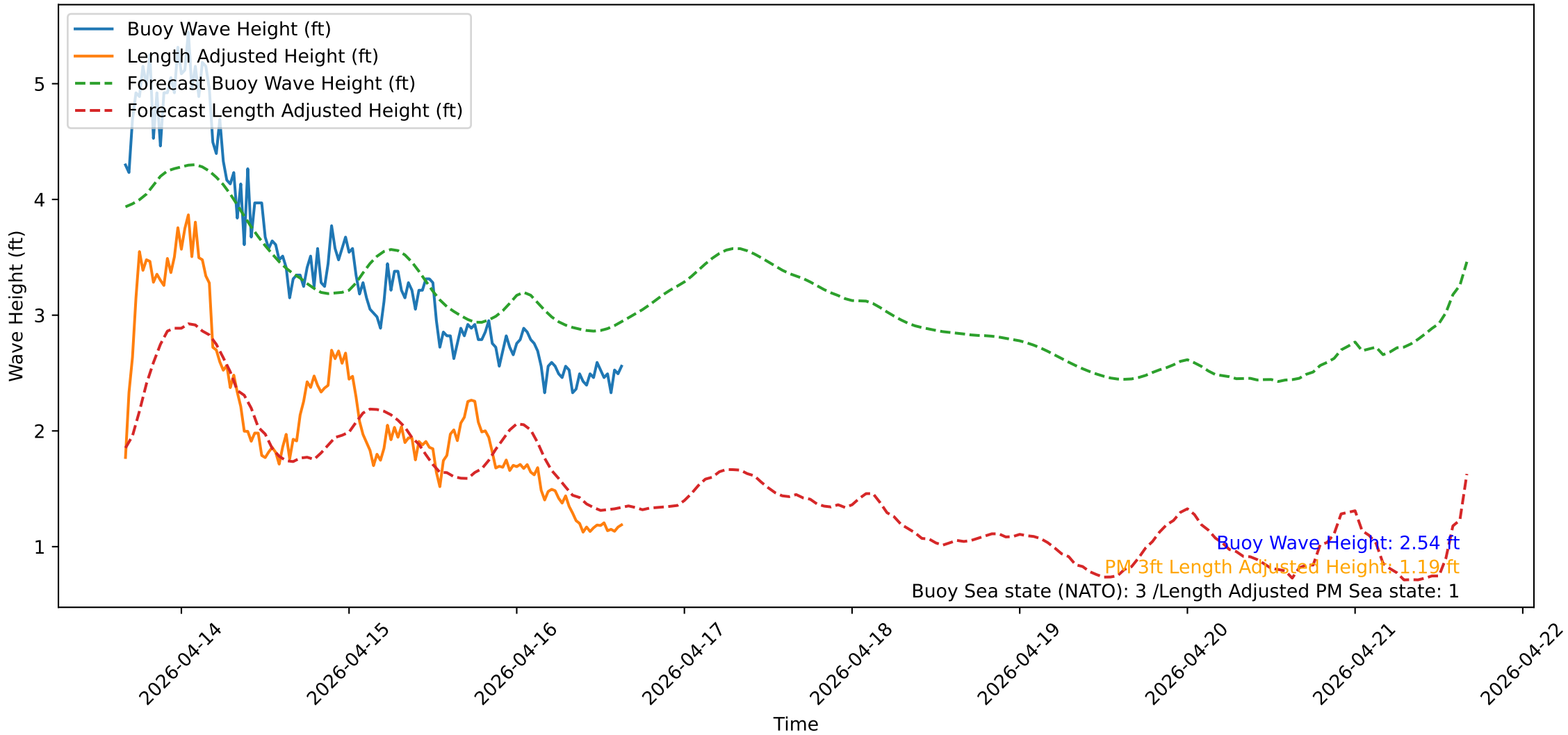
Wave Heights over Time for Oceanside Harbor at 2026-04-16 15:50:31
