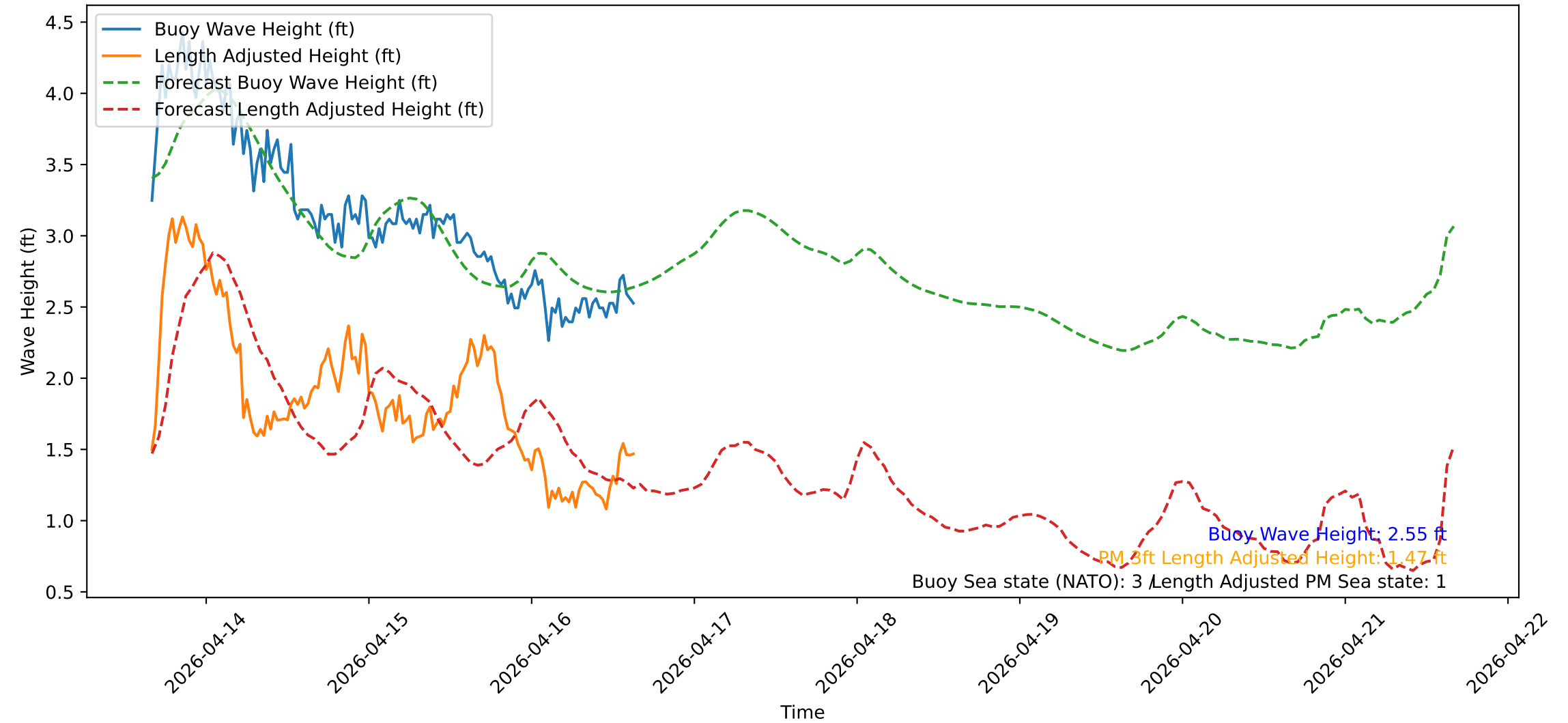
Wave Heights over Time for Red Beach at 2026-04-16 15:50:51
