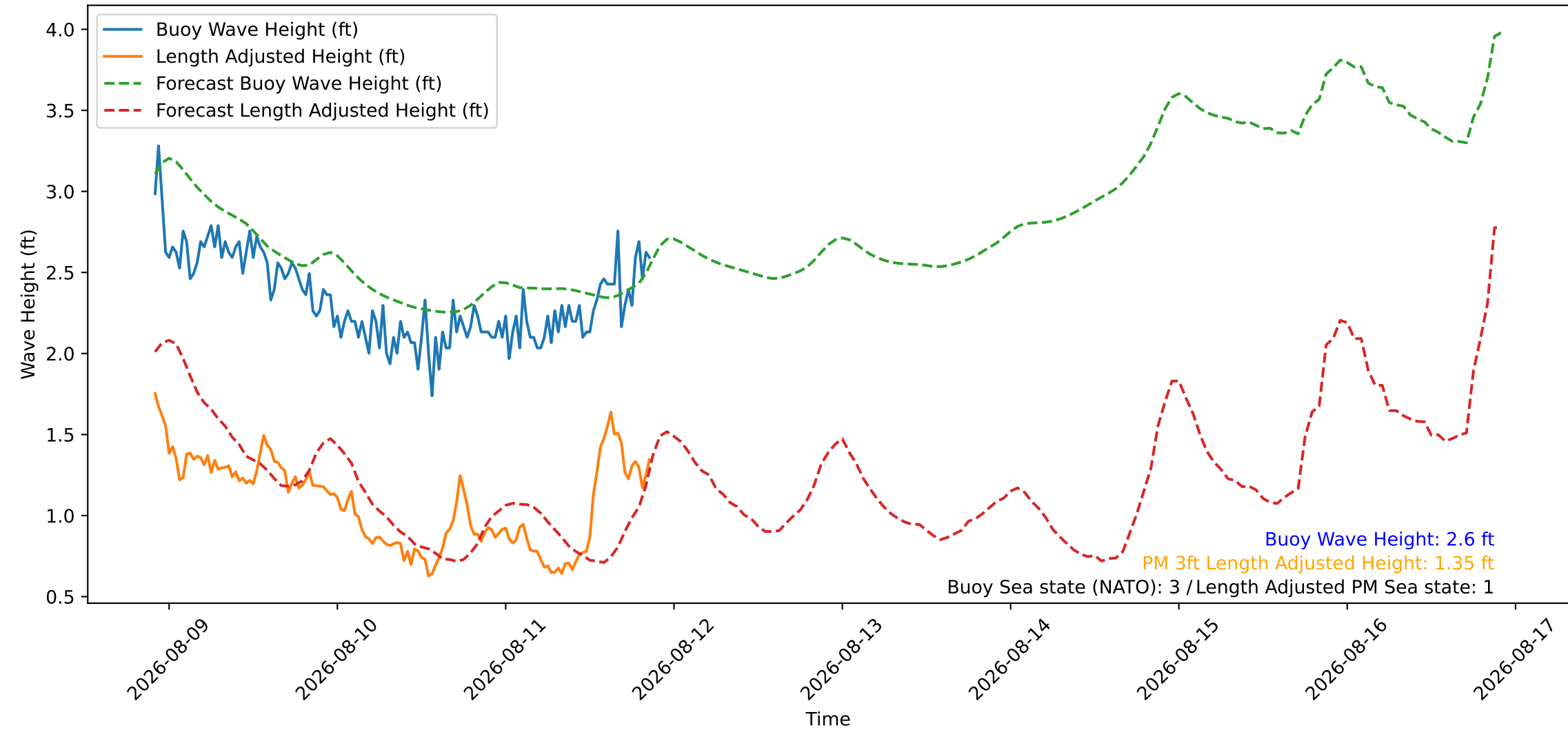
Wave Heights over Time for Red Beach at 2026-08-11 21:30:46
