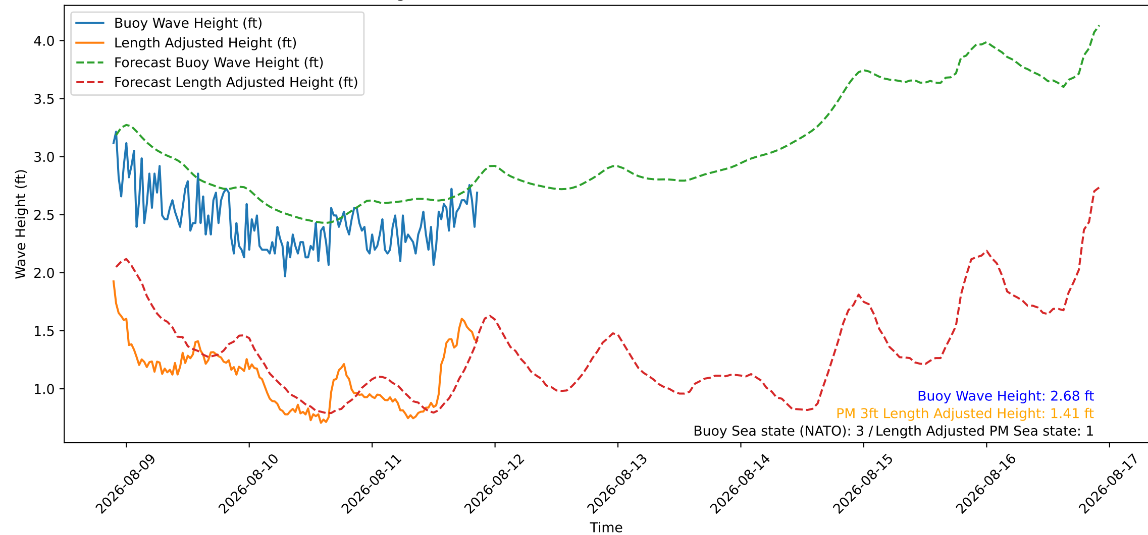
Wave Heights over Time for Oceanside Harbor at 2026-08-11 21:30:26
