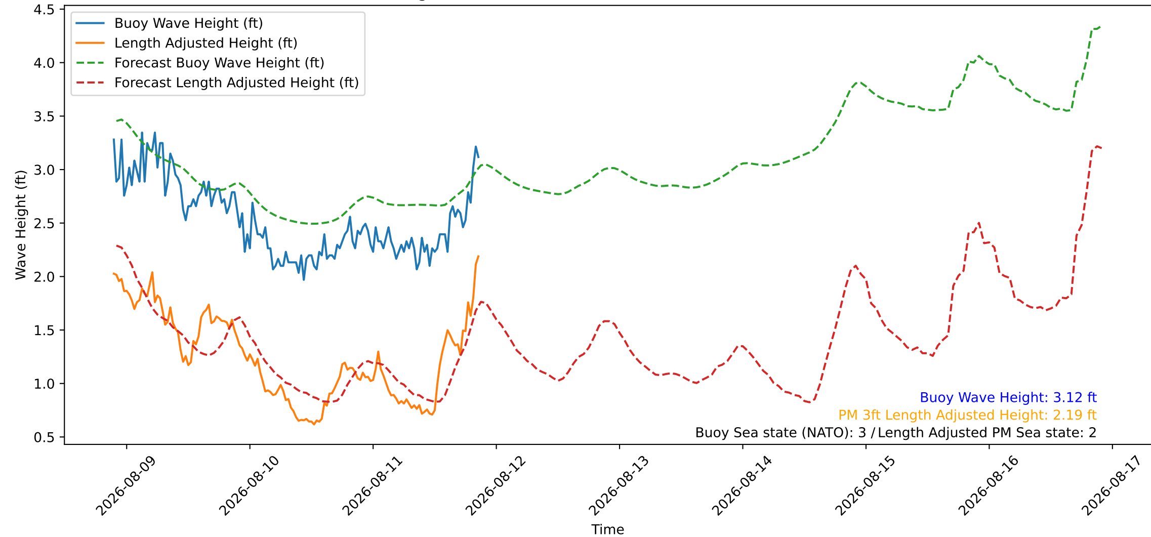
Wave Heights over Time for Green Beach at 2026-08-11 21:31:08
