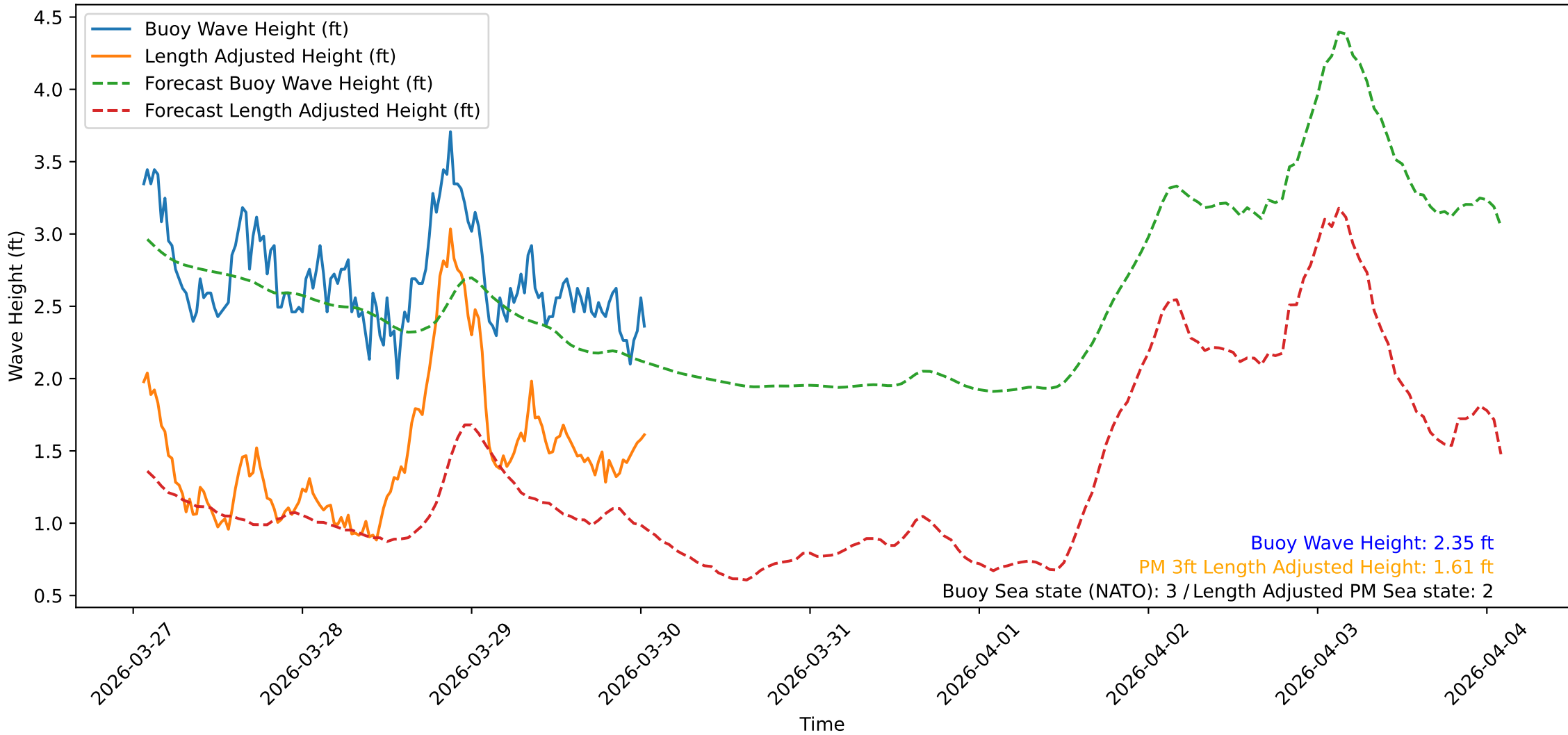
Wave Heights over Time for Green Beach at 2026-03-30 01:31:11
