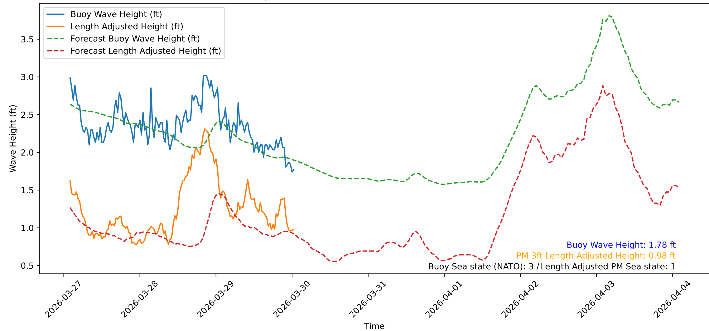
Wave Heights over Time for Red Beach at 2026-03-30 01:30:48
