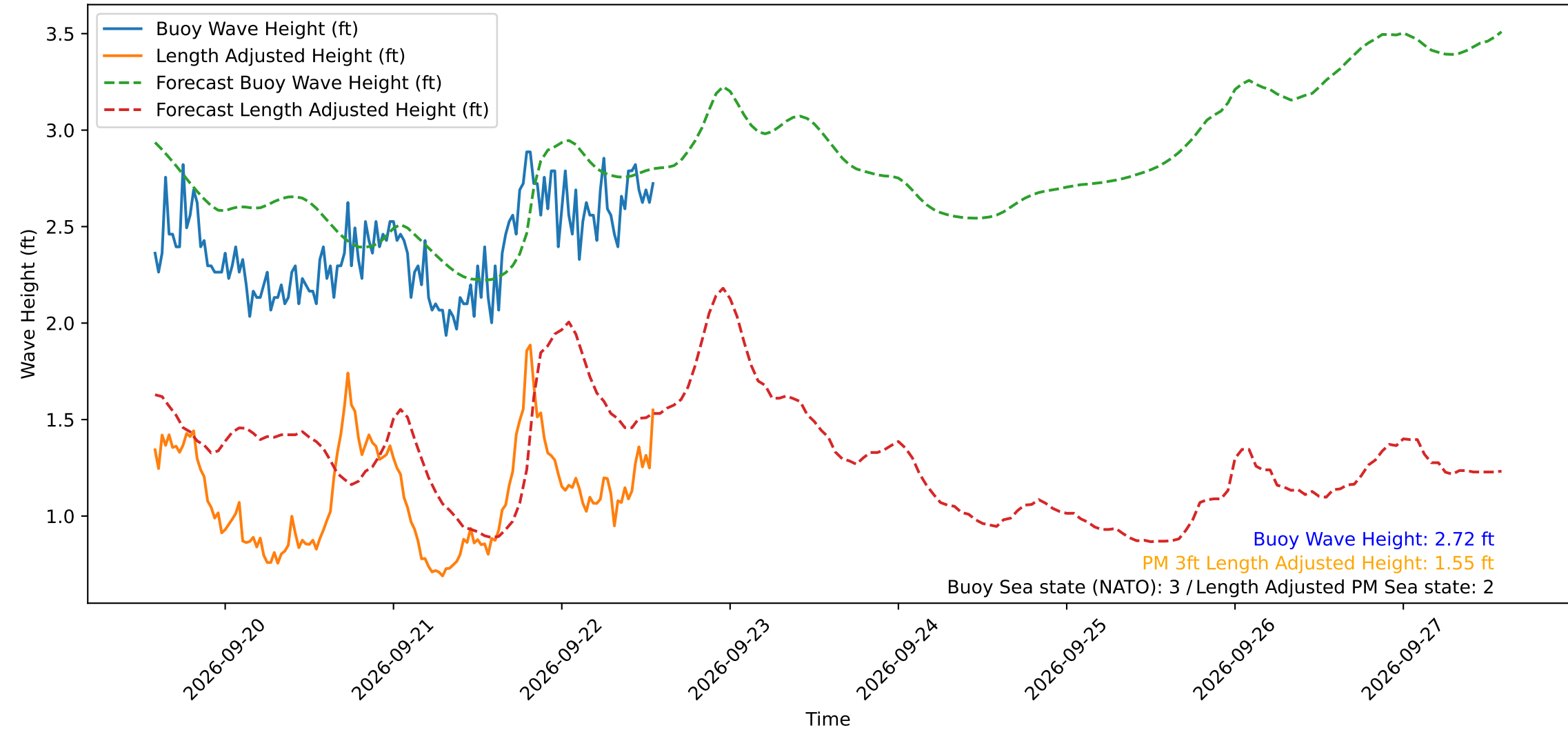
Wave Heights over Time for Red Beach at 2026-09-22 13:50:50
