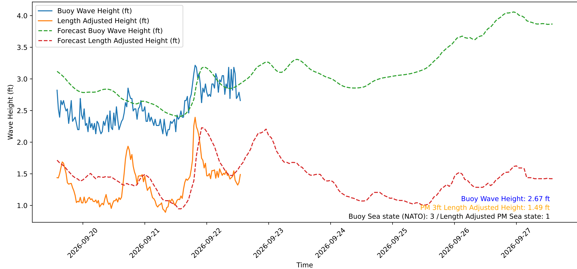
Wave Heights over Time for Oceanside Harbor at 2026-09-22 13:50:29
