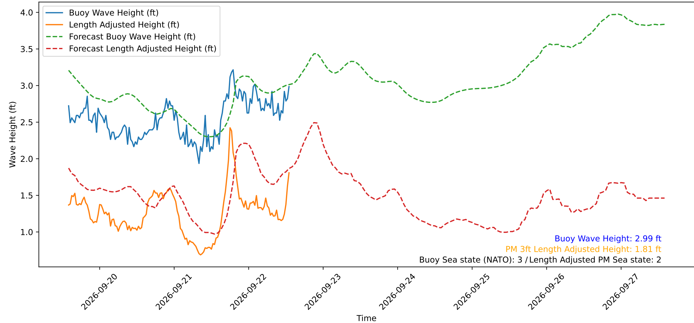
Wave Heights over Time for Green Beach at 2026-09-22 13:51:13
