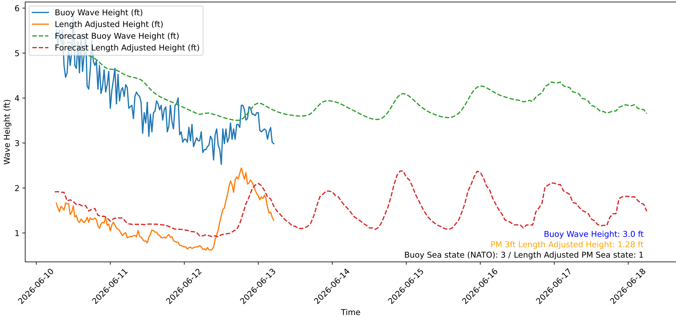
Wave Heights over Time for Red Beach at 2026-06-13 06:00:45
