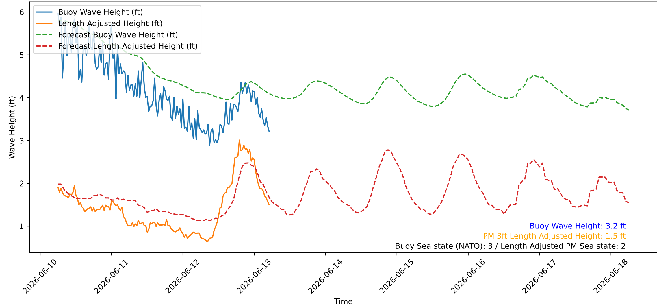
Wave Heights over Time for Green Beach at 2026-06-13 06:01:08
