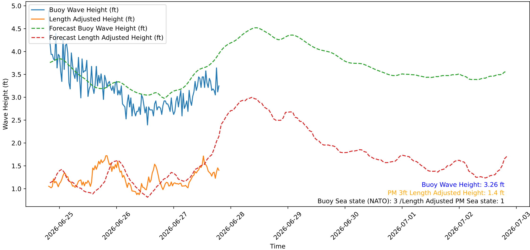
Wave Heights over Time for Oceanside Harbor at 2026-06-27 19:40:26
