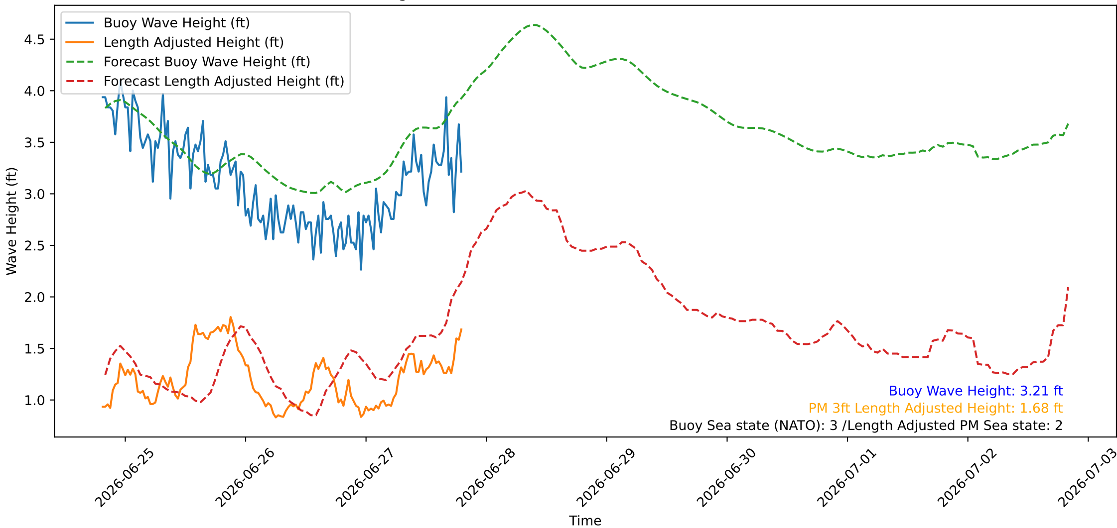
Wave Heights over Time for Green Beach at 2026-06-27 19:41:08
