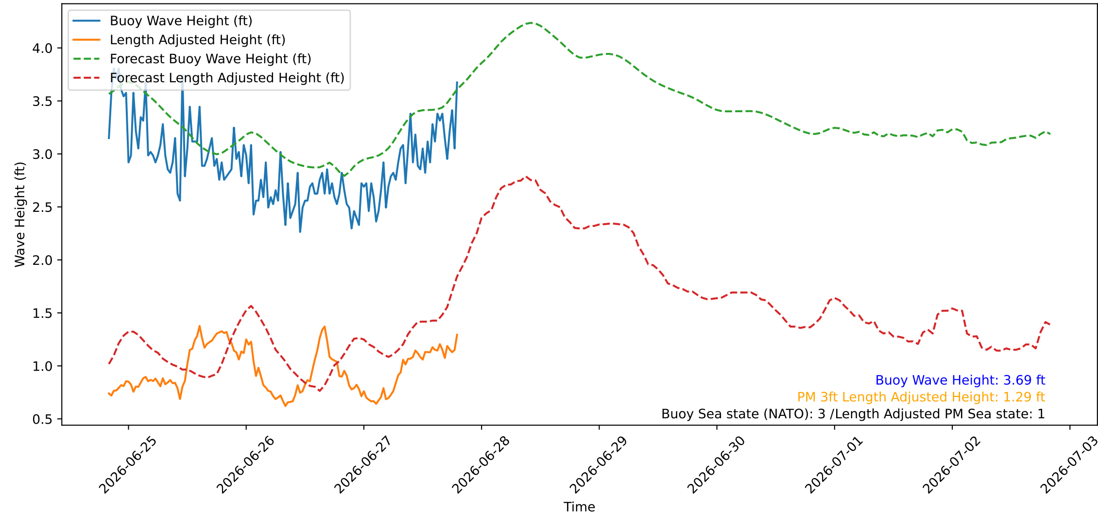
Wave Heights over Time for Red Beach at 2026-06-27 19:40:45
