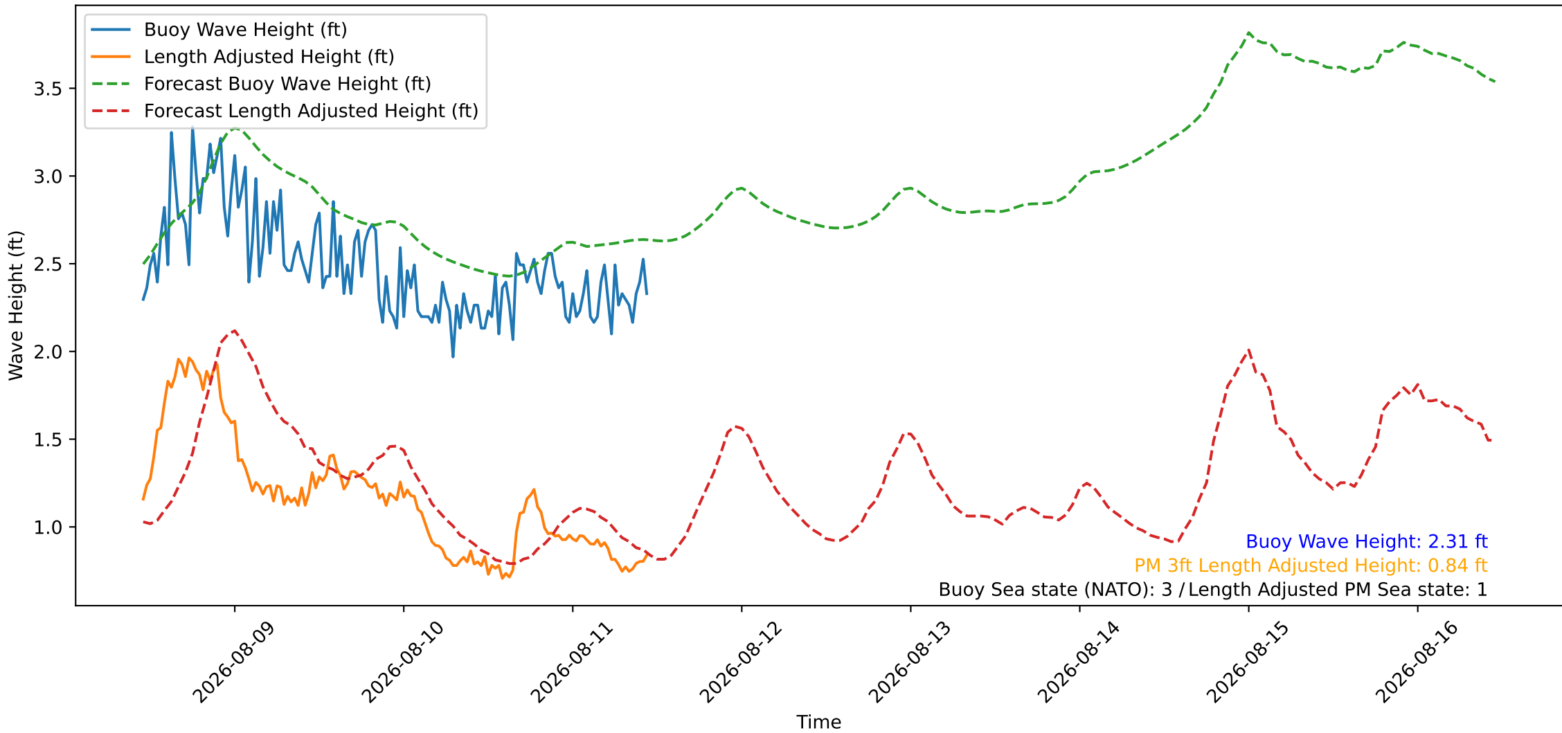
Wave Heights over Time for Oceanside Harbor at 2026-08-11 11:10:26
