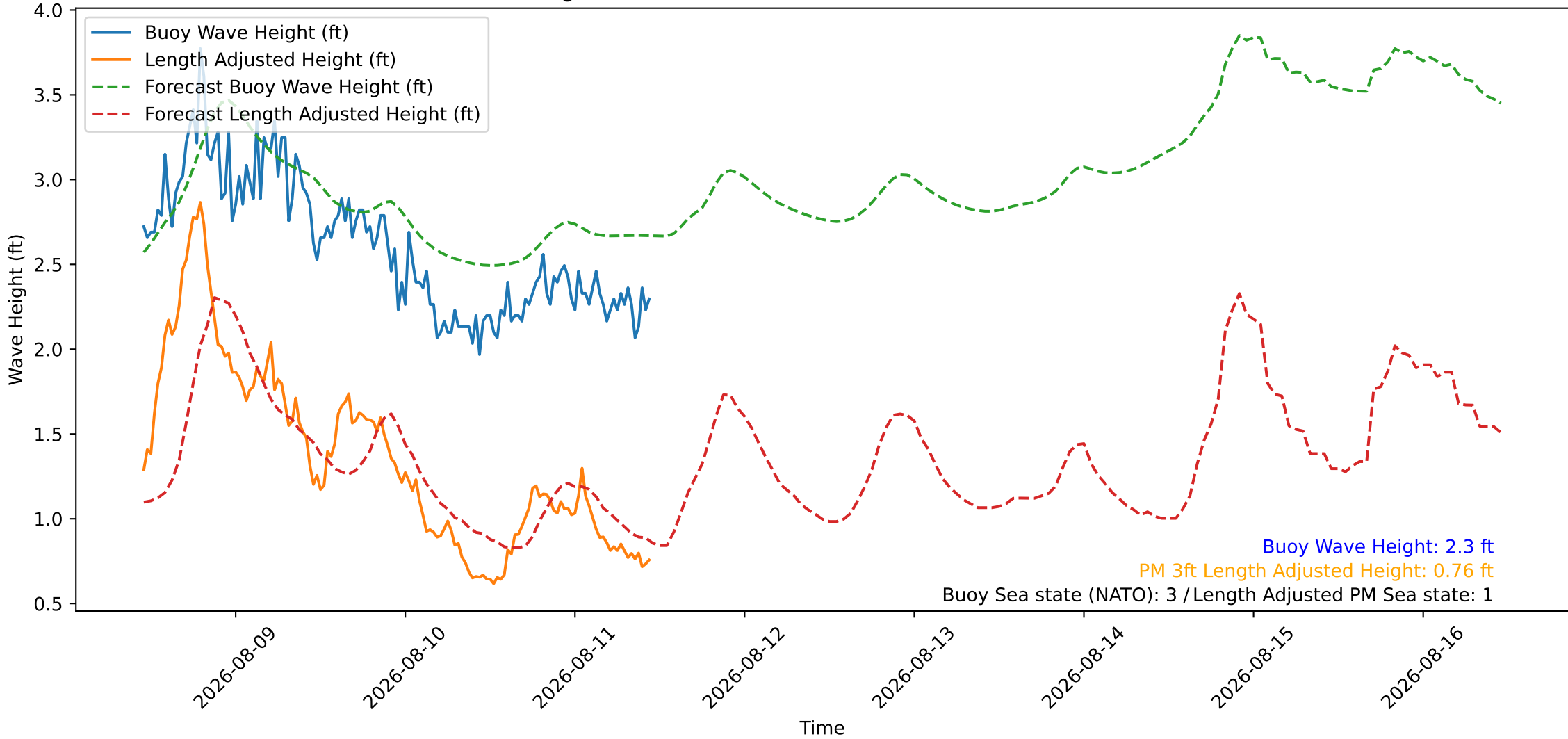
Wave Heights over Time for Green Beach at 2026-08-11 11:11:09
