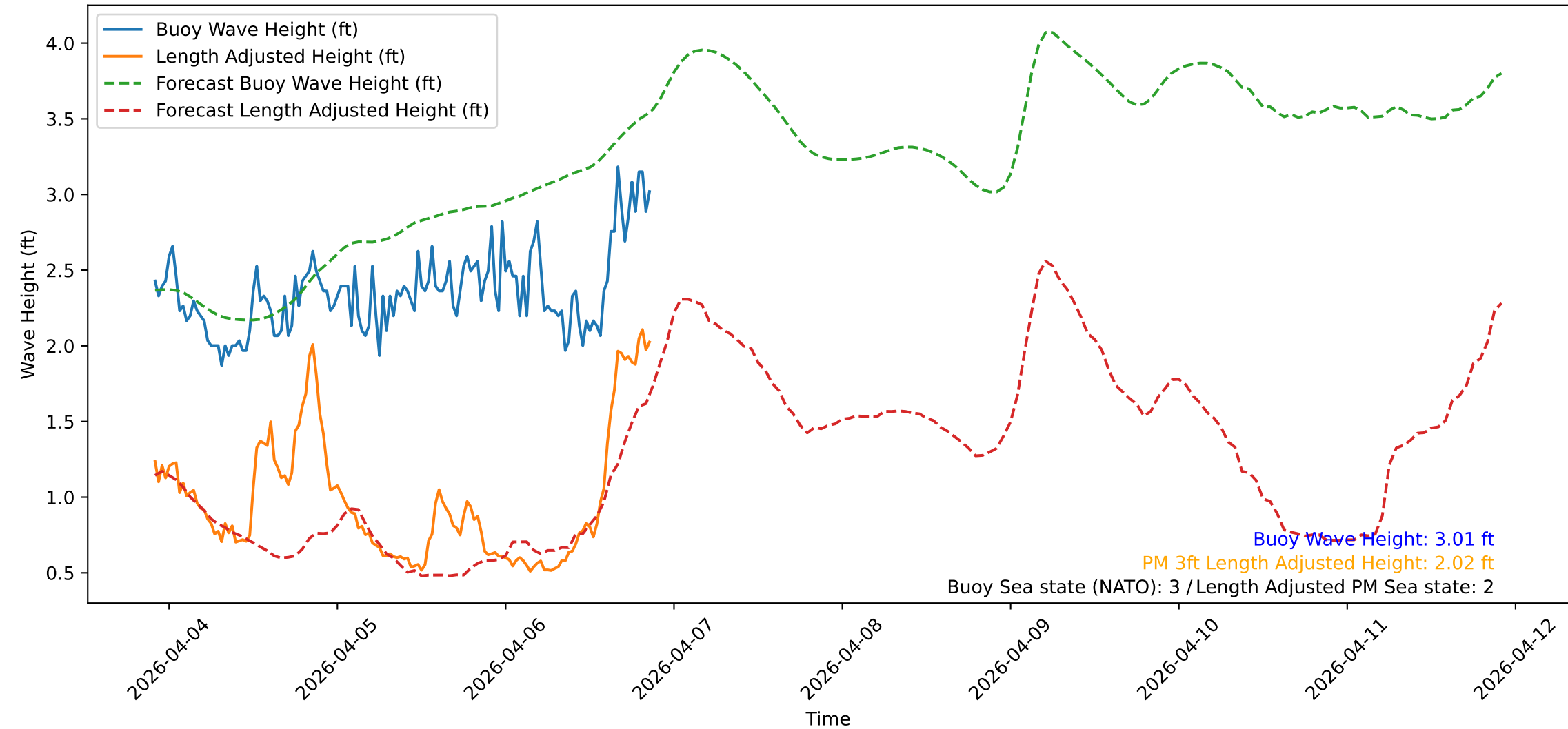
Wave Heights over Time for Red Beach at 2026-04-06 21:30:48
