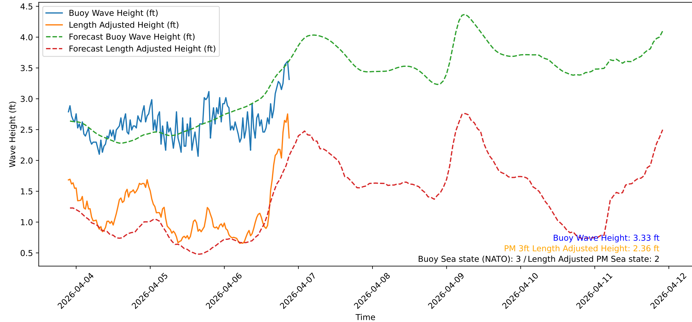
Wave Heights over Time for Oceanside Harbor at 2026-04-06 21:30:33
