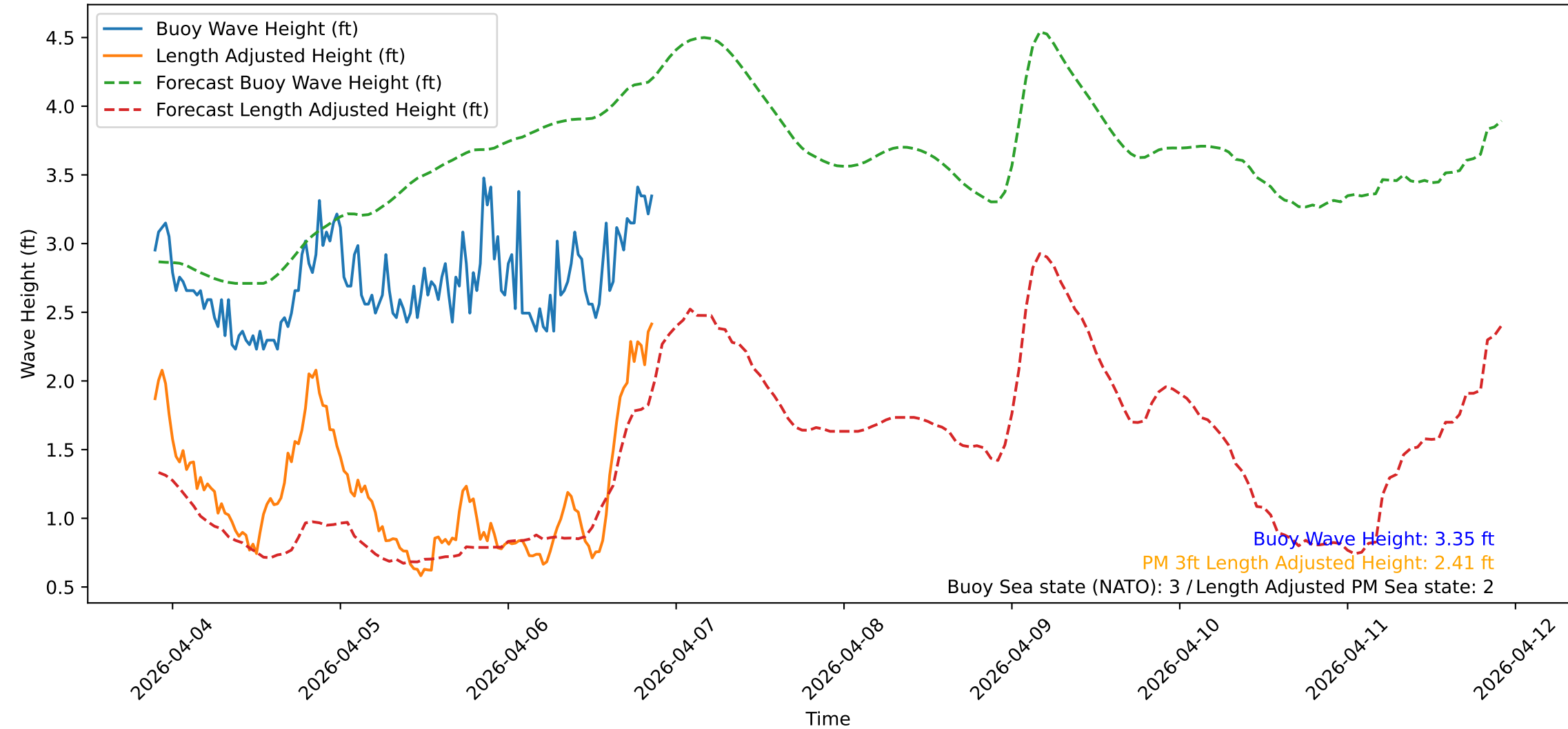
Wave Heights over Time for Green Beach at 2026-04-06 21:31:11
