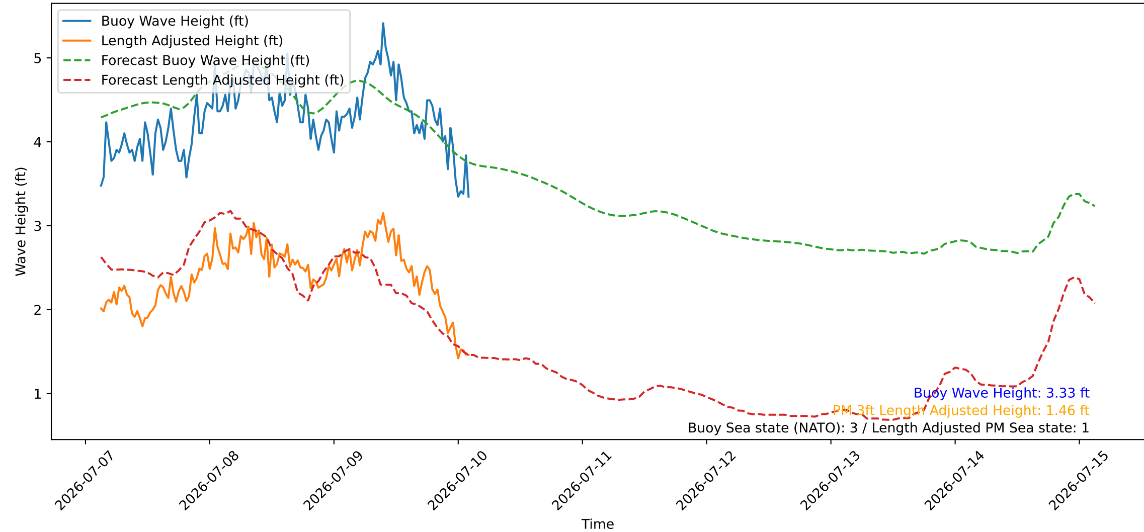
Wave Heights over Time for Oceanside Harbor at 2026-07-10 03:00:26
