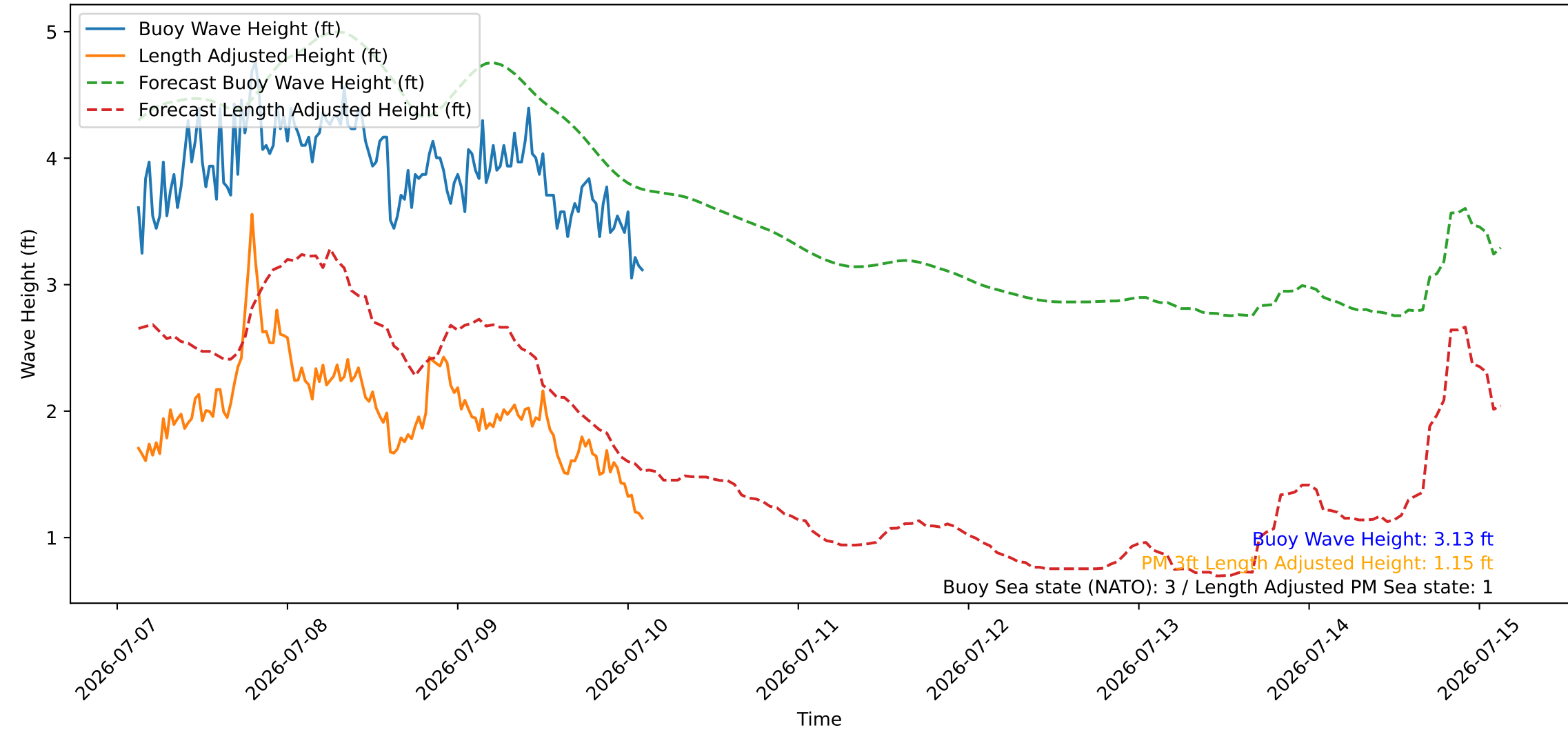
Wave Heights over Time for Green Beach at 2026-07-10 03:01:08
