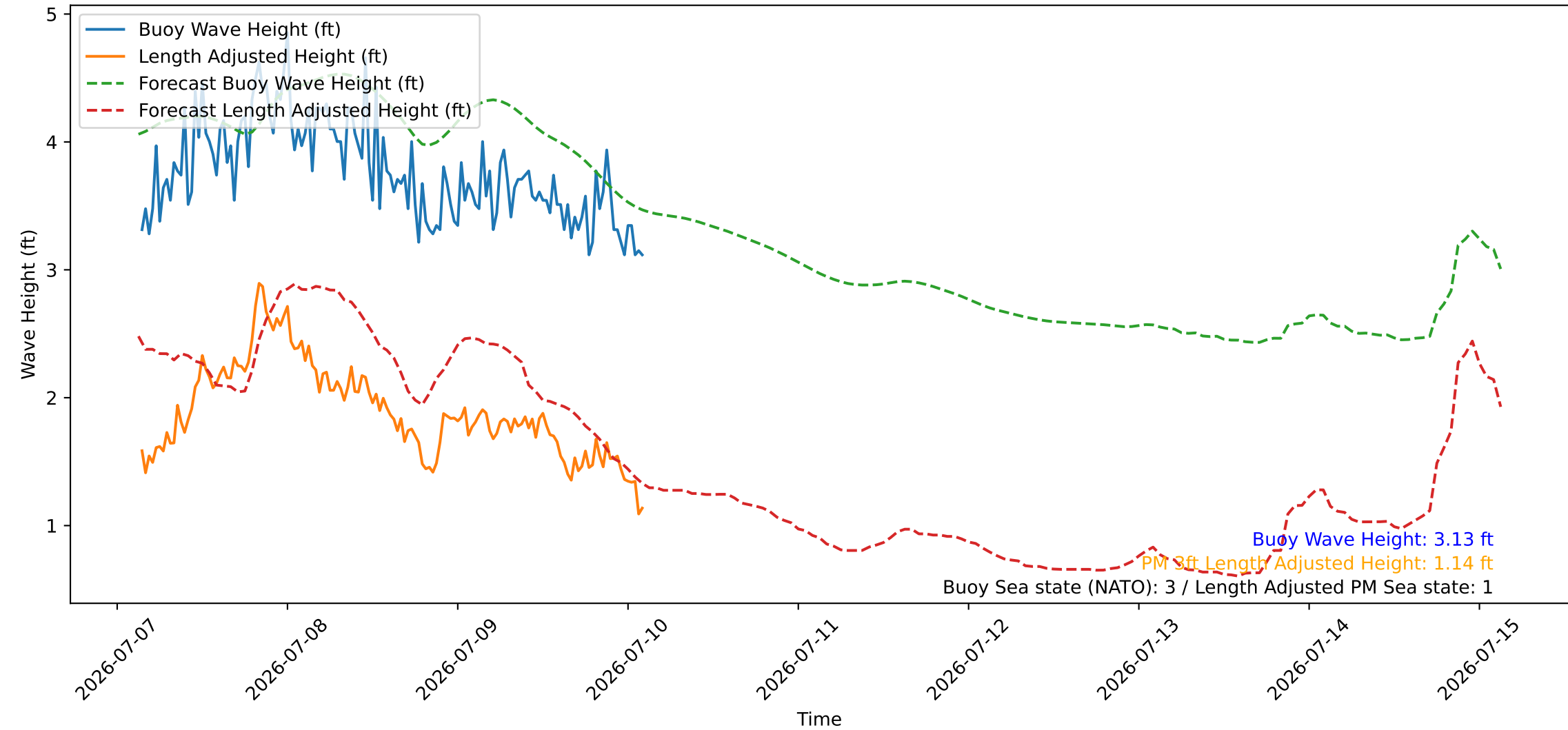
Wave Heights over Time for Red Beach at 2026-07-10 03:00:46
