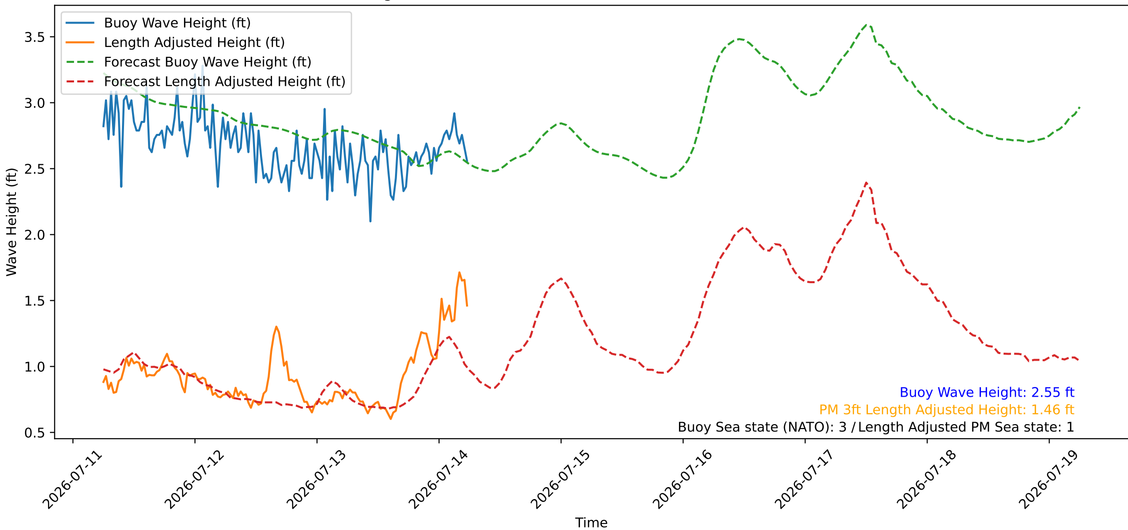
Wave Heights over Time for Oceanside Harbor at 2026-07-14 06:10:26
