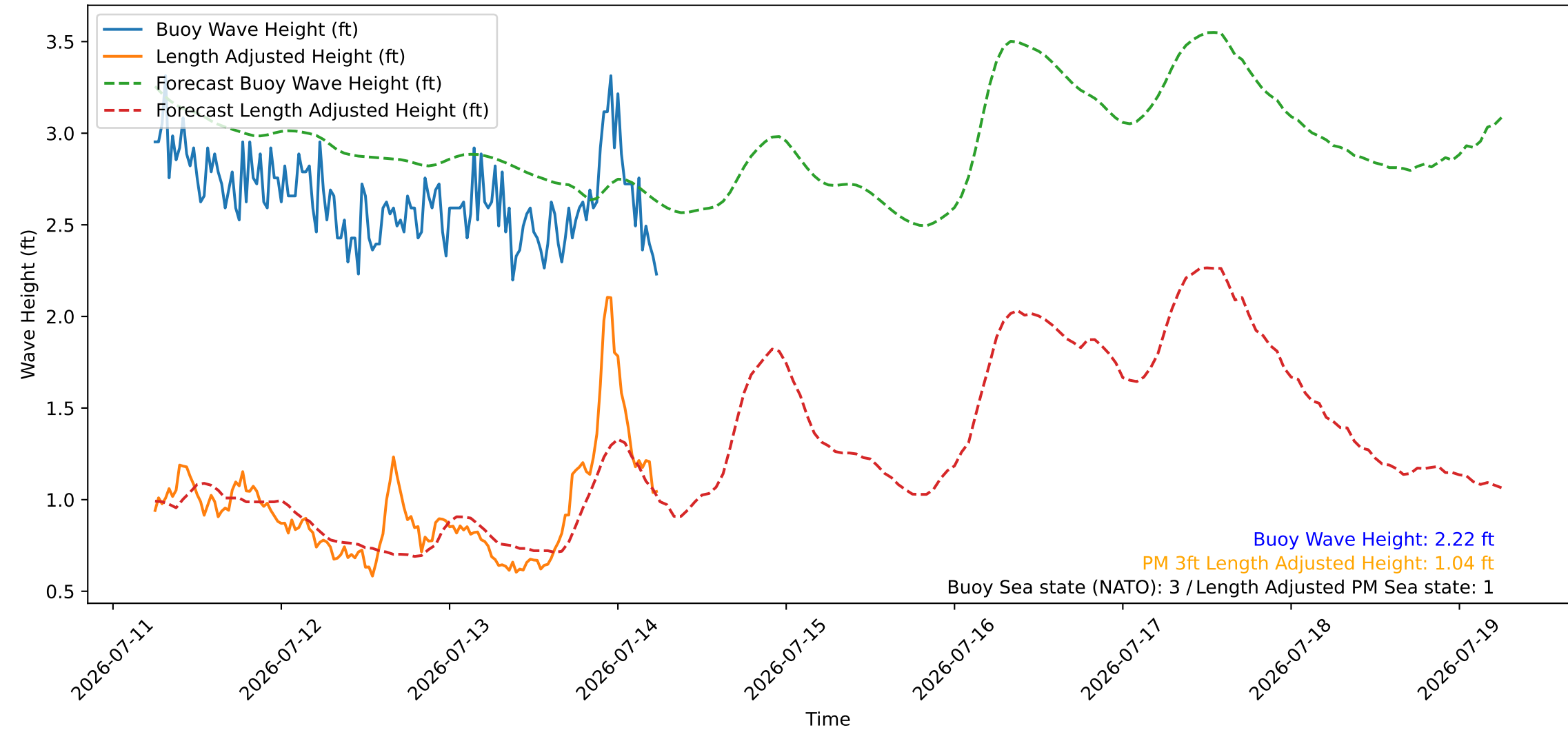
Wave Heights over Time for Green Beach at 2026-07-14 06:11:08
