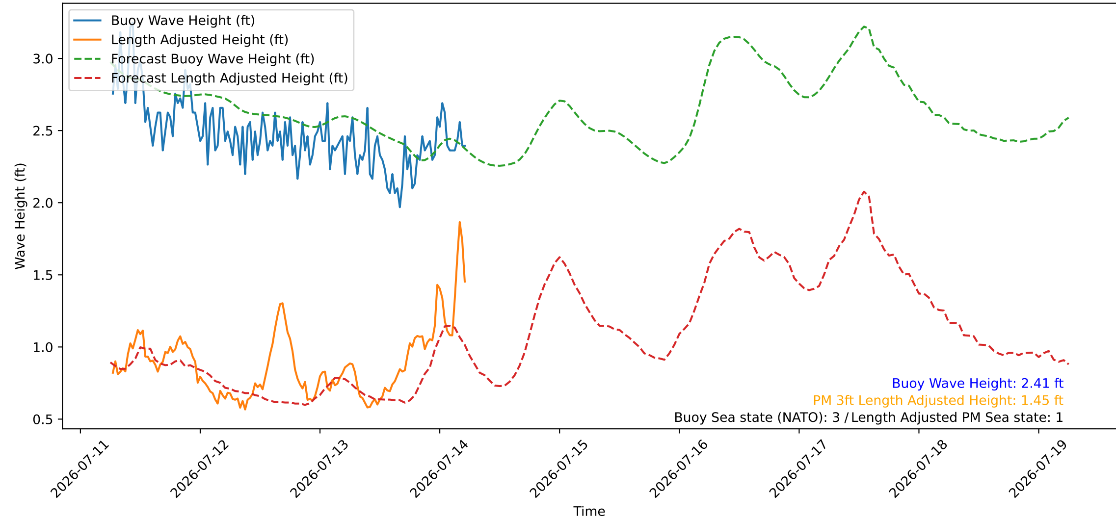
Wave Heights over Time for Red Beach at 2026-07-14 06:10:45
