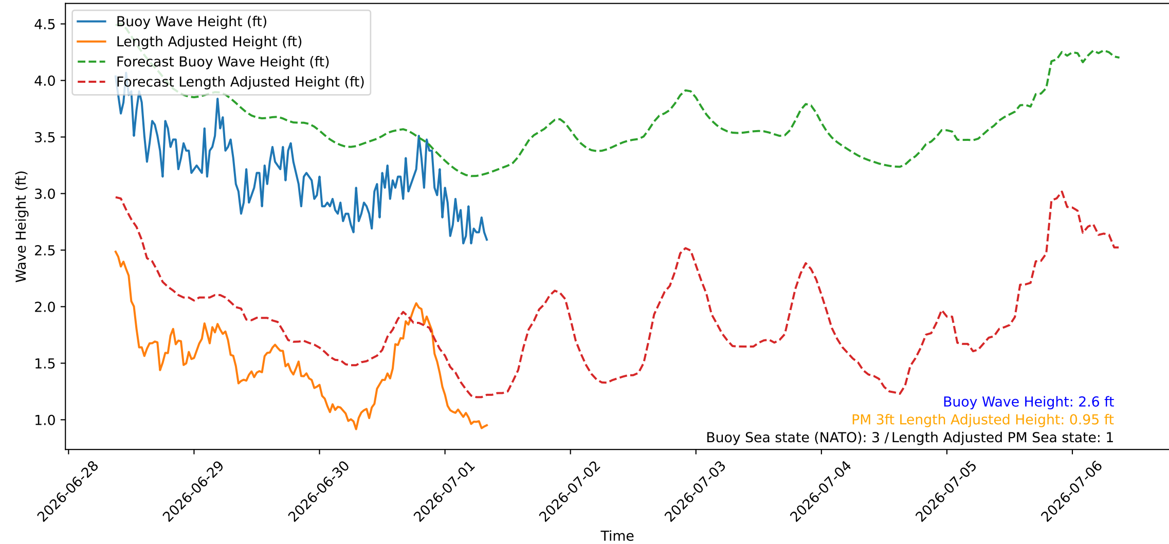
Wave Heights over Time for Green Beach at 2026-07-01 08:51:08
