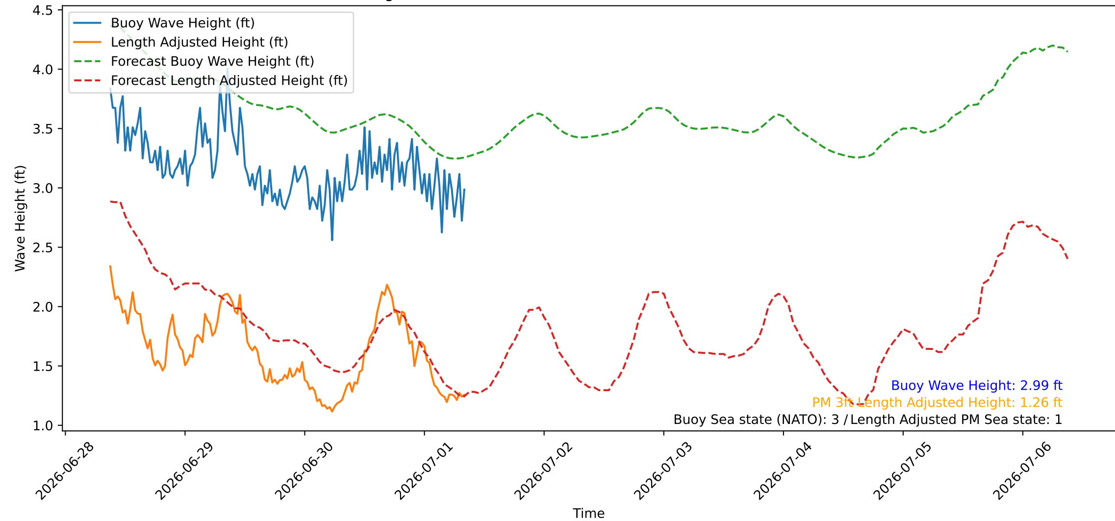
Wave Heights over Time for Oceanside Harbor at 2026-07-01 08:50:26
