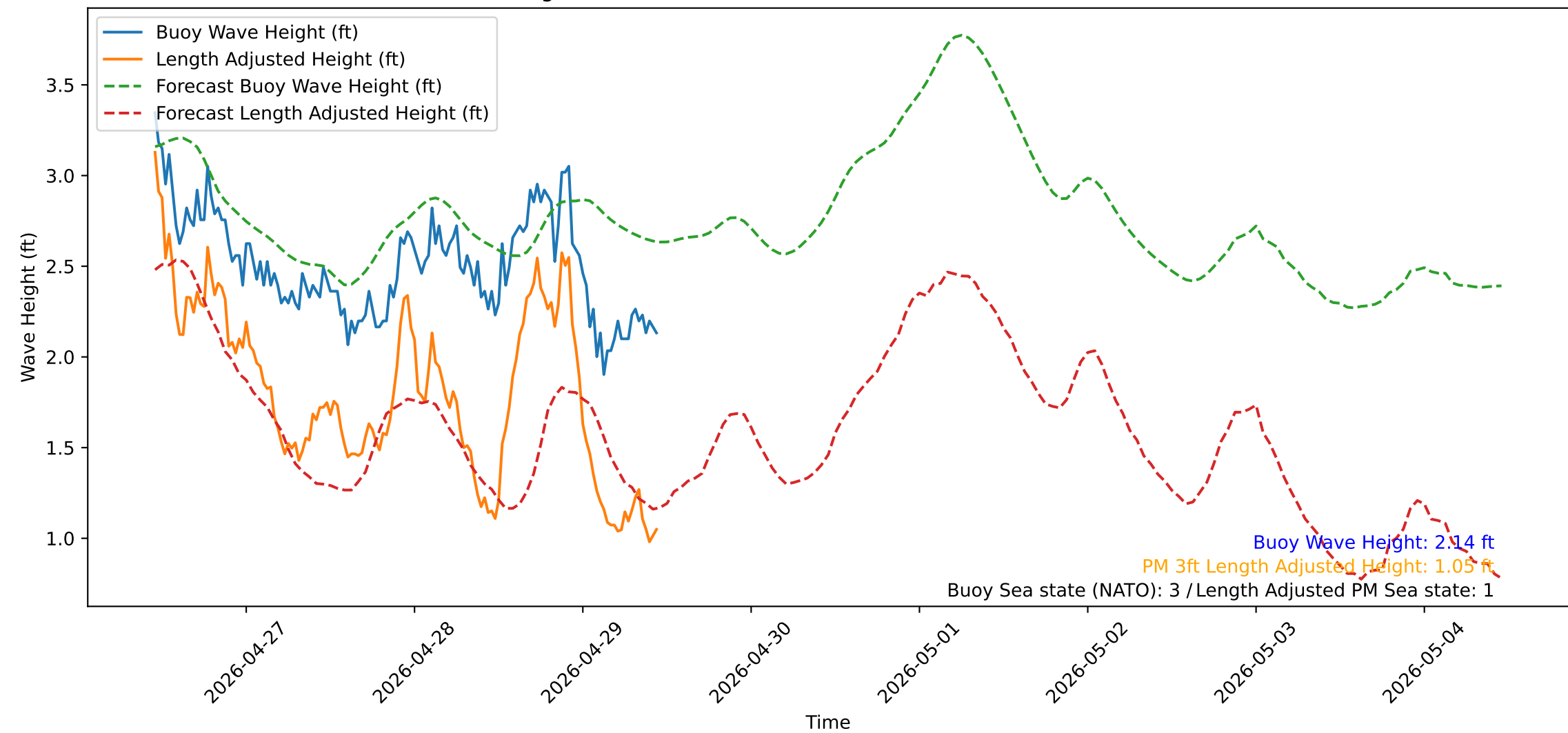
Wave Heights over Time for Oceanside Harbor at 2026-04-29 11:10:32
