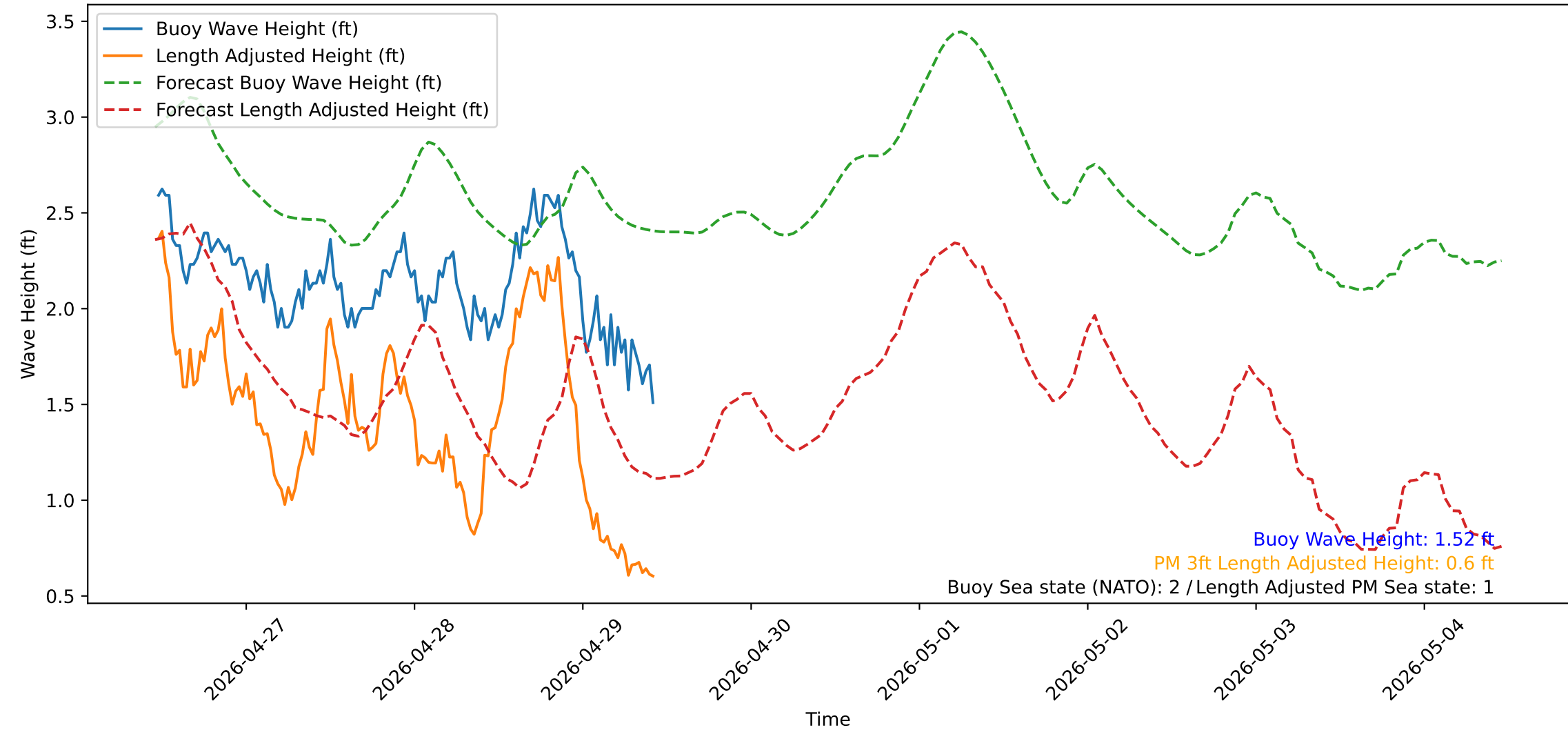
Wave Heights over Time for Red Beach at 2026-04-29 11:10:51
