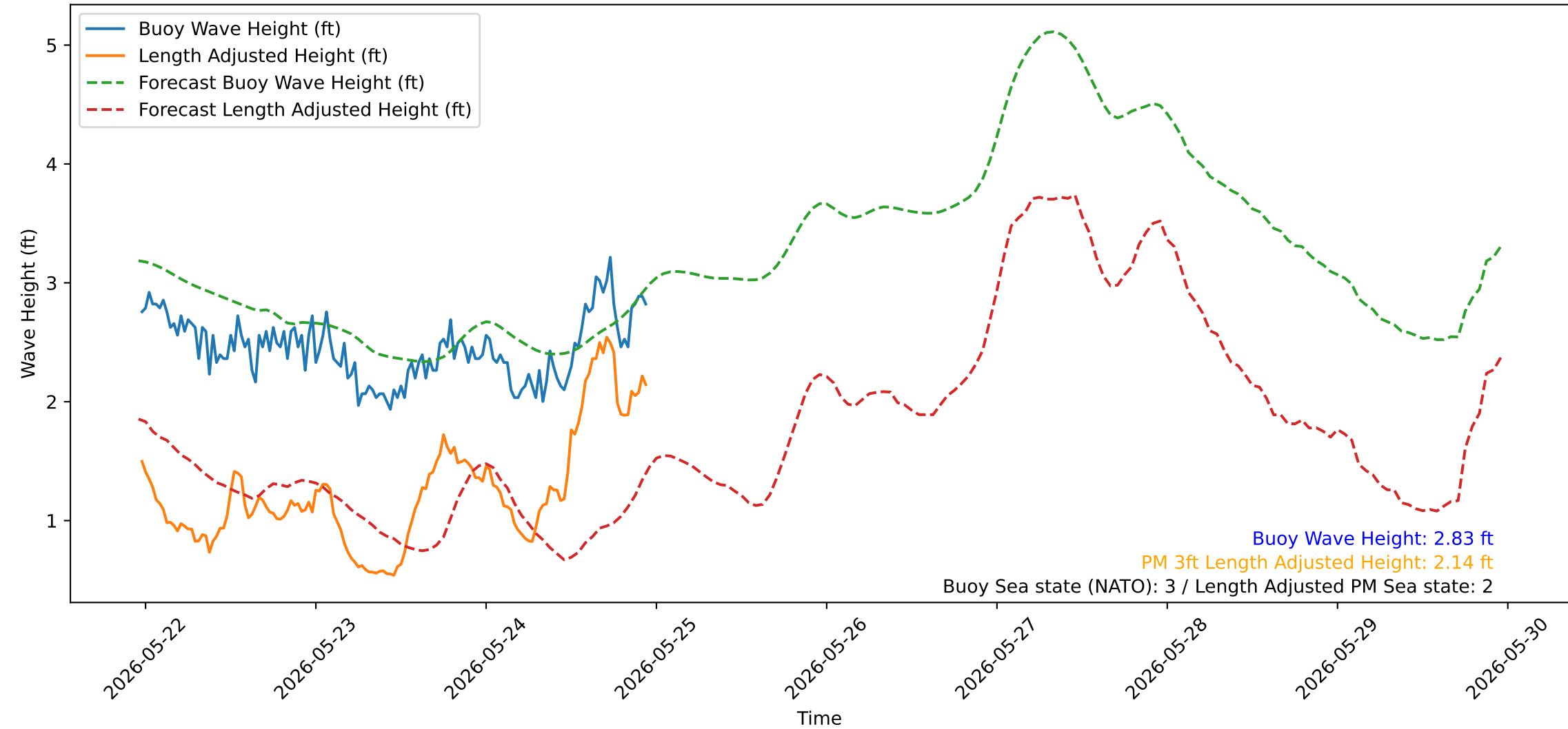
Wave Heights over Time for Red Beach at 2026-05-24 23:10:51
