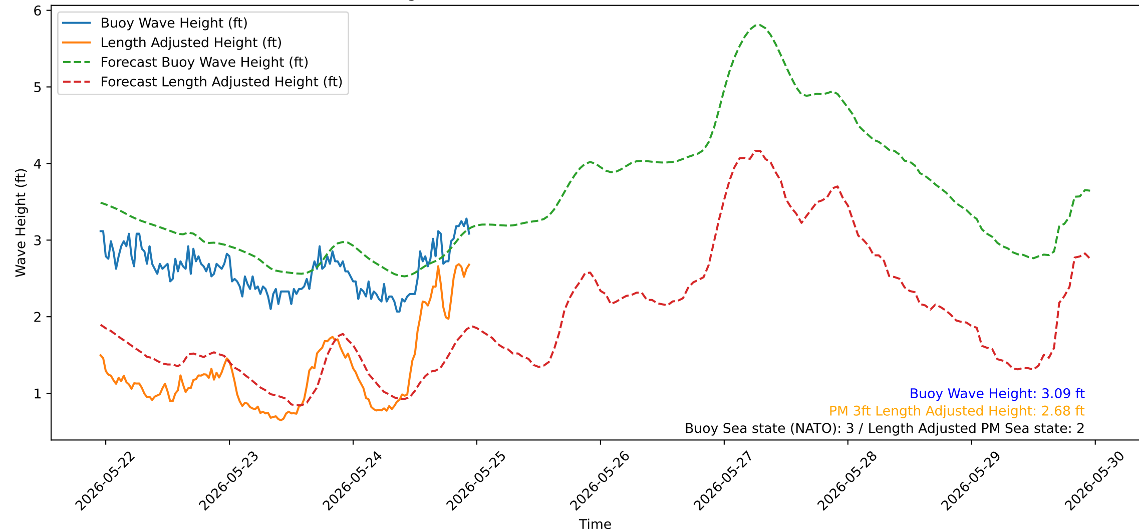
Wave Heights over Time for Green Beach at 2026-05-24 23:11:13
