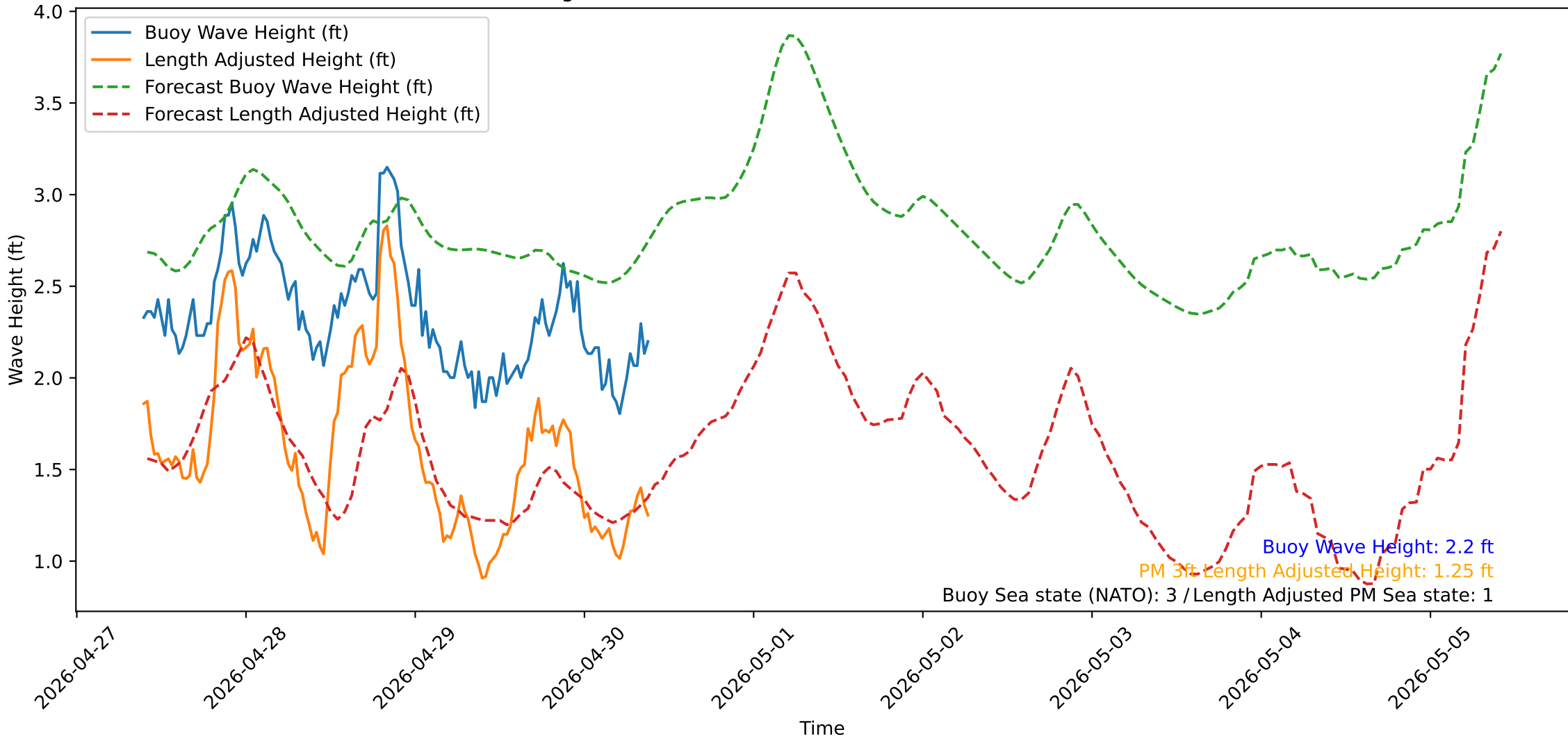
Wave Heights over Time for Green Beach at 2026-04-30 09:41:13
