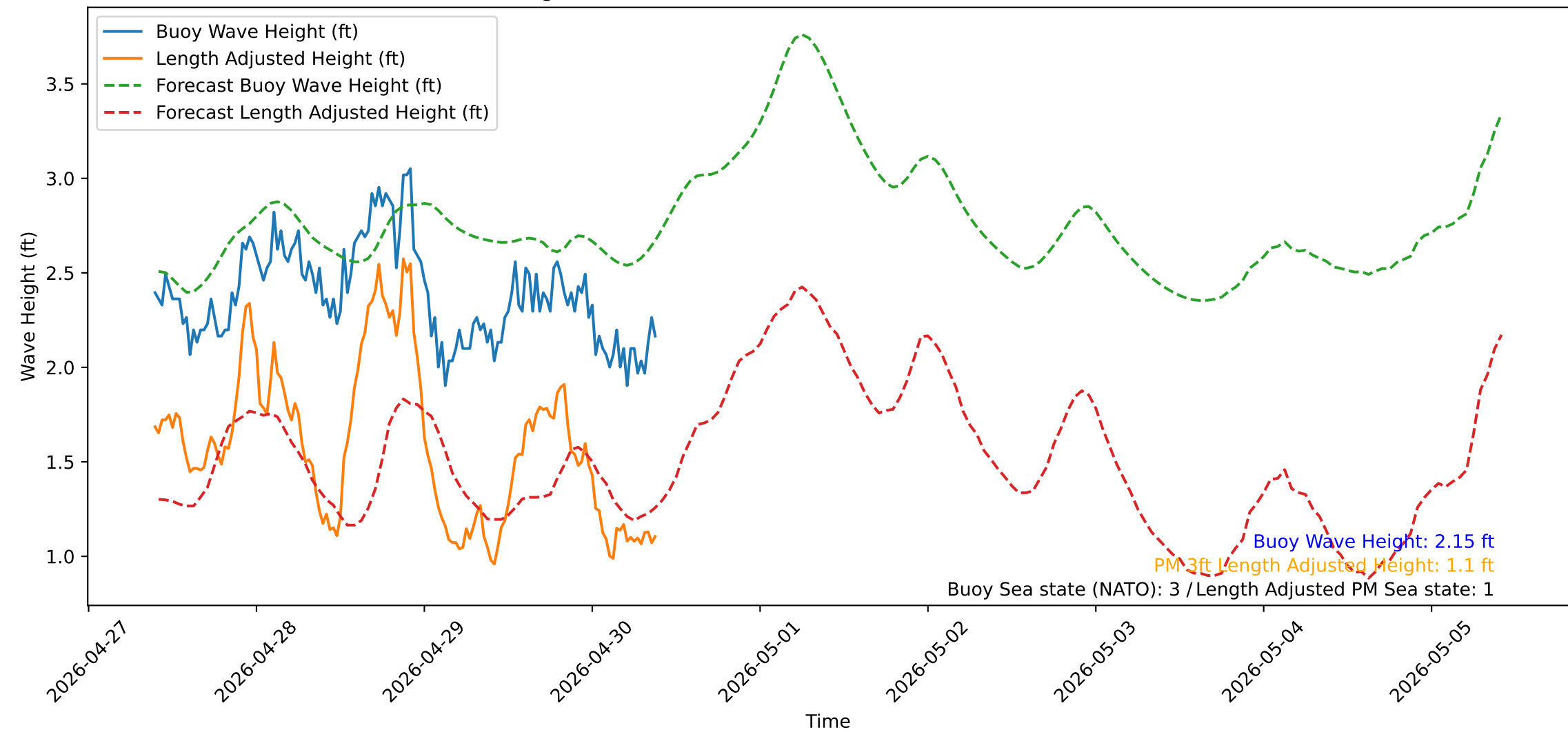
Wave Heights over Time for Oceanside Harbor at 2026-04-30 09:40:31
