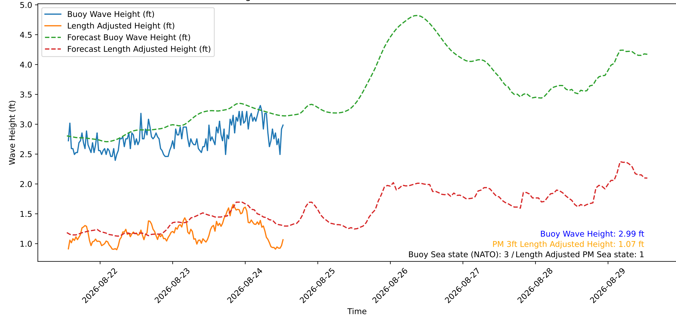
Wave Heights over Time for Green Beach at 2026-08-24 13:21:14
