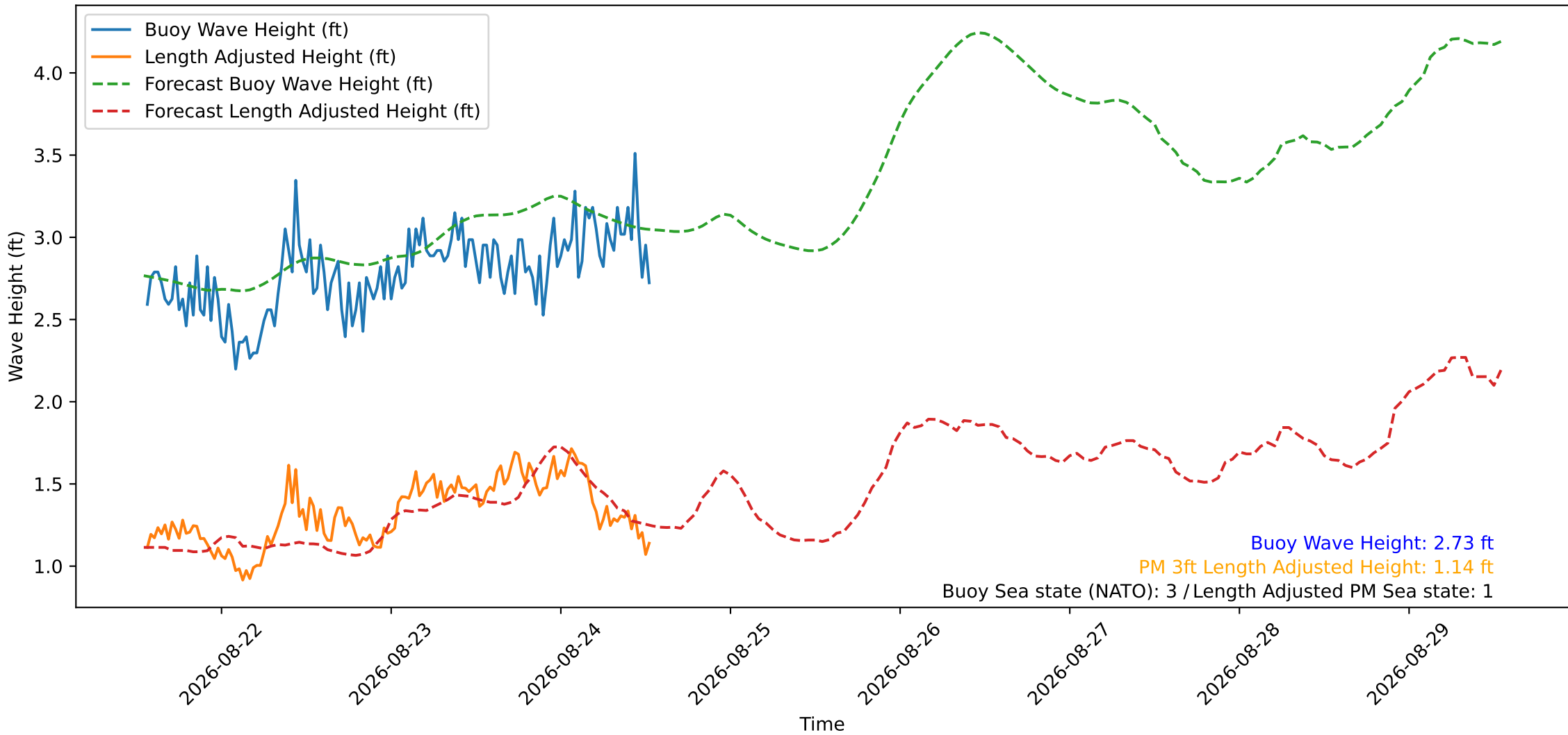
Wave Heights over Time for Oceanside Harbor at 2026-08-24 13:20:29
