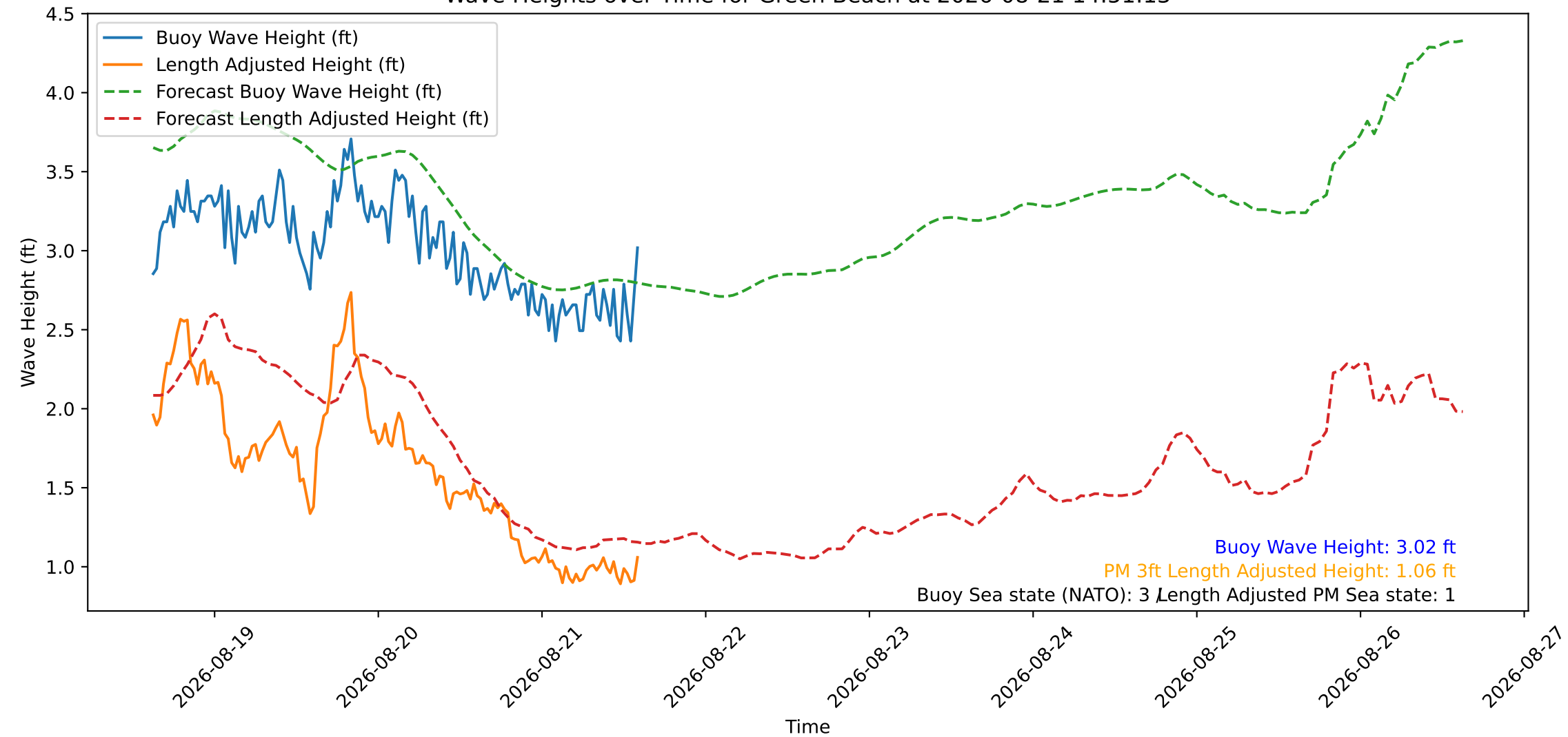
Wave Heights over Time for Green Beach at 2026-08-21 14:51:13
