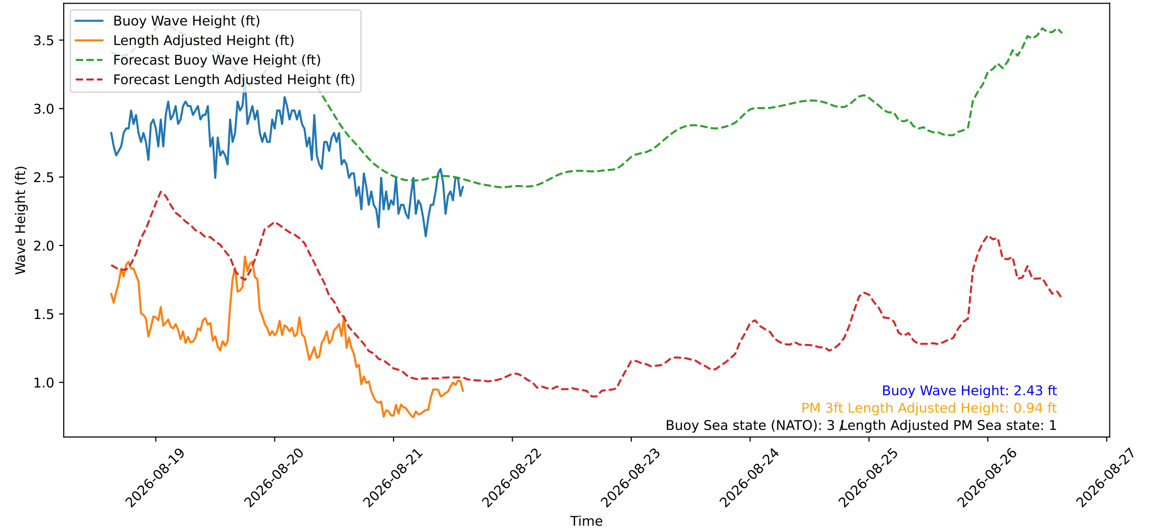
Wave Heights over Time for Red Beach at 2026-08-21 14:50:48
