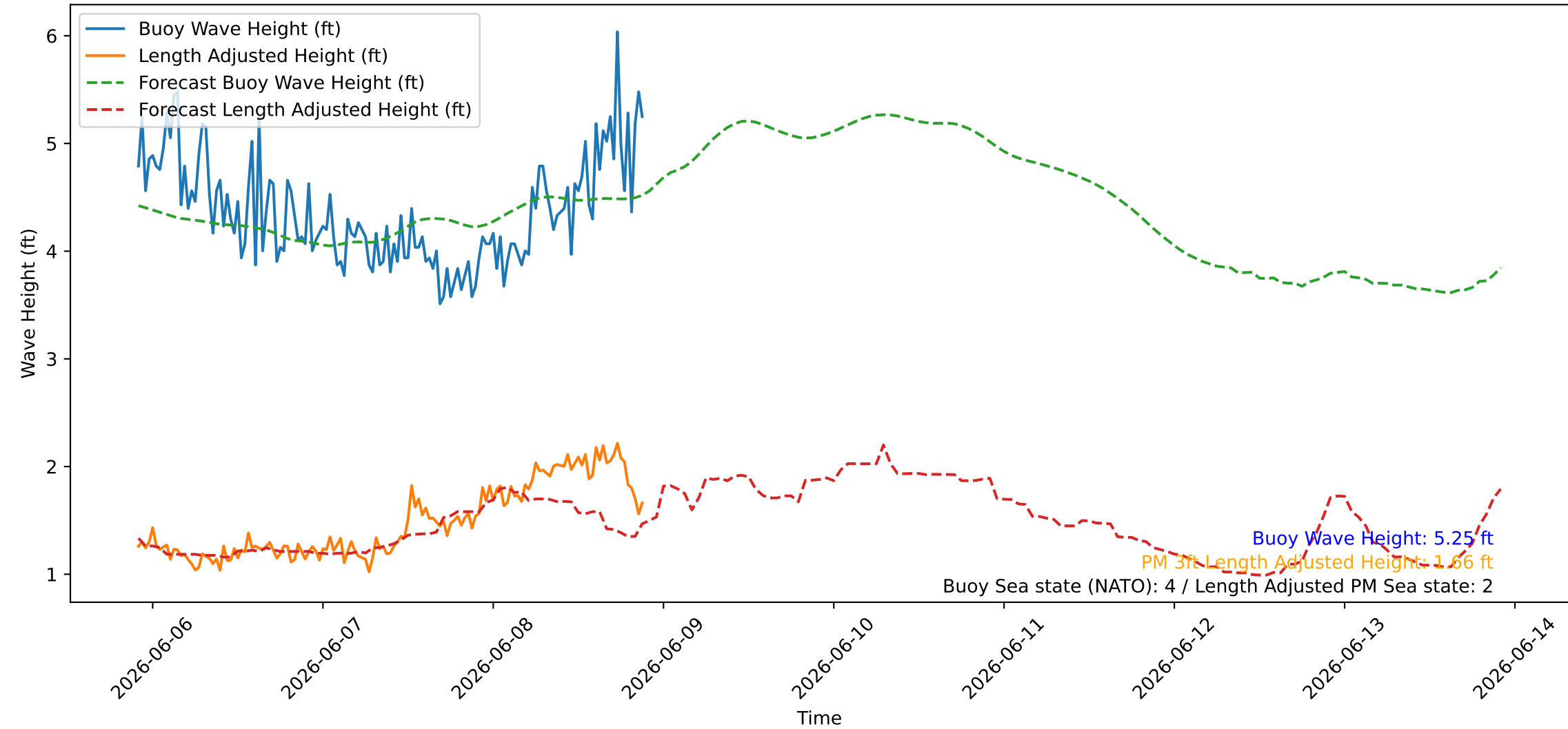
Wave Heights over Time for Oceanside Harbor at 2026-06-08 21:50:25
