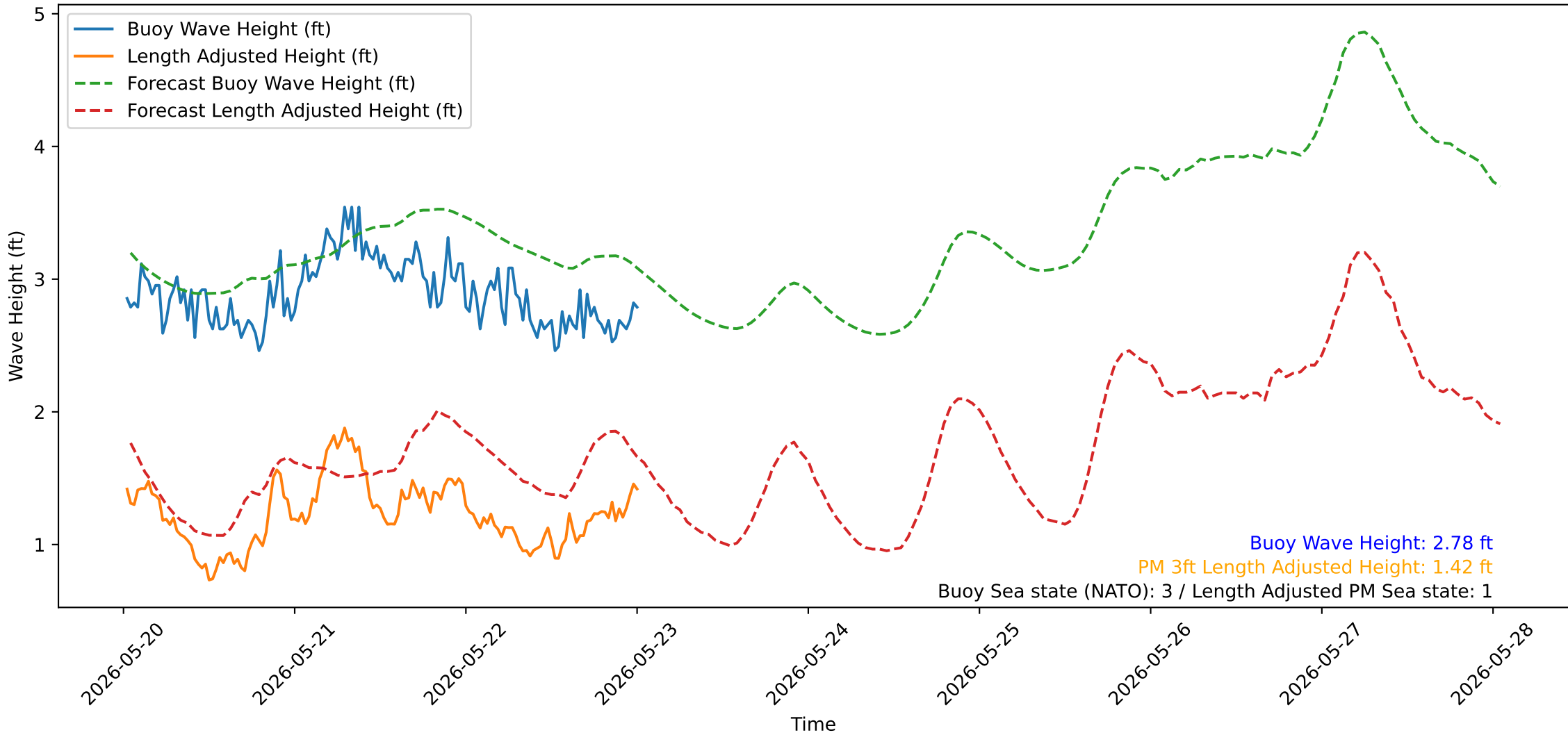
Wave Heights over Time for Green Beach at 2026-05-23 00:41:15
