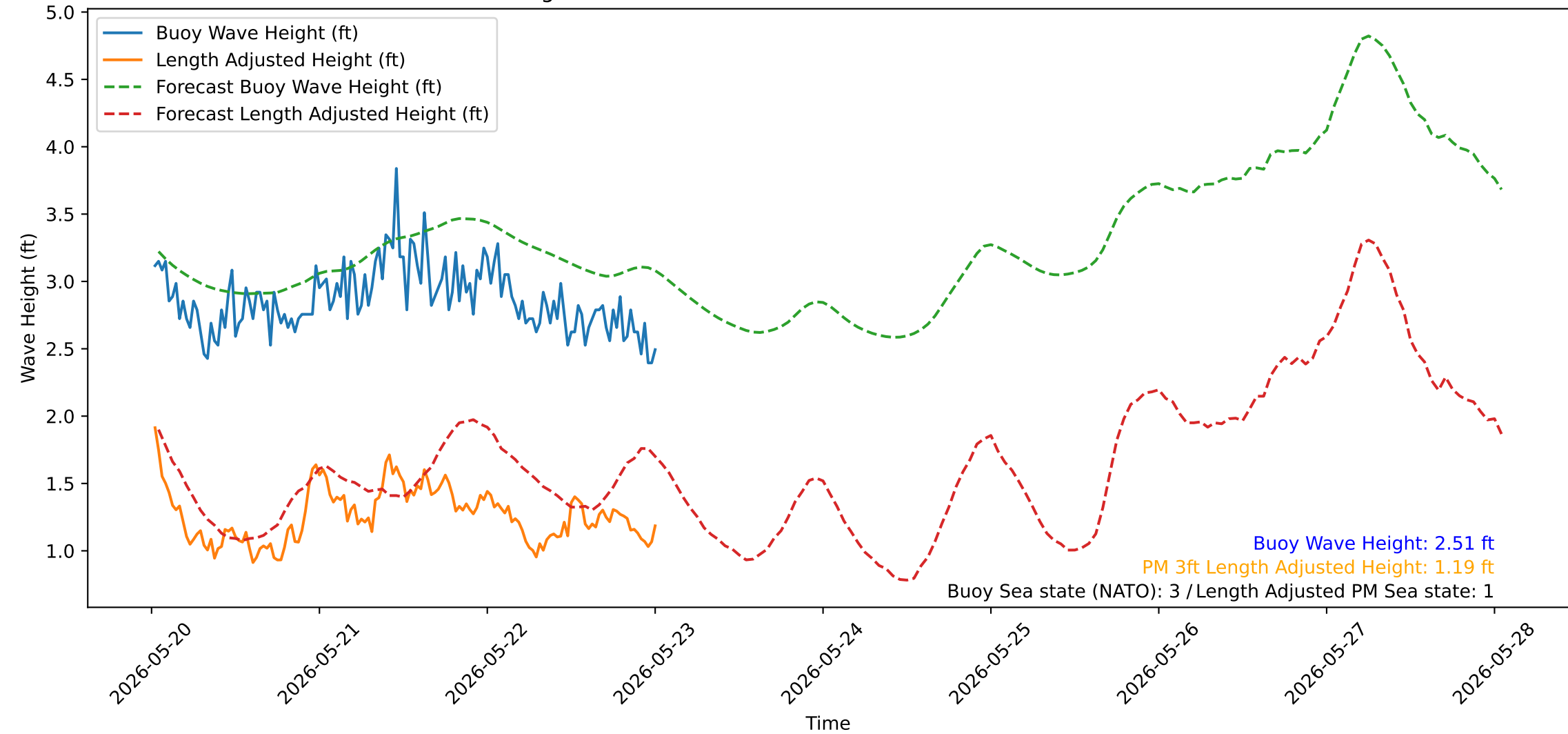
Wave Heights over Time for Oceanside Harbor at 2026-05-23 00:40:32
