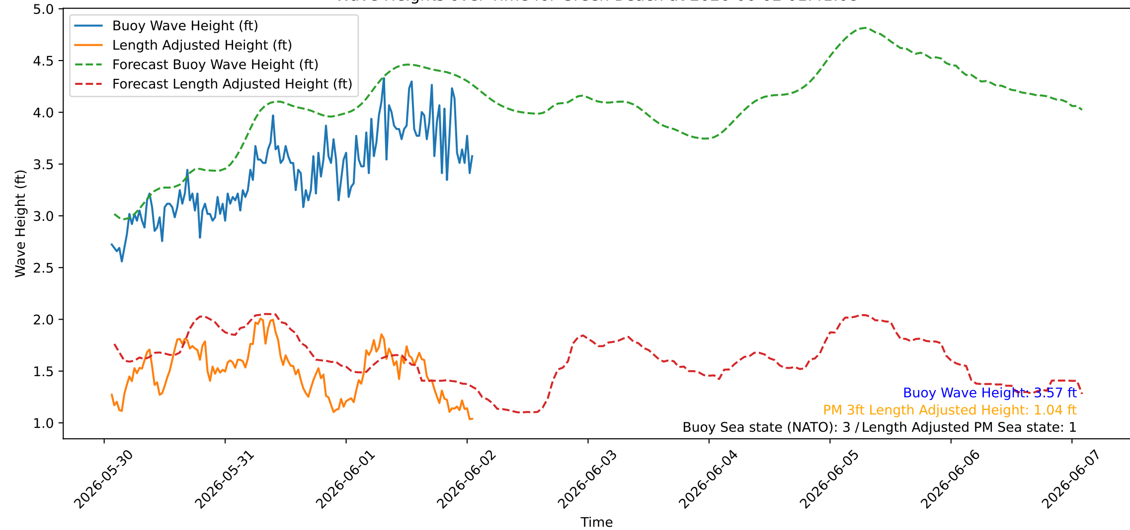
Wave Heights over Time for Green Beach at 2026-06-02 01:41:08
