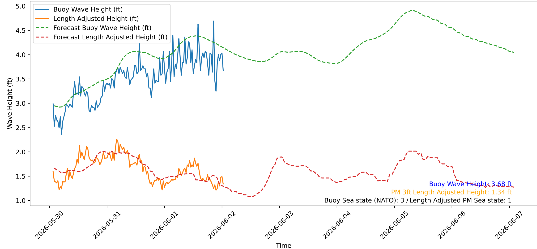
Wave Heights over Time for Oceanside Harbor at 2026-06-02 01:40:26
