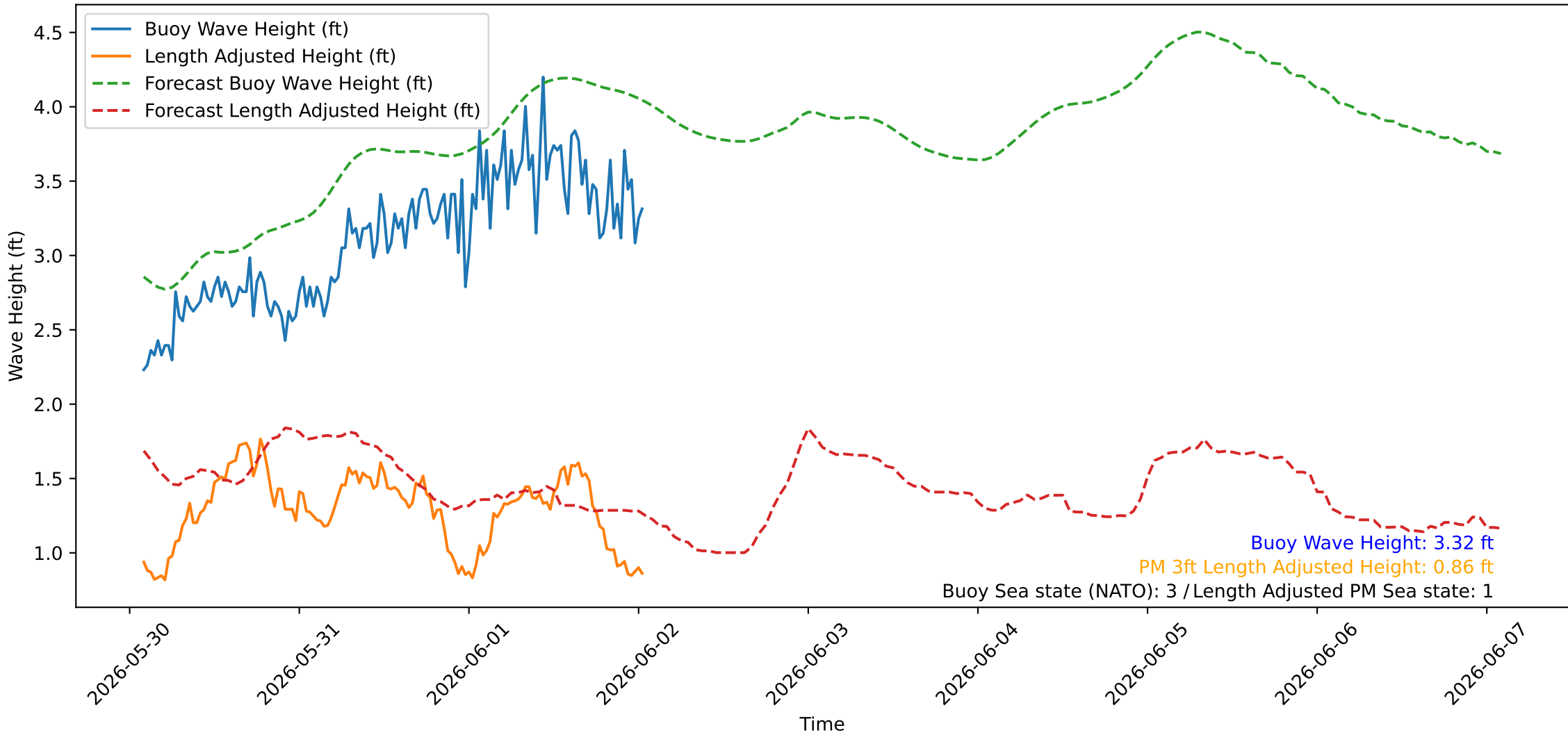
Wave Heights over Time for Red Beach at 2026-06-02 01:40:46
