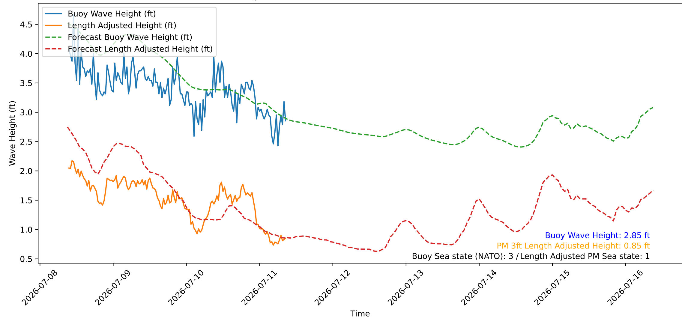
Wave Heights over Time for Red Beach at 2026-07-11 09:10:46
