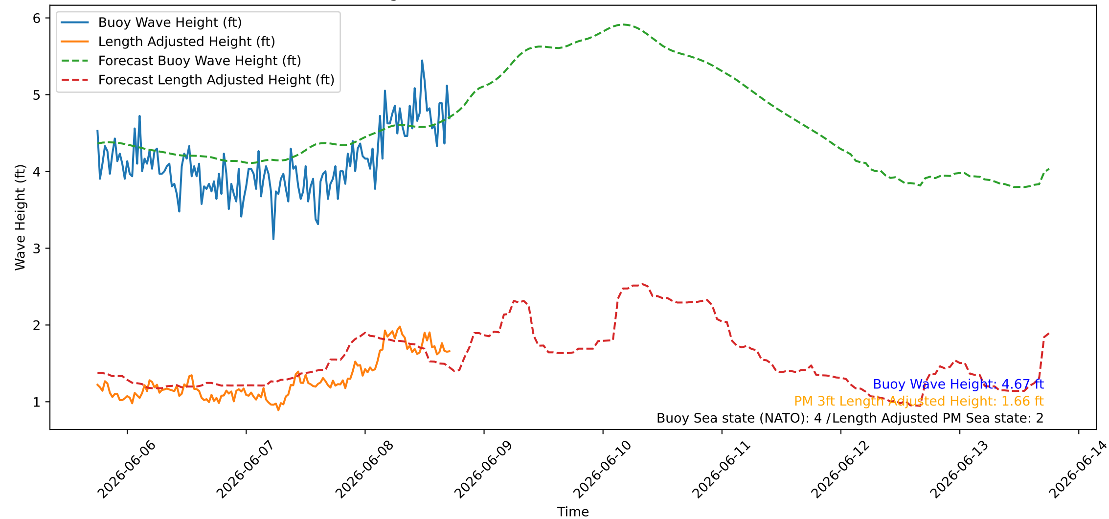
Wave Heights over Time for Green Beach at 2026-06-08 17:51:09
