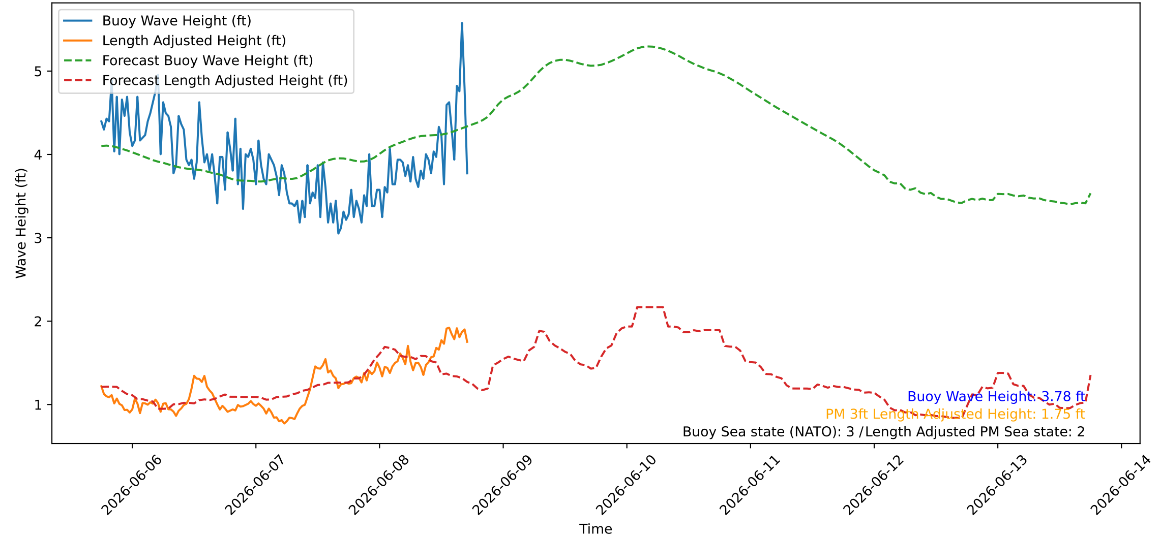
Wave Heights over Time for Red Beach at 2026-06-08 17:50:47
